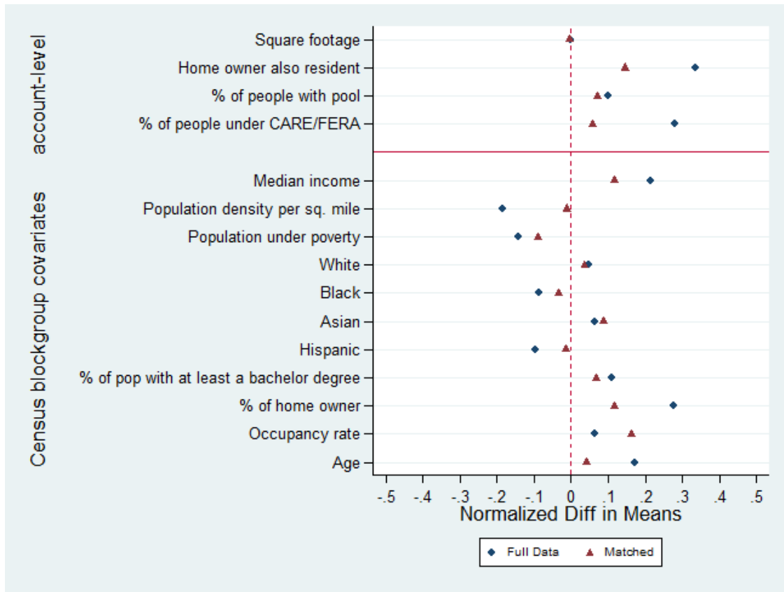
Figure A2: Changes in Normalized Differences after Matching
