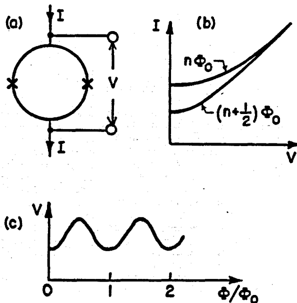
Figure 2 (a) dc SQUID, with resistivity shunted junctions; (b) I-V characteristics with fluxes n\Phi_0 and (n + 1/2)\Phi_0 threading SQUID; (c) V vs. \Phi .
