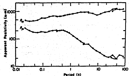
Figure 7. Apparent resistivities obtained from one set of data at Upper La Gloria, using remote reference method.
