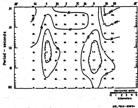
Figure 17 Calculated TE mode apparent resistivity pseudo-section (line A-A') for the revised two-dimensional model shown in Figure 16.
