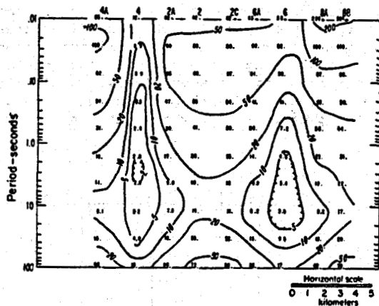
Figure 14. Calculated TE mode apparent resistivity pseudo-section (line A-A') for model shown in Figure 12.
