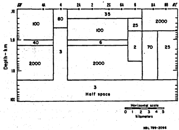
Figure 16 Revised two-dimensional model fit to the MT stations along line A-A' after inter-changing modes at stations 4, 8A, and 8B.
