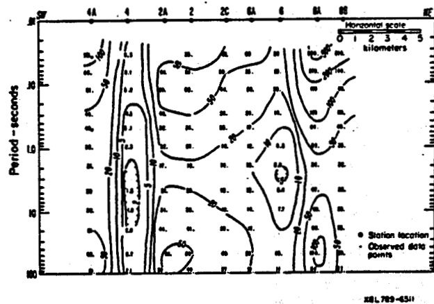
Figure 13 Measured TE mode apparent resistivity pseudo-section for line A-A', Swan Lake Valley, Klamath County, Oregon.
