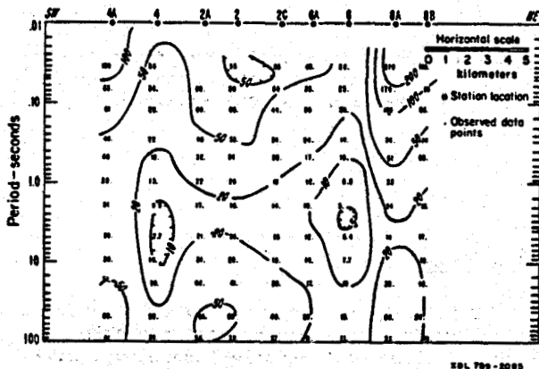
Figure 15 Measured TE mode apparent resistivity pseudo-section (line A-A') after presumed TE and TM apparent resistivities were interchanged at stations 4, 8A, and 8B.
