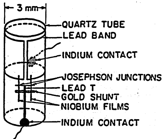
Figure 3 Practical dc SQUID.
