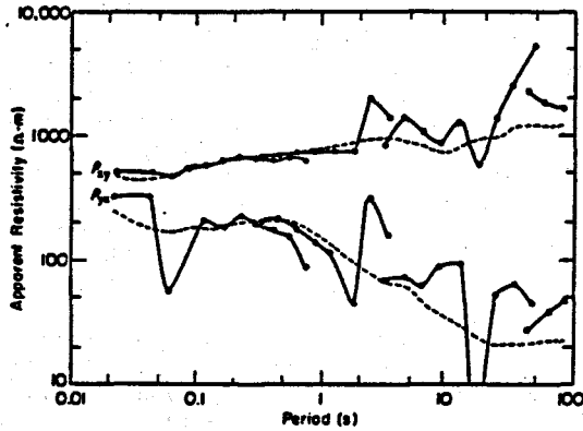
Figure 8 Apparent resistivities obtained from the same set of data as in Fig. 7, using conventional analysis scheme (solid line). Dashed lines represent curves in Fig. 7.
