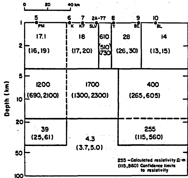
Figure 19 Two-dimensional model fitted to the regional MT survey between the Parker (PM) and Bly (BL) stations.
