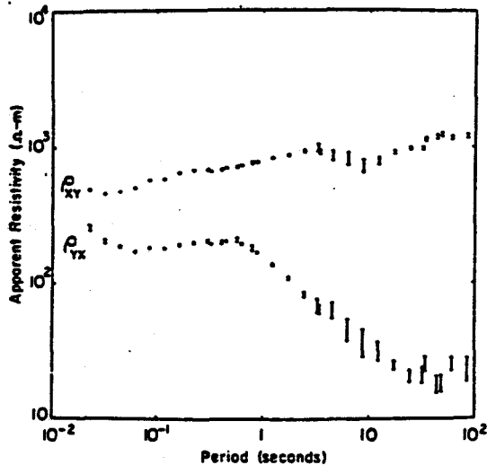
Figure 9 Apparent resistivities shown in Figure 7 replotted with vertical bars representing the probable errors.
