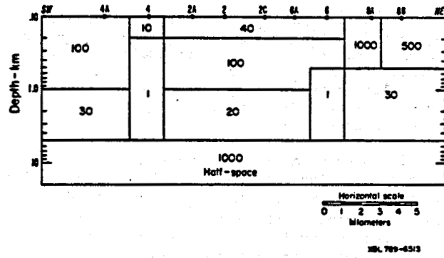
Figure 12 Initial two-dimensional model fit to the line of MT stations along line A-A', Swan Lake Valley area, Klamath County, Oregon.
