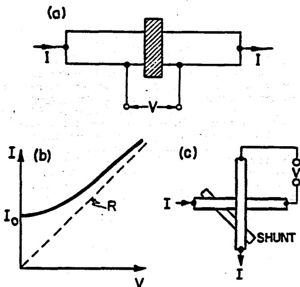
Figure 1 (a) Two superconductors separated by insulating barrier to form a Josephson tunnel junction; (b) current (I) vs. voltage (V) characteristic for a Josephson junction shunted with a resistance, as shown in (c).
