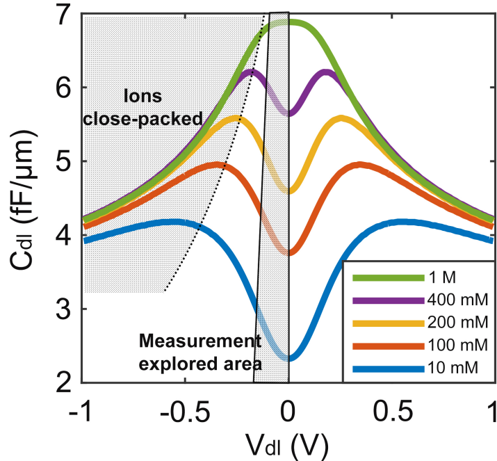
Figure 3.10: Double layer capacitance of a SWNT as a function of surface potential and ionic concentration. Ions are close-packed near the SWNT when either the surface potential or the ionic concentration is high (top left grey area). The measurement here only covers the double layer capacitance in a low potential range (middle grey area), due to the domination of quantum capacitance.
