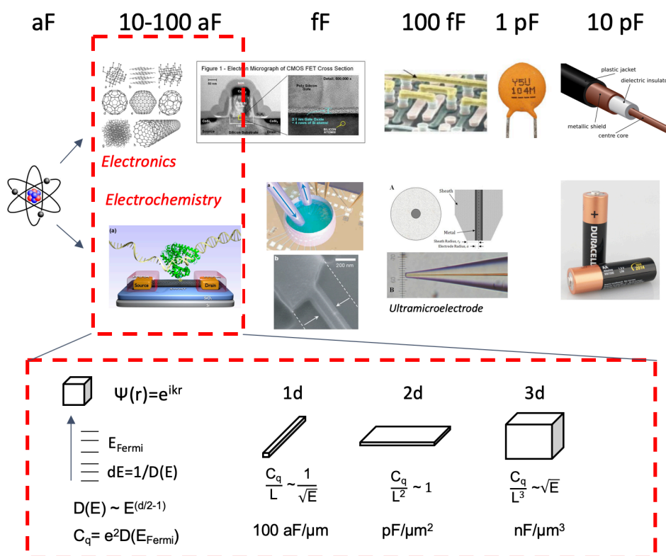
Figure 4.2: Typical capacitance values for various conditions, from atomic to macroscopic. Top: Dry environment (Ref. 66-68 ). Middle row: liquid environment (Ref. 69-71 ). The inset indicated schematically the density of states for materials whose dimension approach the de Broglie wavelength of the electrons, adding an additional quantum capacitance which is not significant in the larger macroscopic electrode.
