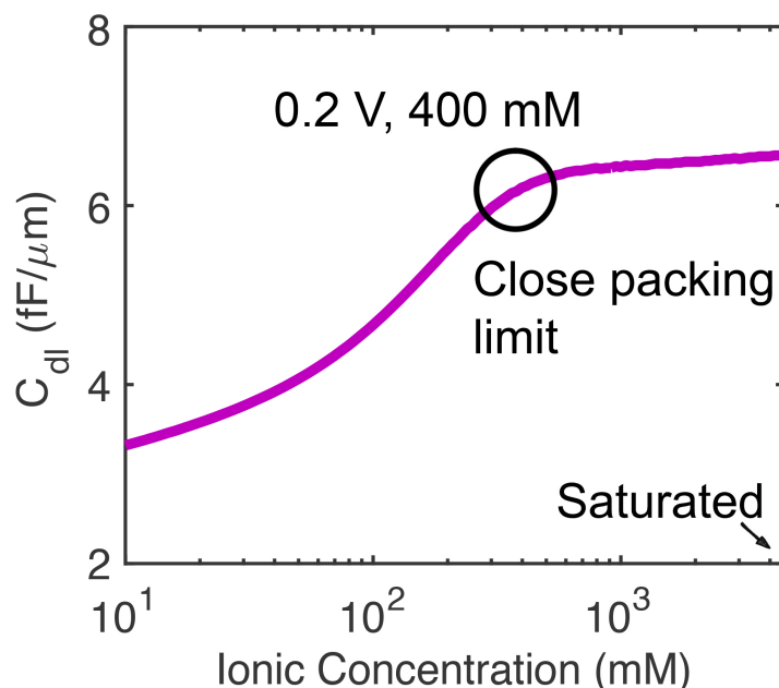
Figure 3.11: Double layer capacitance as a function of ionic concentration. The capacitance reaches close-packing limit at ionic concentration \sim 400 mM and surface potential 0.2 V.
