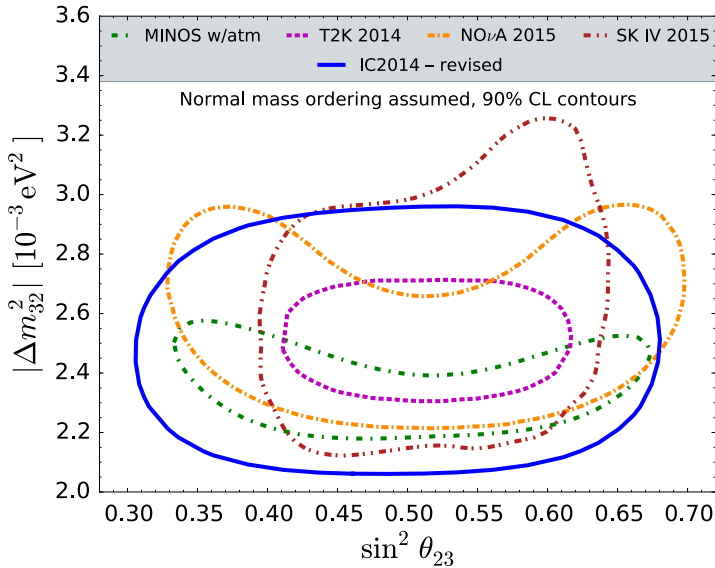
Figure 4: Current measurements of the atmospheric mixing between the second and third mass eigenstates from atmospheric and long-baseline neutrino experiments. Note that only the magnitude of the mass-squared splitting is known, not its sign.
