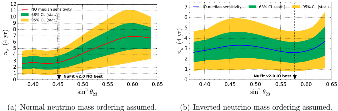
Figure 8: Expected significance with which the neutrino mass ordering will be determined using four years of data, as a function of the true value of \sin^2(\theta_{23}) . Solid red (NO) and blue (IO) lines show median significances, while the green and yellow bands indicate the range of significances obtained in 68% and 95% of hypothetical experiments. The significance for determining the ordering when the true ordering is inverted is relatively insensitive to \theta_{23} , while for the normal ordering large values of \theta_{23} are advantageous. The range shown corresponds approximately to the current 3\sigma allowed region of \theta_{23} ; the global best-fit values from the NuFit group [23] for both orderings are indicated by black arrows.
