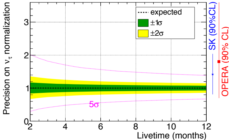
Figure 9: Precision with which the rate of \nu_\tau appearance can be measured, in terms of the PMNS expected rate, as a function of exposure (in months). The true value is assumed to be 1.0 (the standard expectation) for illustration. The expected \pm 1\sigma and \pm 2\sigma regions and \pm 5\sigma limits are shown, as well as current measurements by Super-K [14] and OPERA [52].
