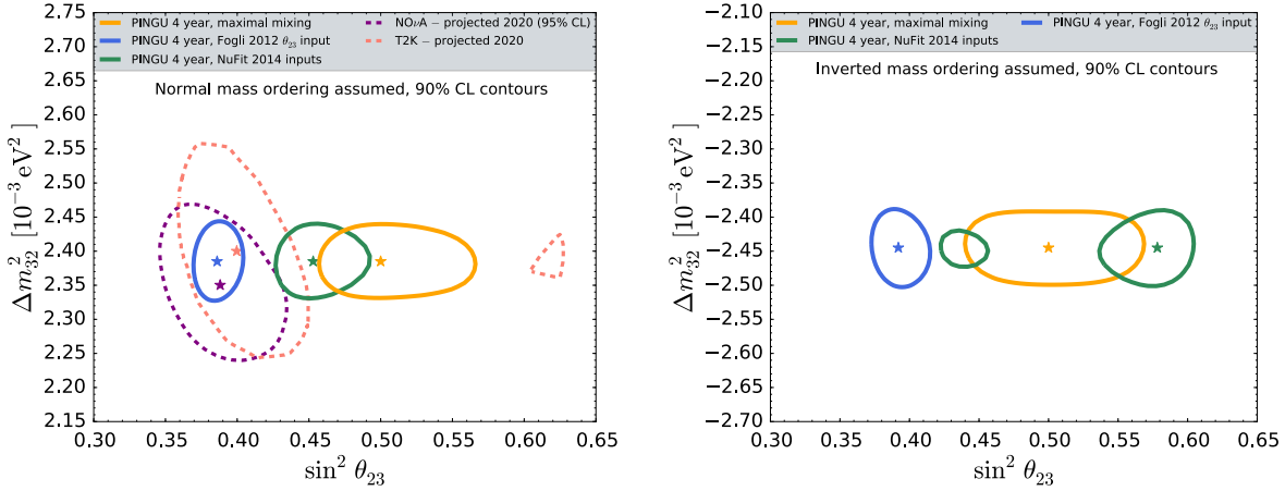
(a) Normal neutrino mass ordering assumed. (b) Inverted neutrino mass ordering assumed.
