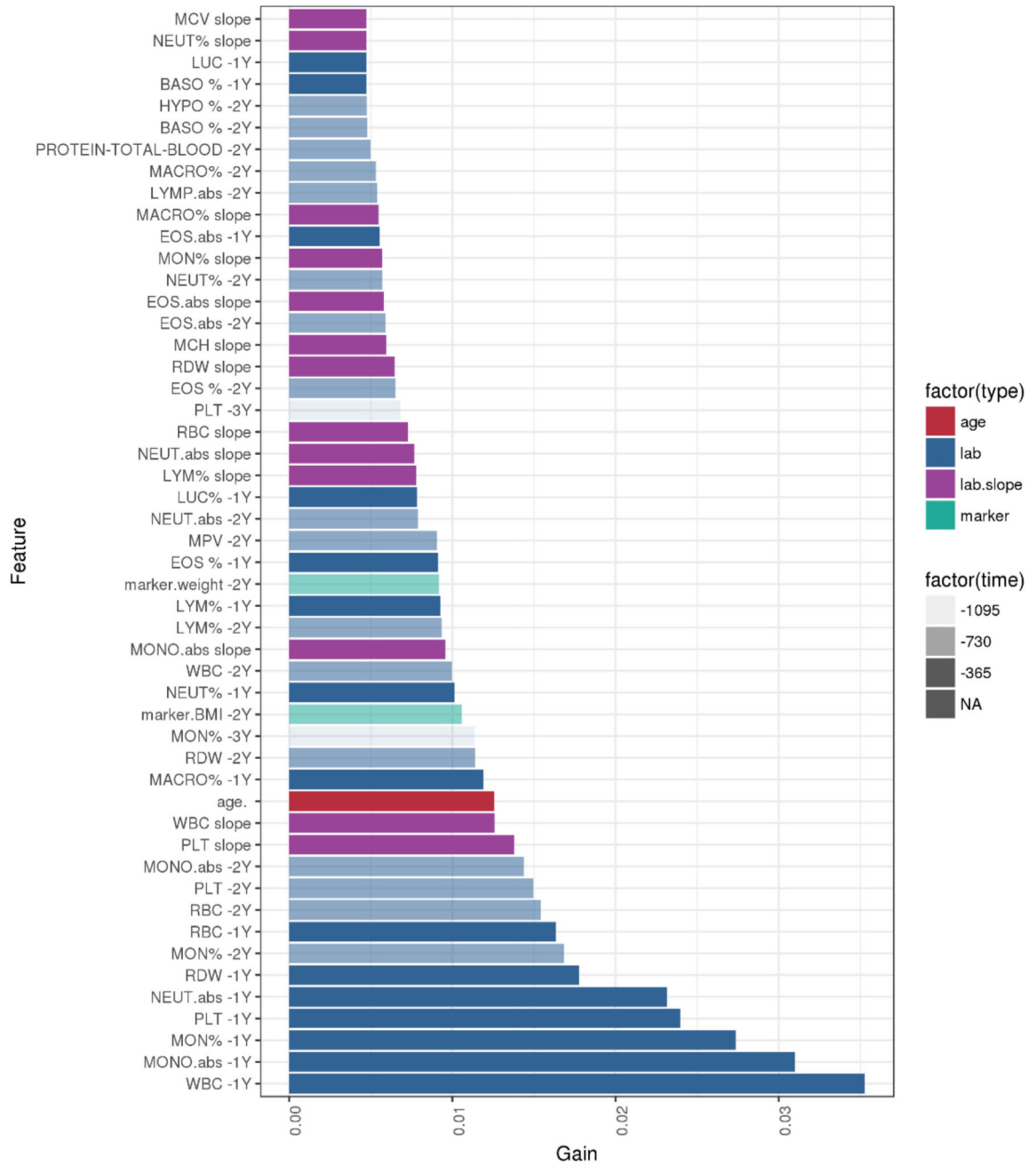
Extended Data Figure 8. Top 50 EHR model parameters
