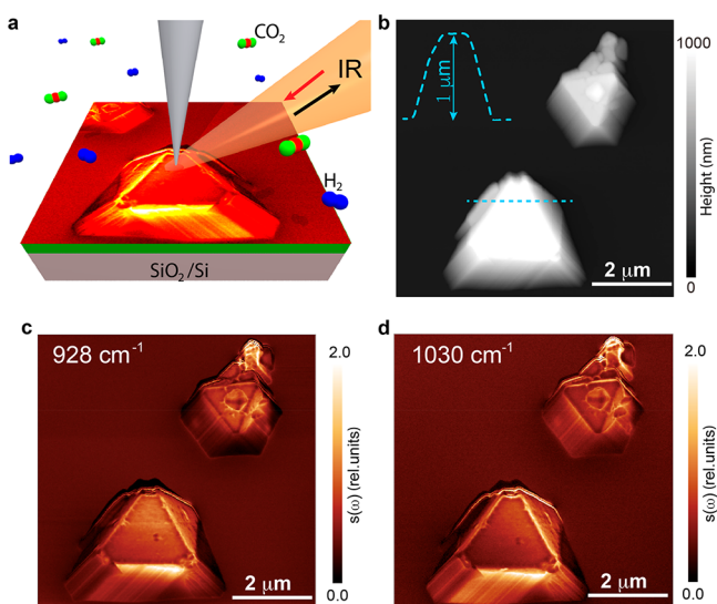
Figure 1. Topographic and nano-IR imaging of \text{Cu}_2\text{O} microcrystals. (a) Schematic of the IR nanoimaging experiment, showing the metallic nanoprobe tip illuminated by an IR laser beam. \text{Cu}_2\text{O} microcrystals were exposed to \text{CO}_2 (white and red) and released \text{H}_2 (blue). (b) Atomic force microscope topography image of \text{Cu}_2\text{O} crystals. Inset shows the experimental line profile across one of the \text{Cu}_2\text{O} crystals. (c and d) Nano-IR amplitude s(\omega) images of \text{Cu}_2\text{O} at two different IR frequencies.
