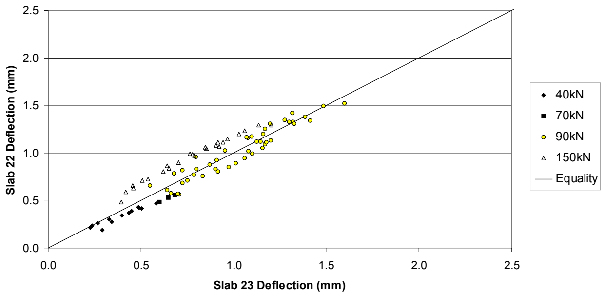
Comparison of deflections on either side of Joint 22 Slab 23/Slab 22 (JDMD 4 and JDMD 5)
