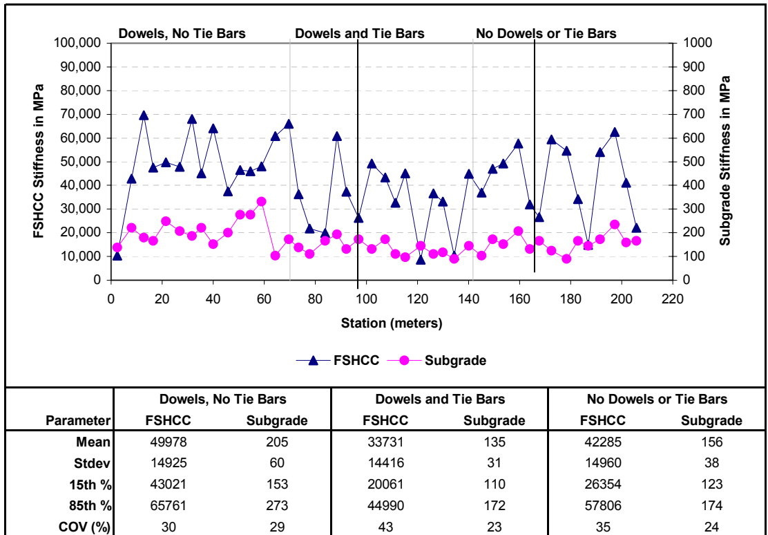
Figure 169. Back-calculated stiffness 90 days after concrete construction.
