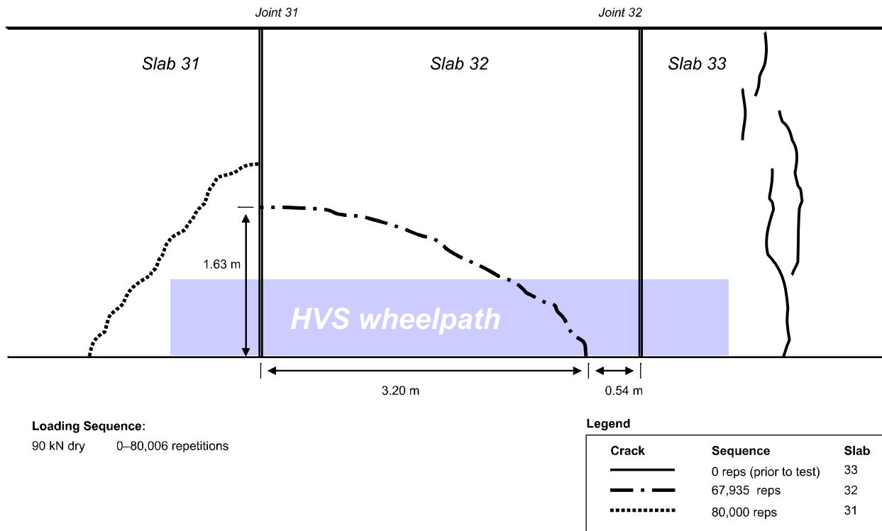
Figure 31. Schematic of crack pattern, Test 535FD.
