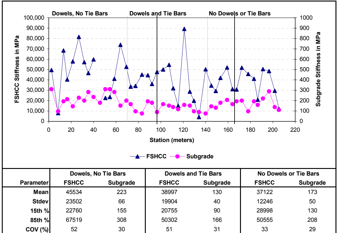
Figure 168. Back-calculated stiffness 49 days after concrete construction.
