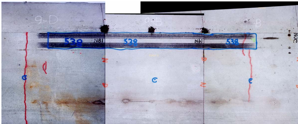
Figure 72. Composite image of Test 538FD showing cracks.
