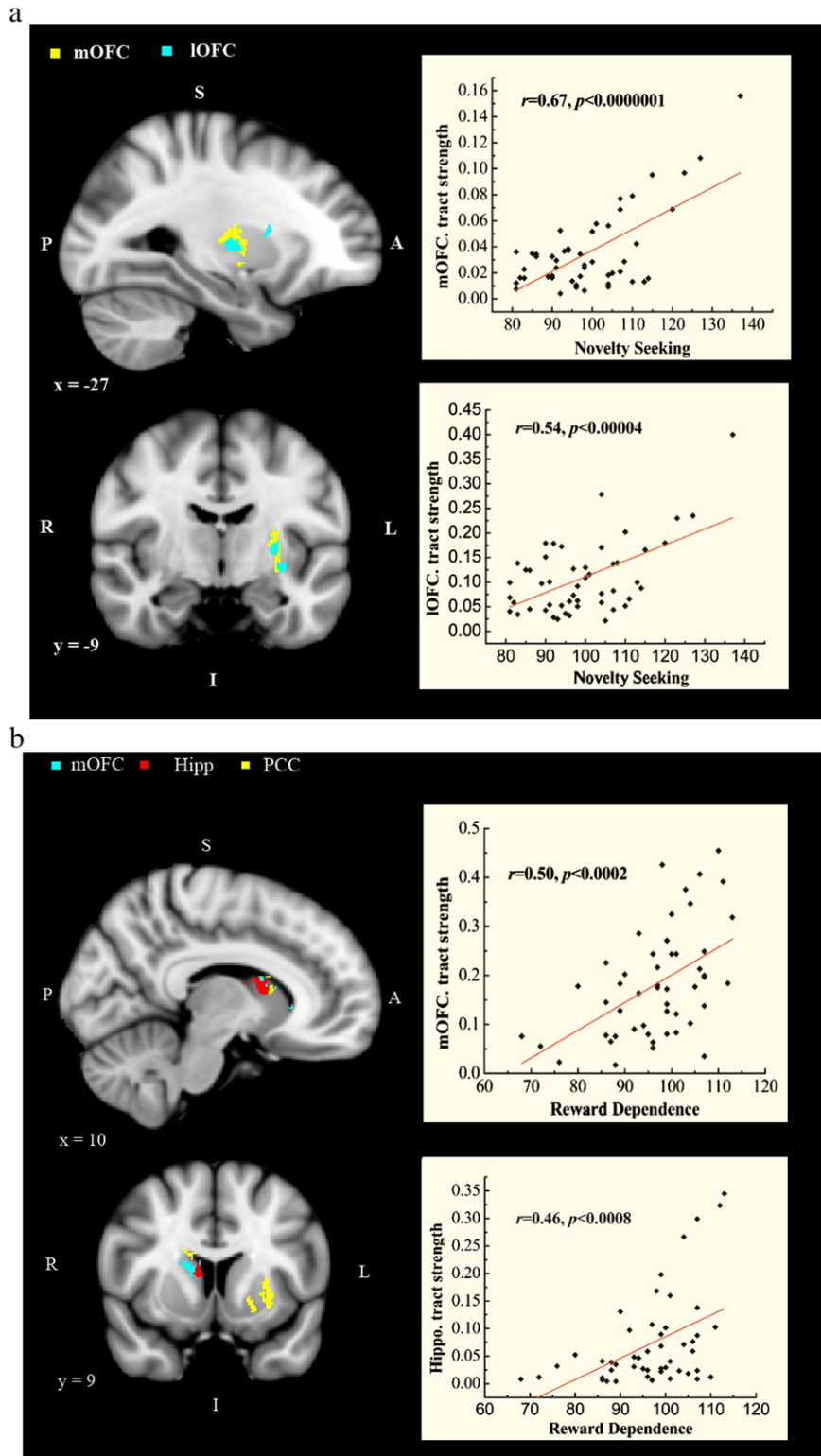
Fig. 1. Fiber connectivity from different brain regions to the striatum were correlated with different temperaments. (a) Fiber connectivity from the mOFC and IOFC to the striatum was correlated with NS. (b) Fiber connectivity from the PCC, mOFC, and hippocampus to the striatum was correlated with RD. (c) Fiber connectivity from the dlPFC and PCC to the striatum was correlated with HA. (d) Fiber connectivity from the mOFC into the striatum was correlated with P.
