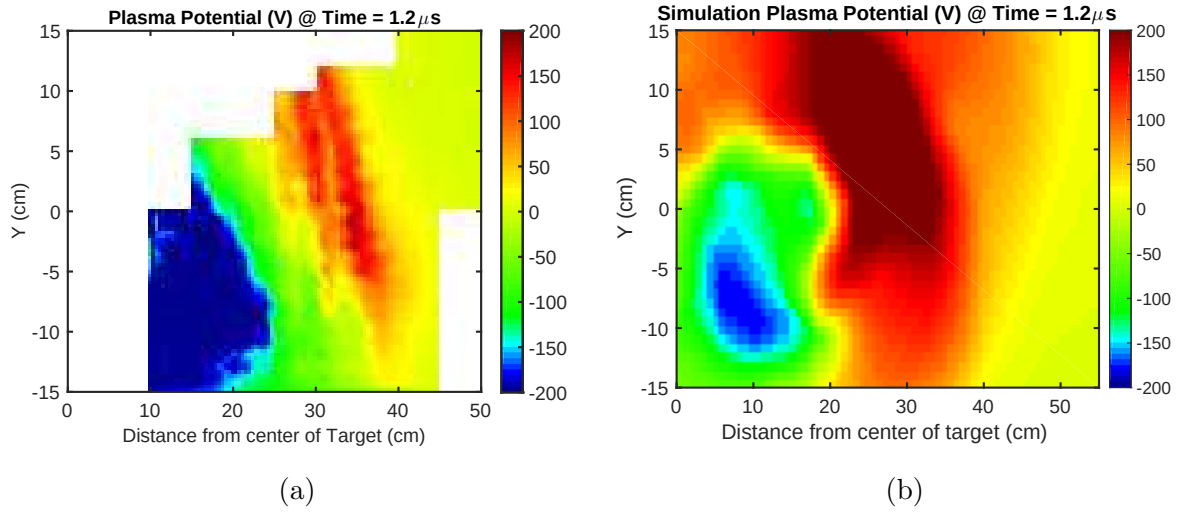
Figure 5.12: Shows (a) measured experimental \phi in an X-Y oriented plane at t = 1.2 \mu s and (b) the corresponding output from fHybrid3D.
