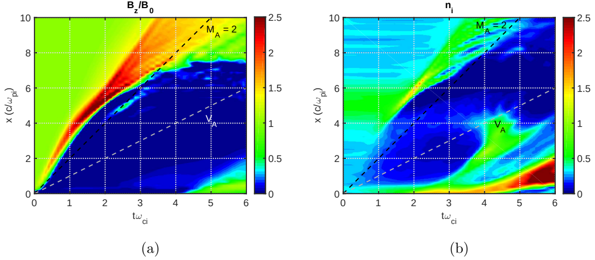
Figure 4.5: Output from fHybrid3D along the blow-off axis for (a) B_z and (b) n_i .
