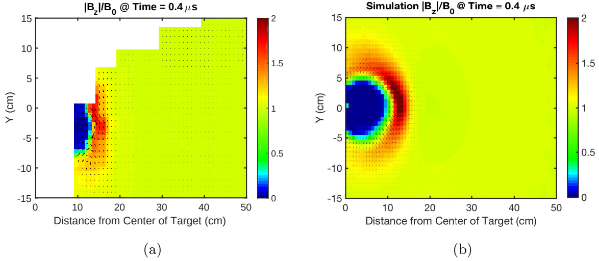
Figure 5.2: Shows (a) measured experimental B_z in an X-Y oriented plane at t = 0.4\mu s , with arrows over-plotted to show direction and magnitude of transverse B field, and (b) the corresponding output from fHybrid3D.
