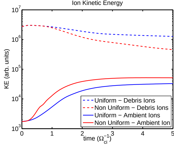
Figure 3.9: Kinetic energy of ambient ions (solid) and debris ions (dashed) for the uniform (blue/outer) versus the nonuniform (red/inner) simulation calculated from a sampling of particle data, which shows improved energy coupling to the ambient ions in the nonuniform case.
