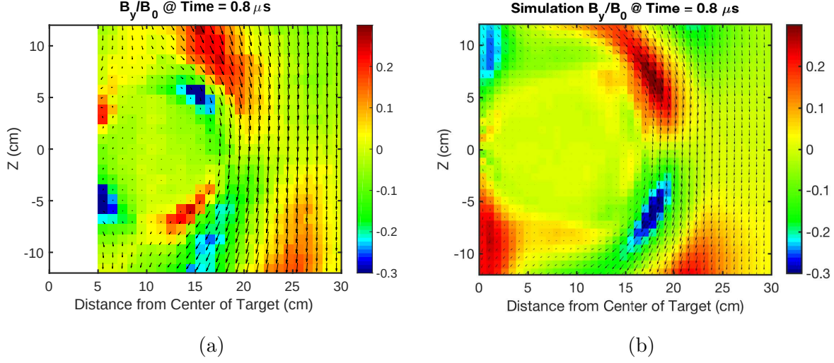
Figure 5.8: Shows (a) measured experimental B_y in an X-Z oriented plane at t = 0.8\mu s , with arrows over-plotted to show direction and magnitude of transverse B field, and (b) the corresponding output from fHybrid3D.
