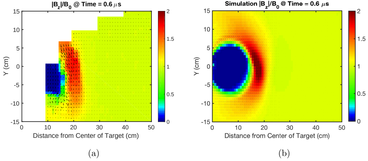
Figure 5.3: Shows (a) measured experimental B_z in an X-Y oriented plane at t = 0.6 \mu s , with arrows over-plotted to show direction and magnitude of transverse B field, and (b) the corresponding output from fHybrid3D.
