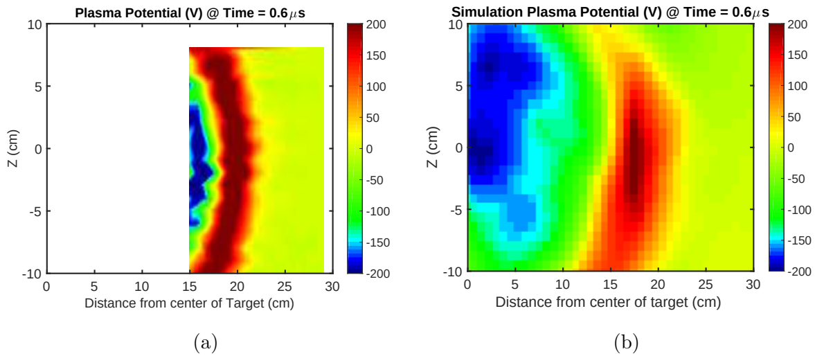
Figure 5.13: Shows (a) measured experimental \phi in an X-Z oriented plane at t = 0.6 \mu s and (b) the corresponding output from fHybrid3D.
