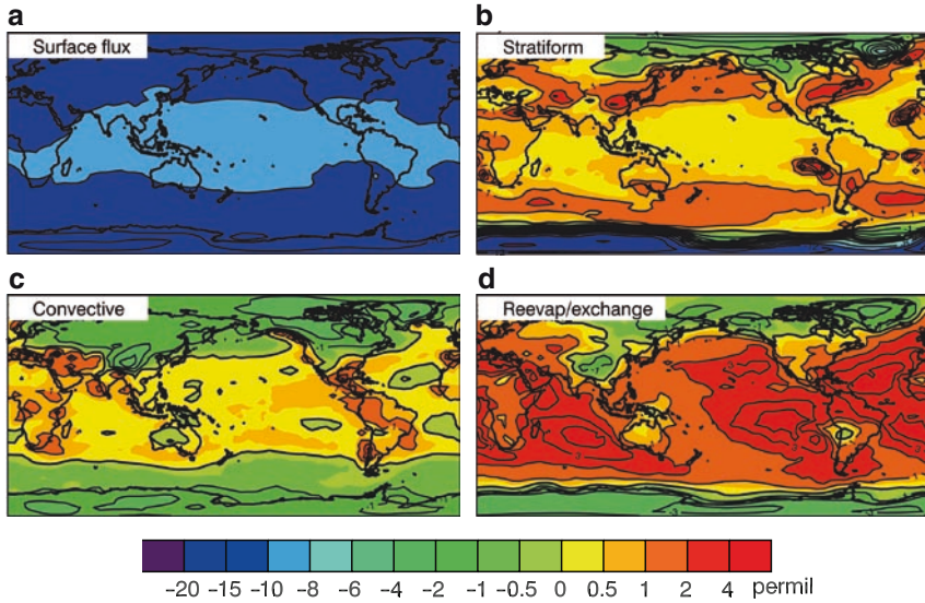
Fig. 10.2 Global model simulation of annual mean \delta^{18}\text{O} in precipitation (‰) in a global isotope model with (a) fractionation only associated with surface evaporative sources and dew/frost sinks, (b) as in (a) but with fractionation also associated with stratiform condensation), (c) as in (a) but with fractionation also associated with convective condensation, and d) the influence of fractionation during exchange as raindrops fall from clouds. Panels (b) and (c) are differences relative to (a), and panel (d) is a difference relative to a control simulation that has all fractionations, and is shown in Fig. 10.4b. To the degree to which the model results are linear, the (weighted) sum of all four components composes the total isotope signal. Fig. 10.2, see Appendix 1, Color Section
