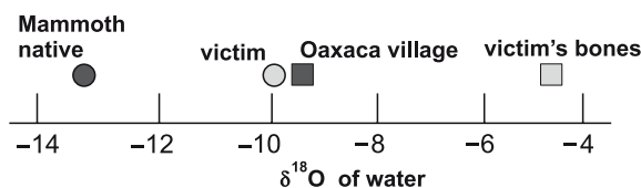
Fig. 16.9 Isotopic tracing of an unidentified murder victim from Mammoth Lakes, California. Data represent \delta^{18}\text{O} values of drinking water corresponding to analyses of teeth and bone (Based on unpublished data from HPS)
