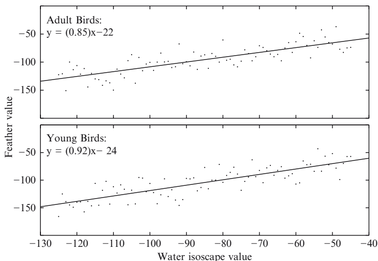
Fig. 12.1 Simulated \delta^2\text{H} data for feathers of known origin from birds of two different age classes. Lines are regressions of \delta^2\text{H} in feathers on predicted values for \delta^2\text{H} at the known origins from a water-based isoscape (Bowen et al. 2005). Simulated data were generated from the equations shown along with error structure given by the Normal distribution \mathcal{N}(\mu, \sigma^2) with \mu = 0 and \sigma^2 = 196 for both age classes. The linear models shown were used to calibrate the water-based isoscape from Bowen et al. (2005) for use in determining spatially explicit probability densities for feathers of unknown origin. See text for details
