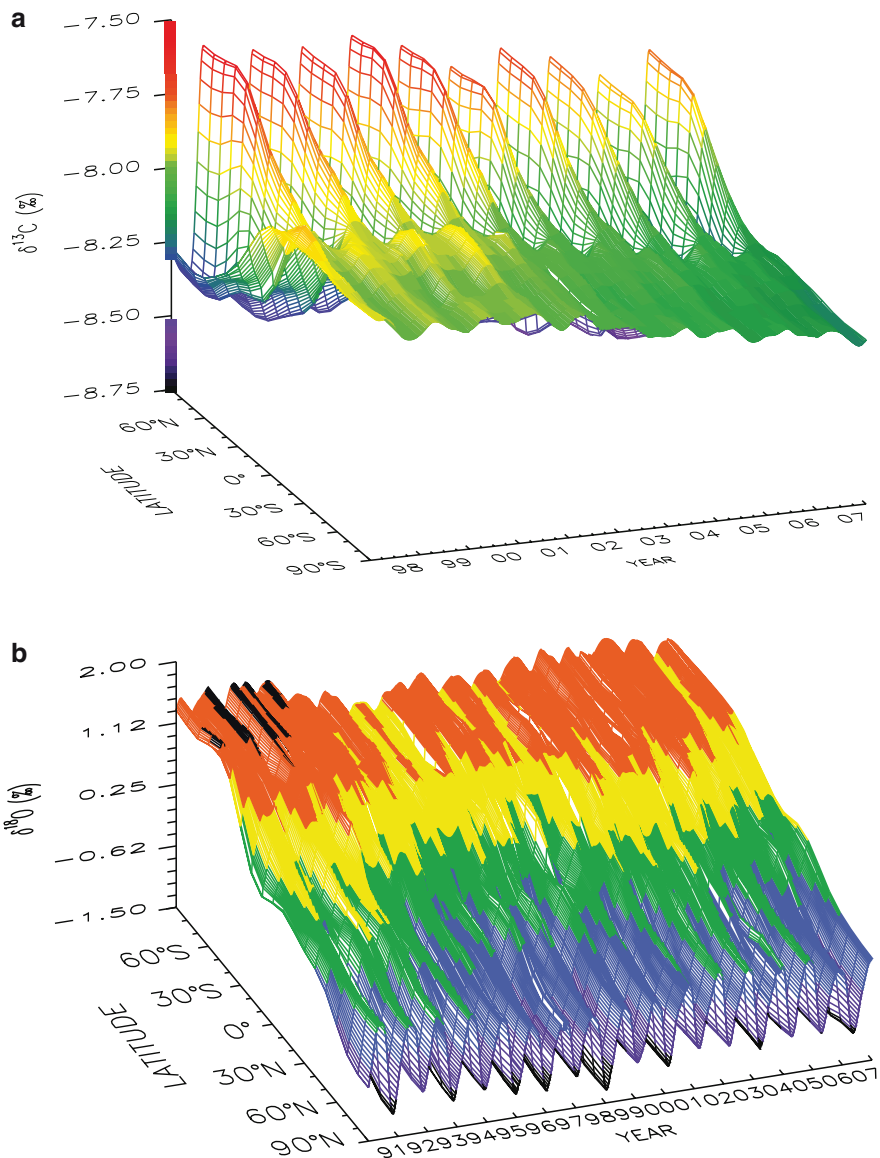
Fig. 1.4 (a) Surface plot of spatial \delta^{13}\text{C} - \text{CO}_2 data from the NOAA/INSTAAR global flask network through time, created from 55 sites from south to north. (b) Surface plot of spatial \delta^{18}\text{O} - \text{CO}_2 data from the NOAA/INSTAAR global flask network through time, created from 55 sites. Note the y-axis is reverse of the \delta^{13}\text{C} - \text{CO}_2 plot, from north to south, in order to better display the large latitudinal gradient. Fig. 1.4, see Appendix 1, Color Section
