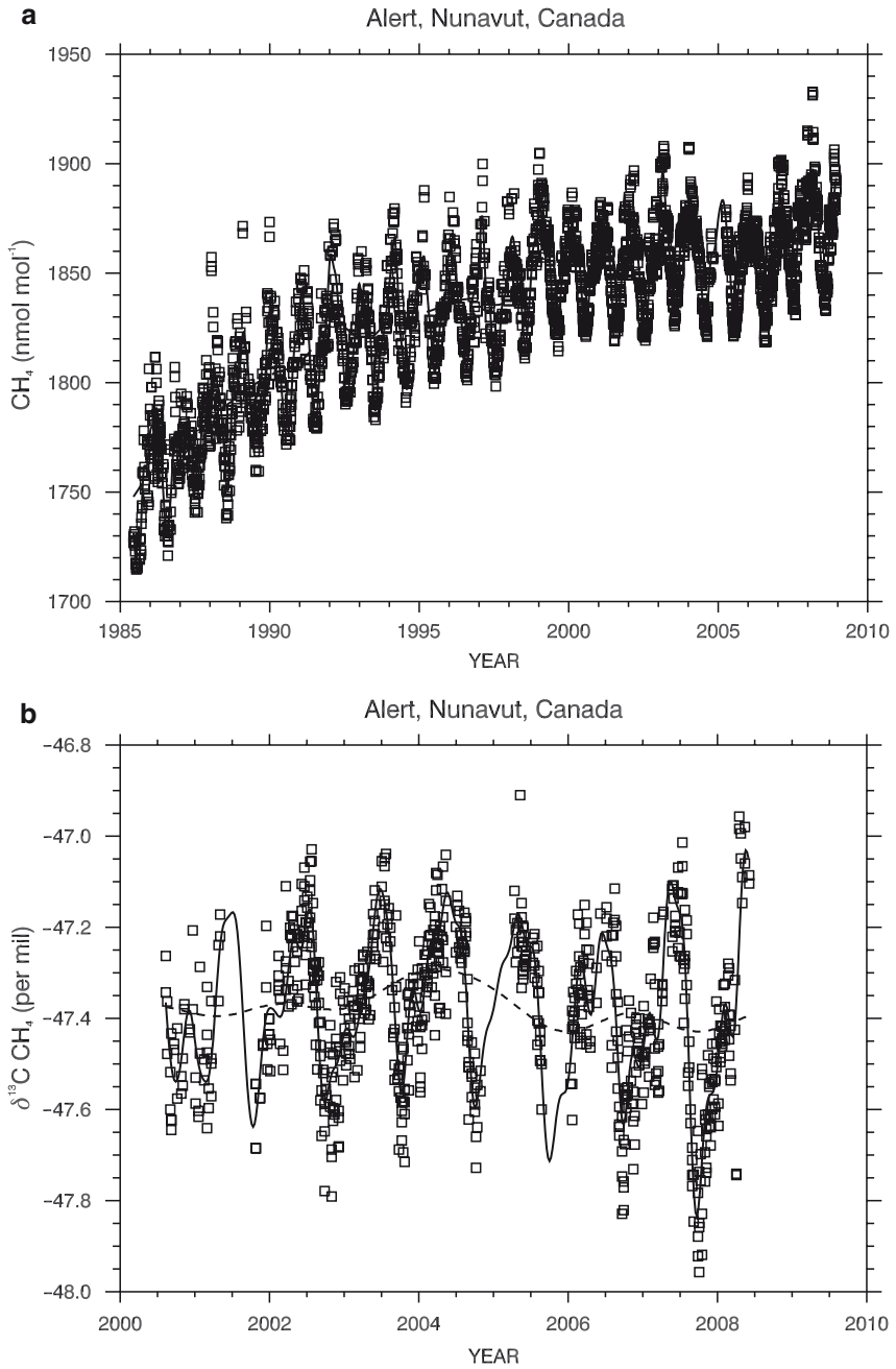
Fig. 1.6 Plot showing atmospheric concentration of methane and \delta^{13}\text{C} of methane collected at Alert, Canada (N 82.45 W -62.52, 200 m.a.s.l.) showing changes in 2007
