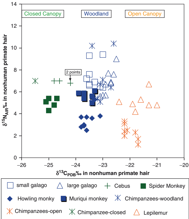
Fig. 15.1 \delta^{13}C values in hair from across primate species reflect the level of canopy cover in the areas in which the animals lived irrespective of their specific diets (indicated by \delta^{15}N values, see text for discussion). Two species of New World monkeys from closed canopies show values around -26\text{‰} to -24.5\text{‰} . Two other species of New World monkeys, two species of African prosimians, and a population of chimpanzees, which all live in deciduous woodland regions show values around -24\text{‰} to -23\text{‰} . One species of prosimian from Madagascar and a population of chimpanzees living in open canopy savanna-woodland habitats have values between -22 and -21\text{‰} (Data from Schoeninger et al. 1997, 1998, 1999)
