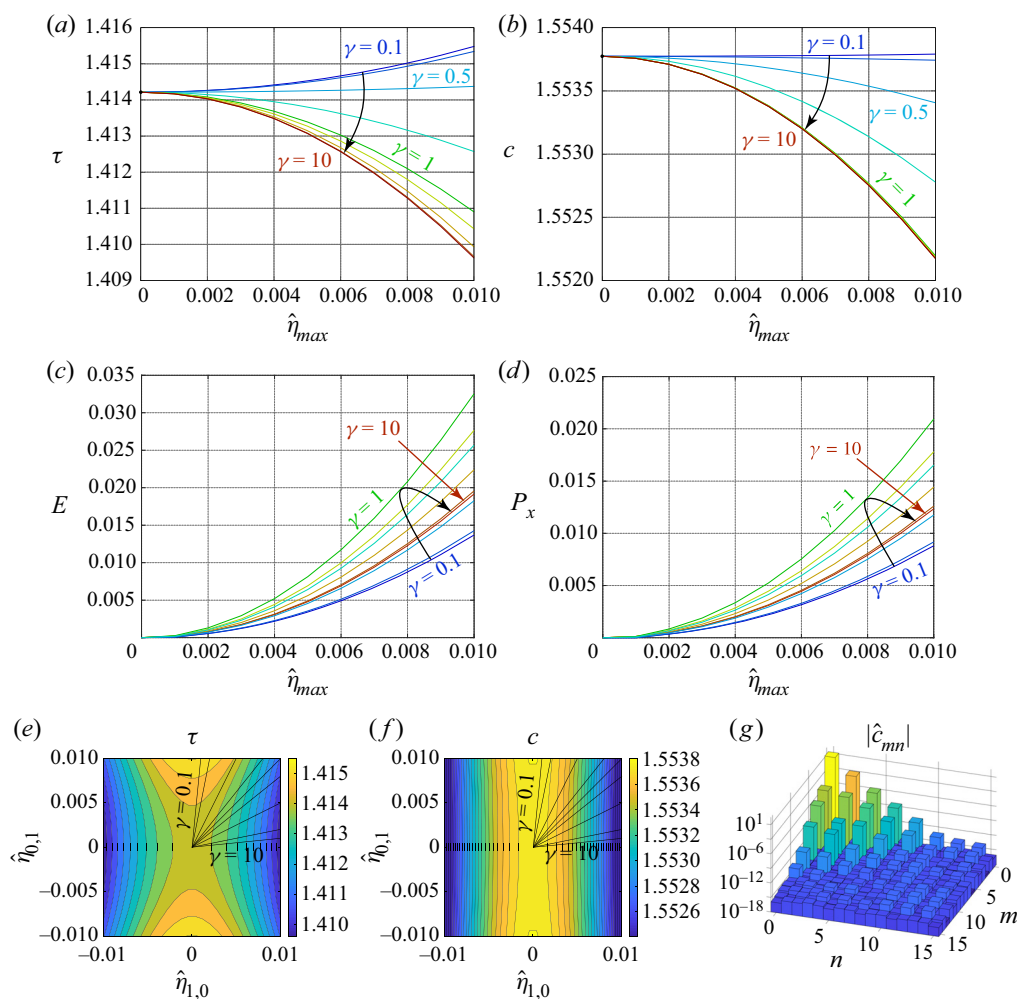
Figure 4. Surface tension, wave speed, energy and momentum of small-amplitude quasi-periodic water waves with k = 1/\sqrt{2} . (a–d) Plots of \tau , c , E and P_x versus \hat{\eta}_{max} = \max\{\hat{\eta}_{1,0}, \hat{\eta}_{0,1}\} holding \gamma = \hat{\eta}_{1,0}/\hat{\eta}_{0,1} fixed. The black arrow in each plot shows how the curves change as \gamma increases from 0.1 to 10. (e, f) Contour plots of \tau and c and the rays of constant \gamma corresponding to (a, b). (g) Mode amplitudes of a two-dimensional Chebyshev expansion of c(\hat{\eta}_{1,0}, \hat{\eta}_{0,1}) over the rectangle -0.01 \leq \hat{\eta}_{1,0}, \hat{\eta}_{0,1} \leq 0.01 .
