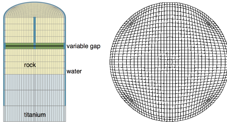
Figure 11. Numerical mesh developed for simulating THMC experiments. Left – Side profile with upper surface depicting grid blocks and elements (dark blue – water; light blue – titanium; yellow – rhyolite); Right – Plan view of grid
