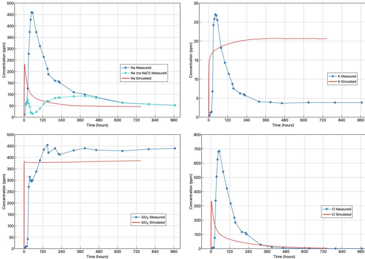
Figure 14. Comparison of simulated (solid red lines) and observed (solid blue lines with dots) fluid compositions for run 1 of the rhyolite ash-flow tuff experiment. The Na plot also includes a correction for NaCl (removing all of the Cl and a stoichiometrically equivalent amount of Na), plotted as a light blue line with dots.
