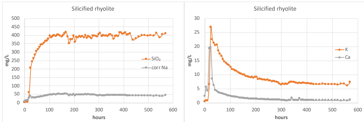
Figure 6. Plots of effluent composition vs. time for Stripa granite, rhyolite ash-flow tuff, metasediment, and silicified rhyolite samples. The rhyolite ash-flow tuff samples are plotted as the combination of two successive runs. For the second run of the rhyolite ash-flow tuff experiment, no water samples were analyzed after 1896 h – the “final” water composition plotted for this run is an average of the previous three water compositions that were analyzed for this run.
