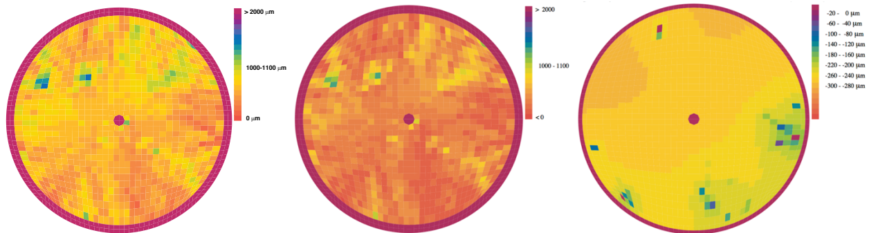
Figure 12. Modeled fracture apertures and change in aperture for simulated rhyolite ash-flow tuff experiment. Left – Fracture aperture (microns) for unloaded sample. Center – Fracture aperture (microns) under 20.7 MPa vertical effective stress. Right – change in aperture caused by loading (microns).
