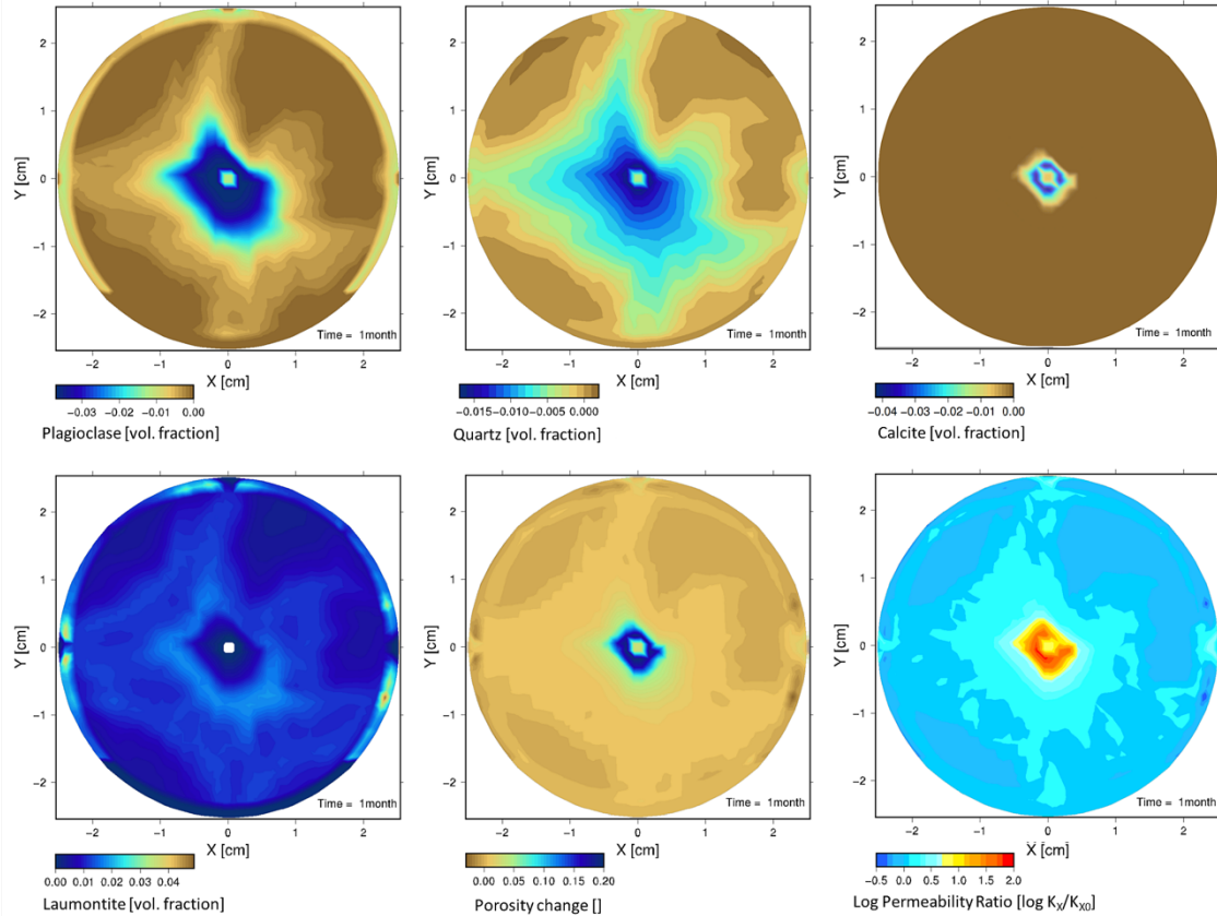
Figure 13. THC modeling of changes in mineral abundance, porosity, and permeability after 1-month simulation. Upper row – Volume changes due to dissolution of plagioclase, quartz, and calcite. Lower row – Volume changes due to precipitation of laumontite, and resulting changes in fracture porosity and permeability.
