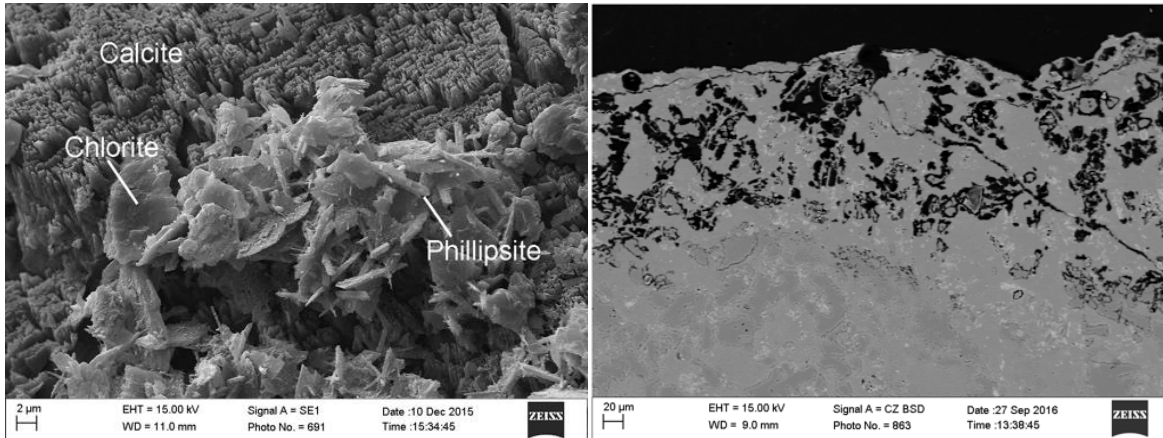
Figure 9. SEM images of metasediment after experiment. Left – SE image of calcite with abundant dissolution pits, and platy crystals of chlorite and prismatic crystals of phillipsite coating the surface. Right – Cross sectional BSE view of fracture surface indicating a ~150-micron thick zone adjacent to the fracture surface with abundant dissolution – likely of calcite and quartz. Note the increased relative abundance of the darker mineral phase (quartz) in the unreacted lower portion of the image.
