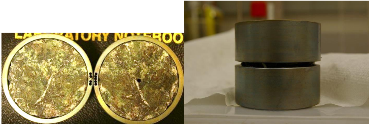
Figure 3. Fractured core sample set-up. Left – Fractured core of BCH-03 metasedimentary rock. Pin and holes in titanium sleeve allow for rotational offset of core samples to create self-propped fractures. Hole in the right rock sample is used as a port to inject fluid into the fracture. Core samples are 50.4 mm in diameter. Right – Jacketed rock core samples (with fracture between titanium sleeves) ready for insertion into pressure vessel.
