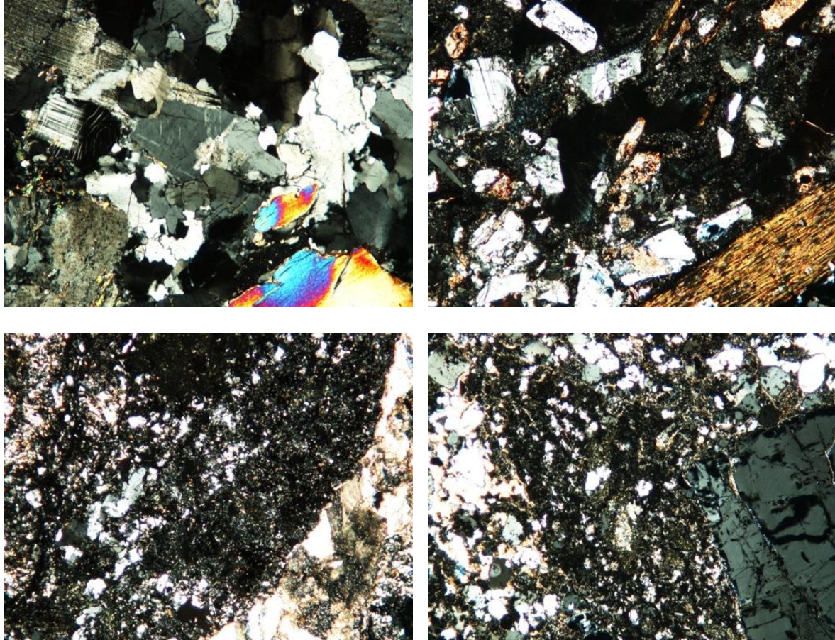
Figure 2. Photomicrographs (crossed nicols) of thin sections from rock samples used in study – bottom dimension of all photos is 1.75 mm. Upper left – Stripa granite, with microcline (cross-hatched twinning), plagioclase, quartz (undulatory extinction), and muscovite (high birefringence); Upper right – BCH-03 rhyolite ash-flow tuff, with phenocrysts of plagioclase (twinned), sanidine, quartz, and biotite (bird's eye extinction) in an altered groundmass; Lower left – BCH-03 metasediment with fine grains of quartz in a clay-chlorite-rich groundmass, cut by a calcite vein on the right side; Lower right – DP35-13 silicified rhyolite tuff with large plagioclase phenocryst, smaller plagioclase, quartz, and sanidine crystals in a silicified groundmass.
