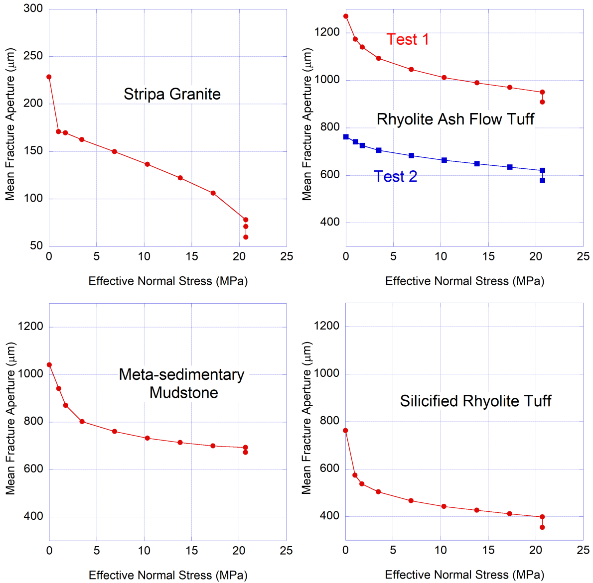
Figure 4. Initial fracture closing under uniaxial loading. The pore pressure was first set at 10.3 MPa, and all plotted measurements (except the final point) were conducted at room temperature.
