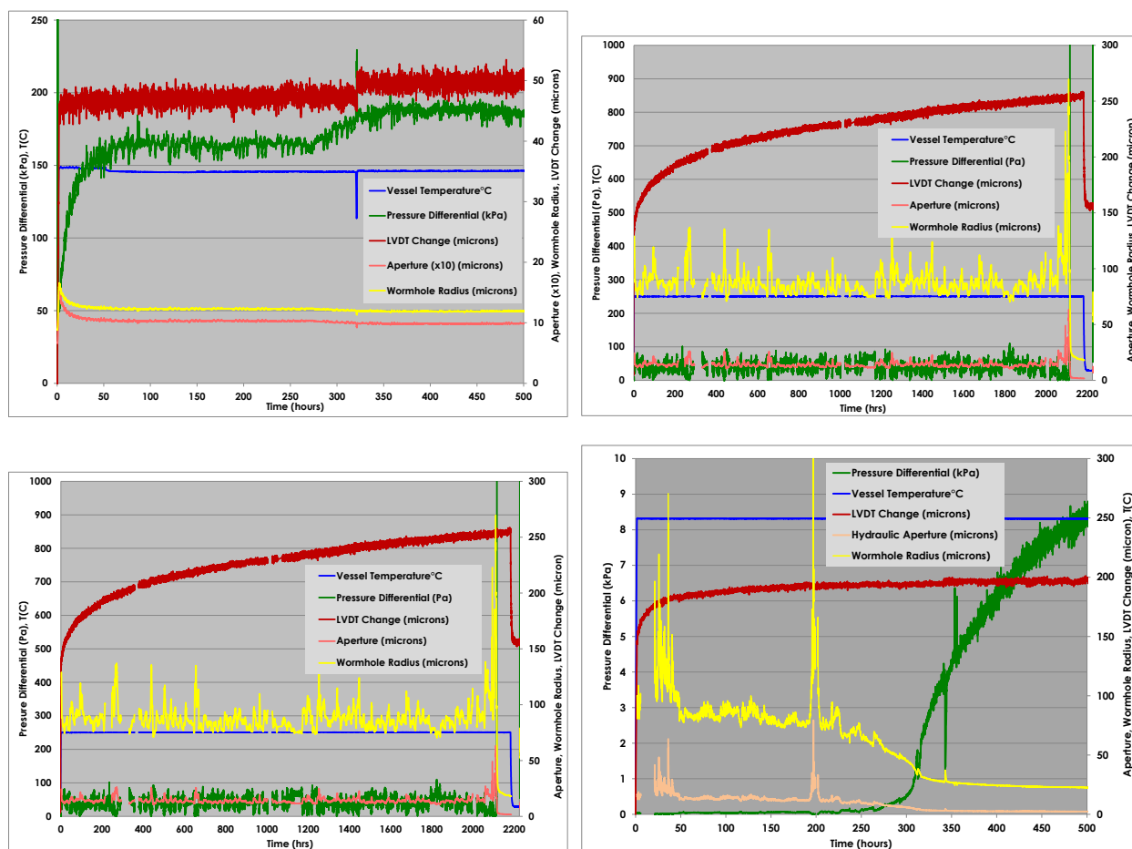
Figure 5. Changes in temperature, sample compression (LVDT change), differential flow pressure, and computed planar aperture and wormhole dimensions for test runs. Upper left – granite; Upper right – rhyolite ash-flow tuff (run 2); Lower left –metasediment; Lower right – silicified rhyolite tuff.
