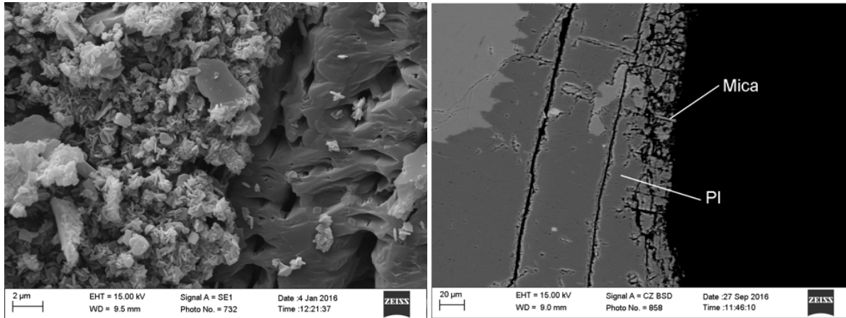
Figure 7. SEM images of granite after experiment. Left – Secondary electrons (SE) image of fracture surface with albite crystal with dissolution pits and newly crystallized diaspore rosette crystal aggregates. Right – Cross sectional backscattering (BSE) view of fracture surface indicating dissolution of albite near the fracture surface along microfractures (likely corresponding to cleavage planes).
