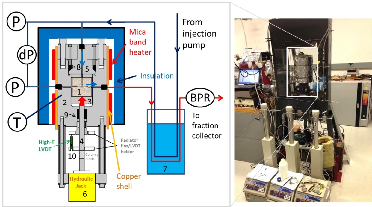
Figure 1. Schematic depiction (left) and photograph (right) of apparatus for fracture sustainability experiments. In diagram, 1 – fractured rock sample, 2 – titanium pressure vessel, 3 – platform, 4 – shaft, 5 – top, 6 – hydraulic jack, 7 – temperature equalizer bath, 8 – top seal, 9 – bottom seal, 10 - linear voltage differential transducer (LVDT), BPR – back pressure regulator.
