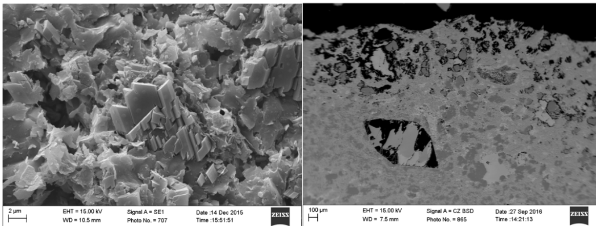
Figure 8. SEM images of rhyolite ash-flow tuff after experiment. Left – SE image of fracture surface depicting platy growth of illite/smectite and prismatic crystals of phillipsite. Right – Cross sectional BSE view of fracture surface where three distinct mineral phases can be identified by their backscatter signal intensity – the lightest colored phase is calcite, the intermediate density phase is plagioclase, and the darkest color is quartz. There is a ~400-micron thick zone adjacent to the fracture surface with abundant dissolution – likely of calcite, quartz, and plagioclase. A grain composed by calcite and plagioclase displaying a high degree of dissolution is present in the lower left of this image.
