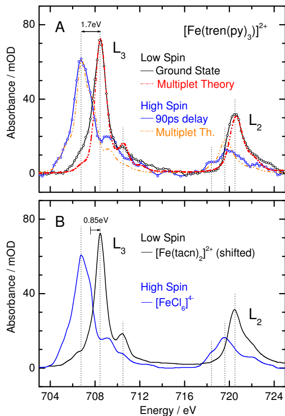
Figure 5. X-ray absorption spectra of various FeII complexes. (A) L-edge spectra of the low-spin ground state and photo-initiated transient high-spin state at 90 ps delay, reconstructed from the differential absorption spectrum in Figure 4B by estimating that (18 \pm 2)\% of the molecules were excited (black and blue open circles with spline fit, respectively) and charge transfer multiplet calculations (black and blue dotted lines). (B) Rescaled L-edge spectra of three crystalline compounds: [\text{Fe}(\text{tacn})_2]^{2+} and [\text{FeCl}_6]^{4-} (solid dark red and blue line, respectively, both from ref 50 measured with an energy resolution of 0.2 eV) and [\text{Fe}(\text{tpp})(\text{ImH})_2]^{2+} (dash-dotted black line, taken from ref 51 measured with an energy resolution of 0.15 eV). See text for further details.
