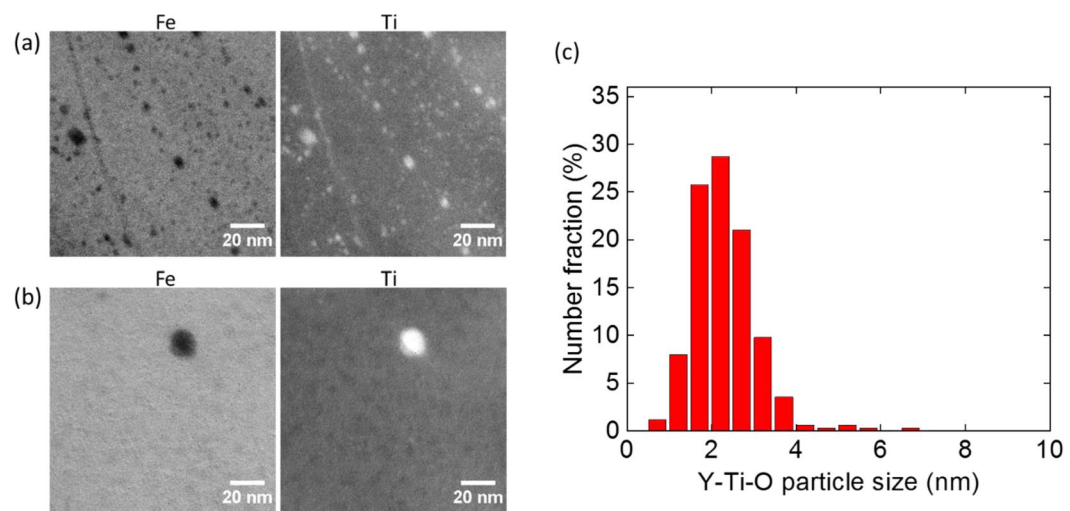
Figure 3. EFTEM Fe and Ti jump ratio maps obtained from (a) a small grain ( <0.5\ \mu\text{m} ) and (b) a large grain ( >2\ \mu\text{m} ), and (c) NO size distribution in small grains after 6 dpa neutron irradiation at 385–430 °C.
