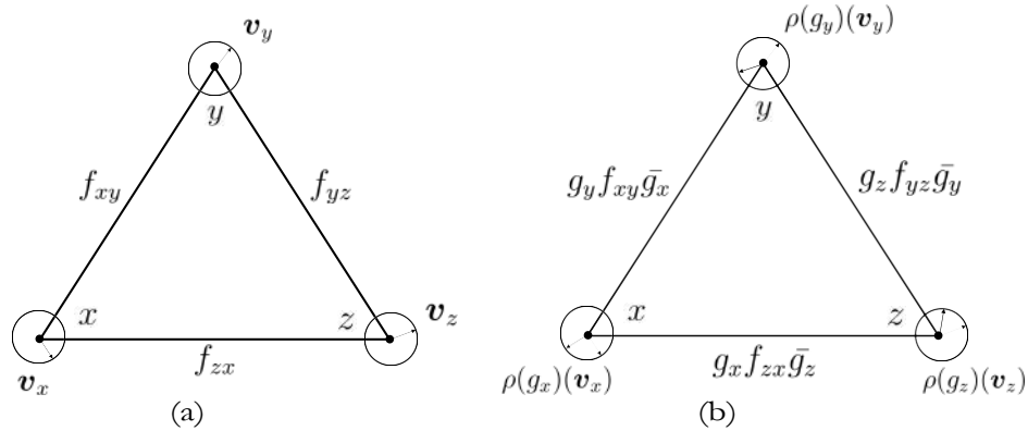
Figure 1: Illustration of lattice gauge theory. (a) Assignment of state vectors \mathbf{v}_x , \mathbf{v}_y and \mathbf{v}_z to vertices x, y, z and of group elements f_{xy} , f_{yz} , and f_{zx} to edges of a graph \Gamma . (b) Assignment after local gauge transformation with group representations acting on state vectors, \mathbf{v}'_x = \rho(g_x)(\mathbf{v}_x) , \mathbf{v}'_y = \rho(g_y)(\mathbf{v}_y) , and \mathbf{v}'_z = \rho(g_z)(\mathbf{v}_z) , and transformed fields f'_{xy} = g_y f_{xy} \bar{g}_x , f'_{yz} = g_z f_{yz} \bar{g}_y , and f'_{zx} = g_x f_{zx} \bar{g}_z . The group inverses are indicated by the bar.
