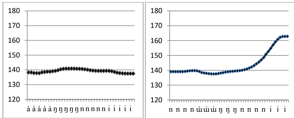
Figure 14. Genitive inflection and tone shift. Averaged time normalized pitch contour for the nouns aṃni 'I-Gen' in the left panel and that of nuṃni 'you-Gen' in the right panel (n=25). The genitive suffix -ni surfaces with a rising contour in nuṃni 'you-Gen' as the high tone of núṃ 'you' moves to the right edge.
