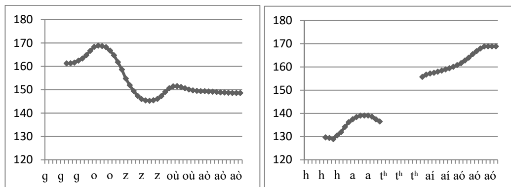
Figure 9. Locative inflection and tone spreading. Averaged time normalized pitch contour for the nouns gozouàò ‘water-Loc’ and hat h aiaó ‘house-Loc’ (n=25)
