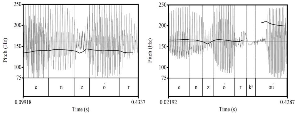
Figure 16. Accusative inflection and absence of tone shift. Pitch contours for the noun enzòr ‘rat’ with and without the accusative case marker -k^hou . The lexical high specification of the accusative case marker -k^hou surface in the presence of the disyllabic stem enzòr ‘rat’.
