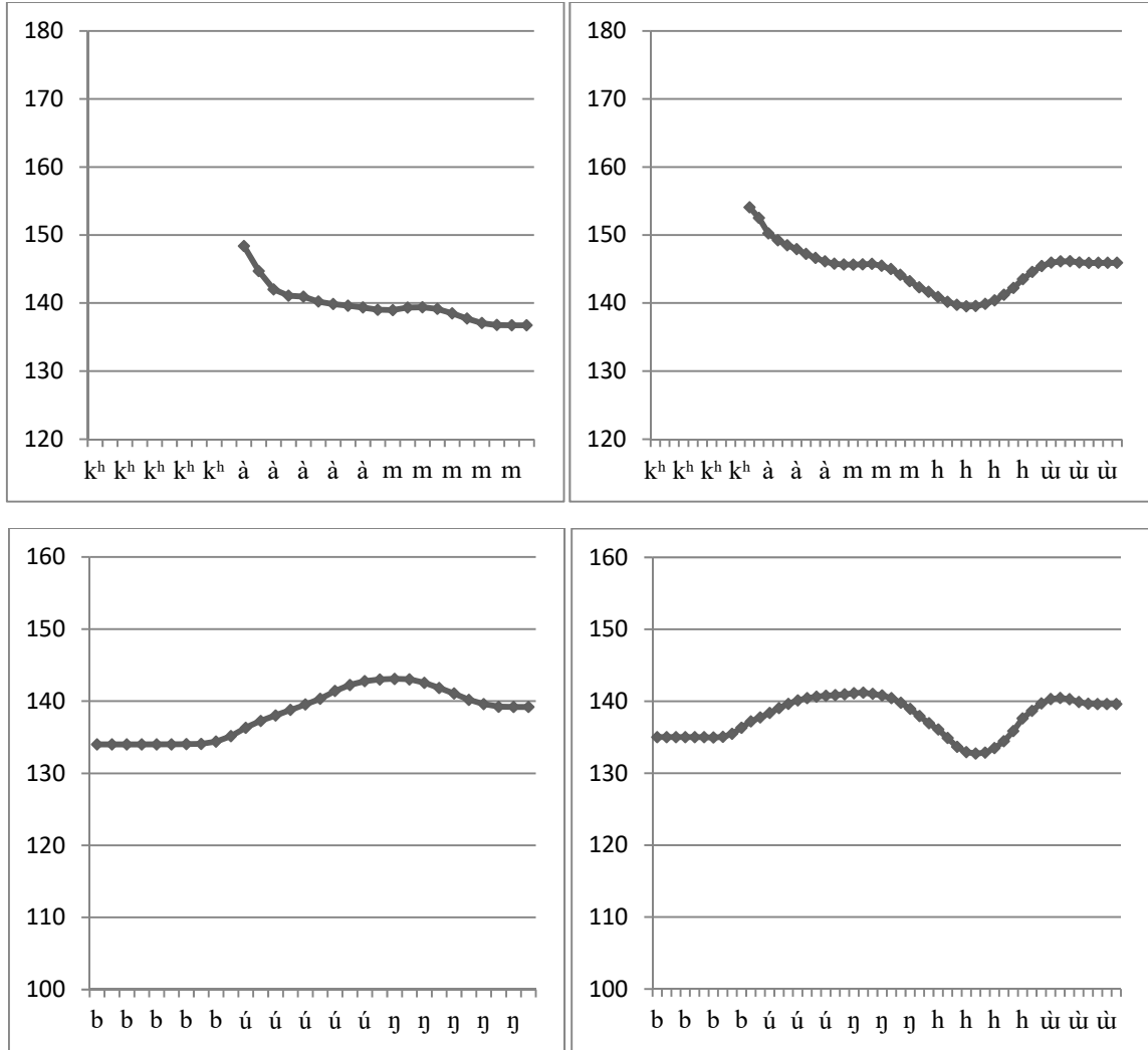
Figure 11. Monosyllabic stem and absence of tone shift. Averaged time normalized pitch contour for the causative verbs k h àmhù ‘to cause a fire’ and búnghù ‘to cause to speak’ derived from the verb k h àm ‘fire’, and from the noun búngh ‘speak’. (n=25).
