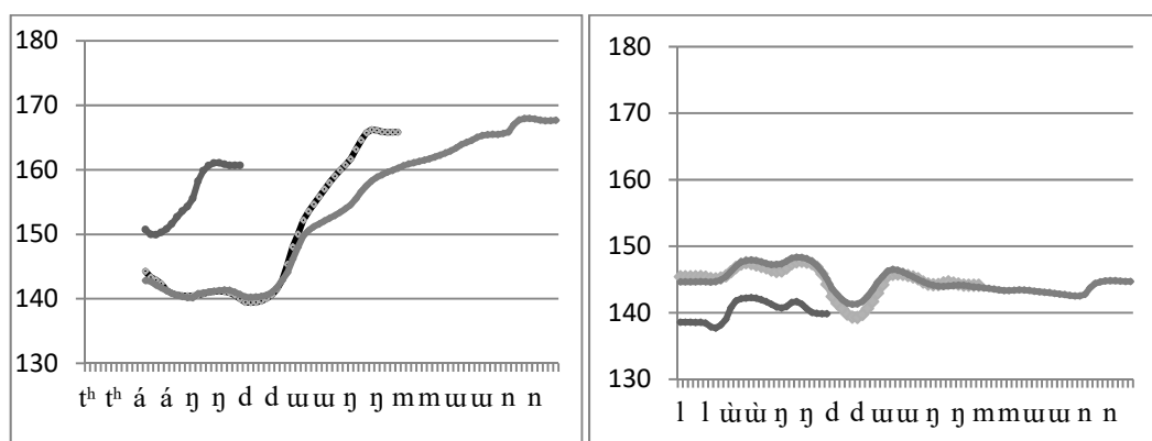
Figure 8. Tense aspect suffixes and tone spreading. Pitch contours of t h añ ‘go’ and lun ‘drink’ with the suffixes -dun and -mun where the lexical tone spreads to the third syllable.
