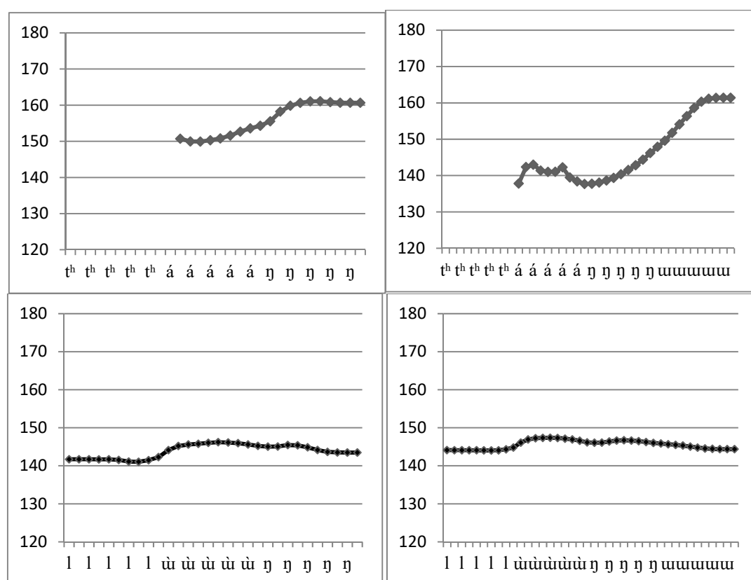
Figure 2. Tense-aspect suffix and tone shift. The upper panels show \text{t}^{\text{h}}\text{a}\eta 'go' with and without the habitual present marking suffix \text{-u} . The lower panels present the \text{f}_0 contour for \text{l}\eta\eta 'drink' with the same suffix. These are time normalized pitch contours for 25 iterations of each of the words (5 repetitions x 5 speakers)
