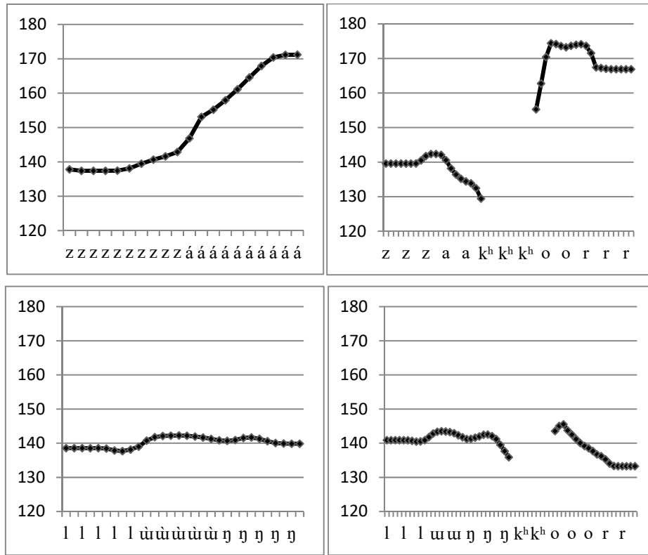
Figure 5. Adjectival suffix and tone shift. Averaged time normalized f_0 contour for the verb zá ‘eat’ and the adjective zak^hór ‘gluttonous’ in the upper panels and lùŋ ‘drink’ and the adjective luŋk^hòr ‘drunkard’ in the lower panels. (n=25)
