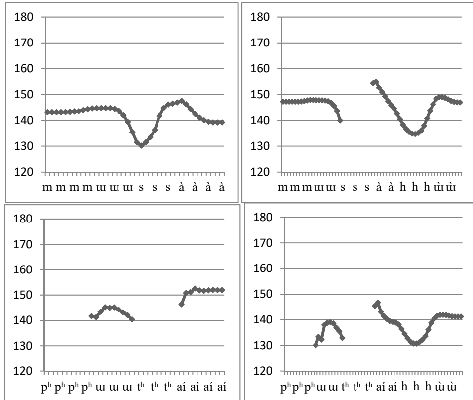
Figure 12. Disyllabic stem and no tone shift. Averaged time normalized pitch contour for the causative verbs musàhù ‘to cause to dance’ and pʰutʰaihù ‘to make someone believe’ from the verb musà ‘dance’ and the noun pʰutʰai ‘belief’. (n=25)
