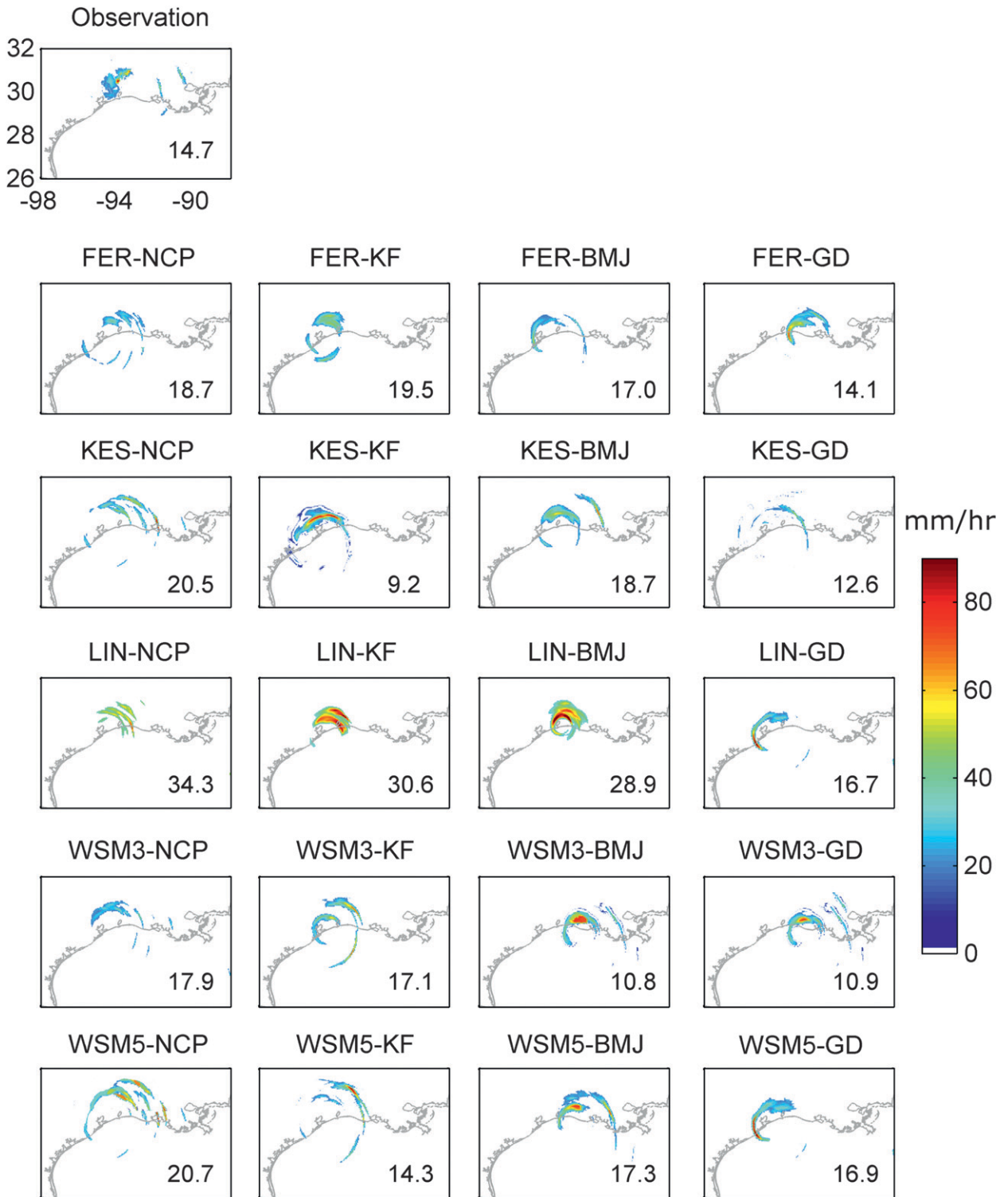
FIG. 3. (top) Observed and (bottom) simulated precipitation patterns ( \text{mm h}^{-1} ) above 90 percentiles at 1000 UTC 24 Sep 2005 (FER, KES, LIN, WSM3, WSM5, NCP, KF, BMJ, and GD). The threshold for each subfigure is shown in \text{mm h}^{-1} .
