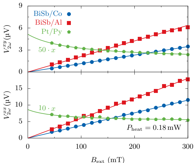
FIG. 4. The magnetic field dependence of the second harmonic voltage. In BiSb/Co and BiSb/Al a linear increase in voltage can be observed, as expected from the ordinary Nernst effect. In Pt/Py on the other hand the harmonic voltage is decreasing as expected from damping-like spin-orbit torque and unidirectional spin-Hall magneto-resistance respectively. Note that the voltage in Pt/Py has been enhanced for visual clarity.
