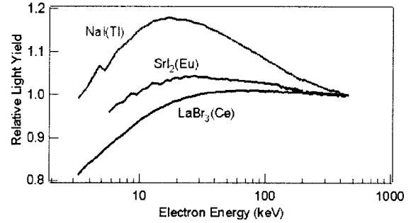
FIG. 6. (Color online) Relative light yields as a function of electron energy acquired using the SLYNCI reveal a proportional response for SrI 2 (Eu), in comparison to both LaBr 3 (Ce) and NaI(Tl).
