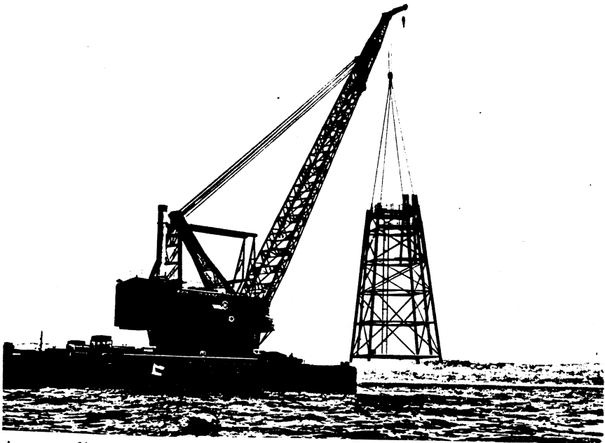
Large floating crane lowers the tower frame into the sea
