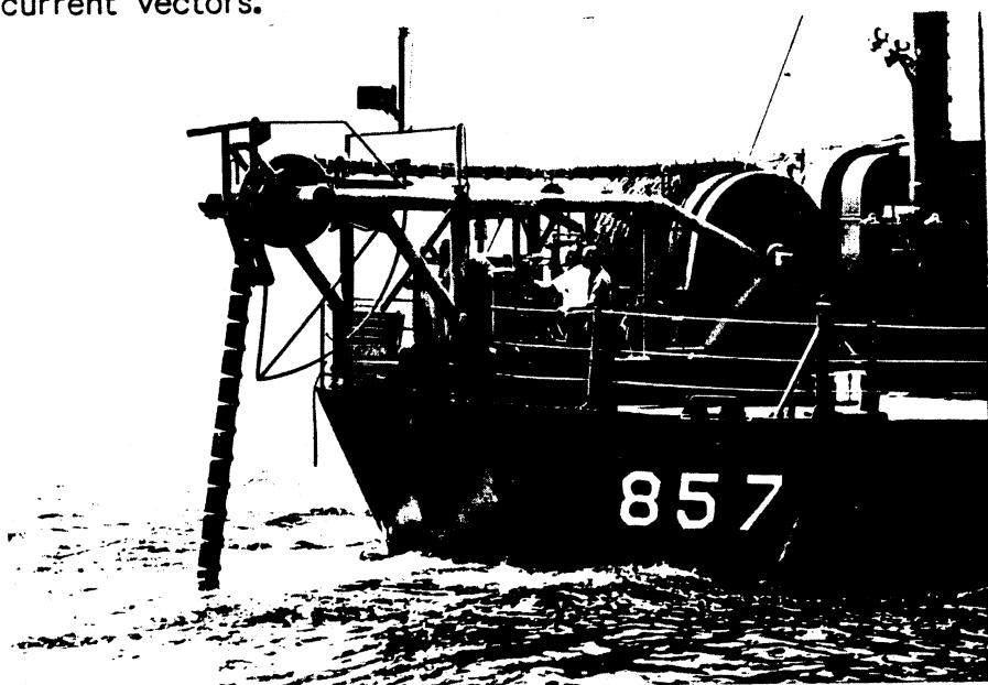
Thermistor chain on USS MARYSVILLE, 1961
