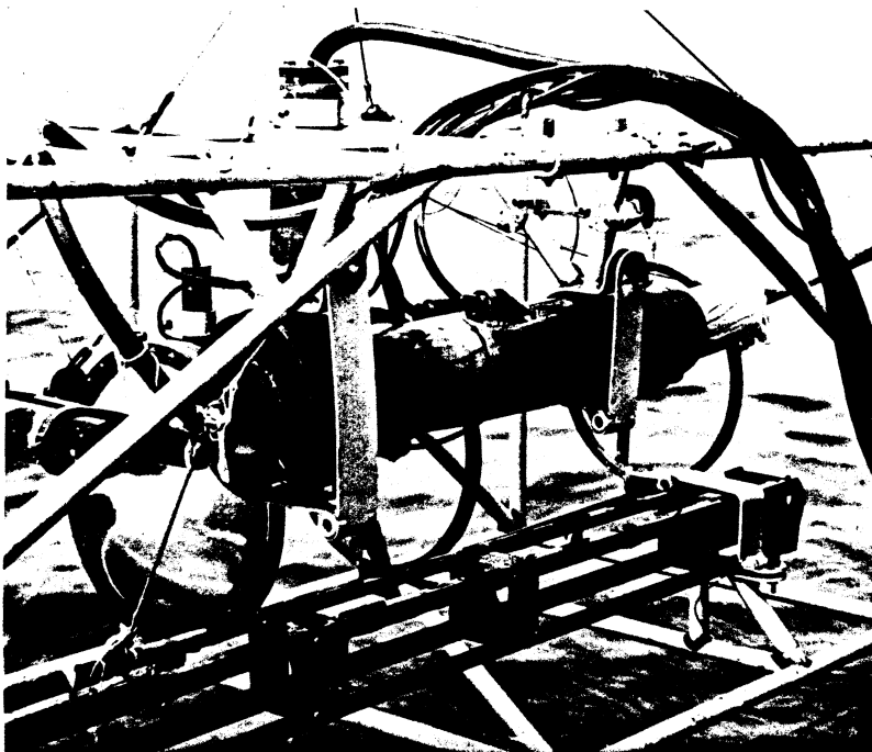
Framework of instruments used to measure oceanographic parameters related to acoustic detection of mines, 1954
