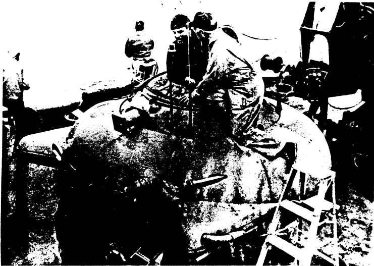
Eugene on Soucoupe Marine getting ready for launch (1964)
