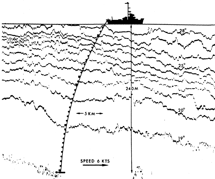
Schematic of towing the thermistor chain and the isotherms which it records
