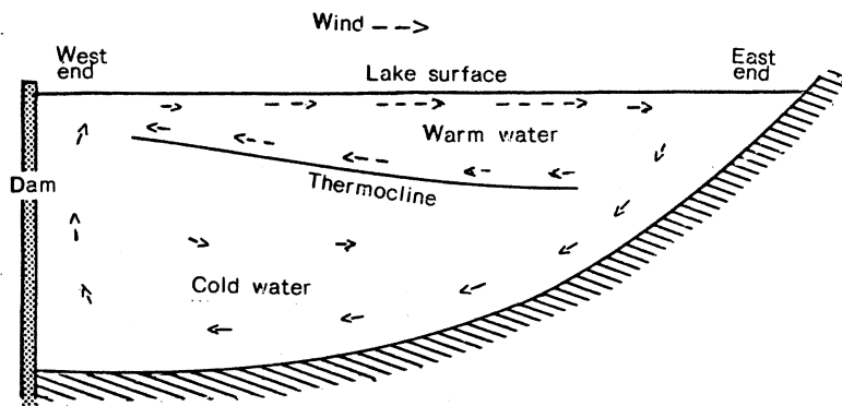
Water circulation determined in Sweetwater Lake in the summer of 1957
