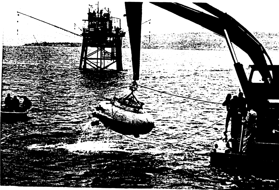
Launching of Soucoupe Marine near oceanographic tower
