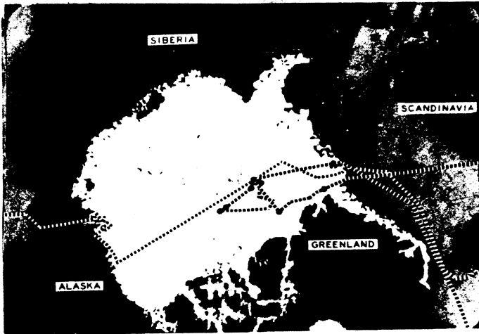
Tracks of SSN NAUTILUS (1957) and SSN SKATE (1958) in the Arctic Ocean under the ice cap. Dots indicate locations of SKATE'S surfacings
