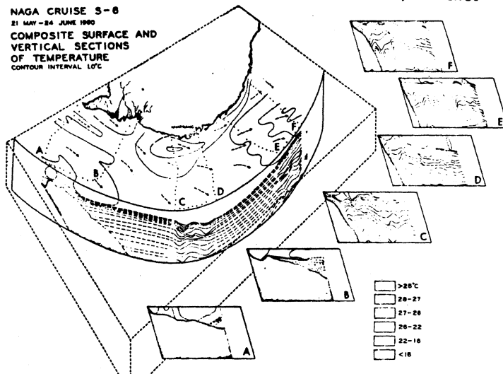
Chart of water structure off Vietnam in the South China Sea developed from the NAGA Expedition
