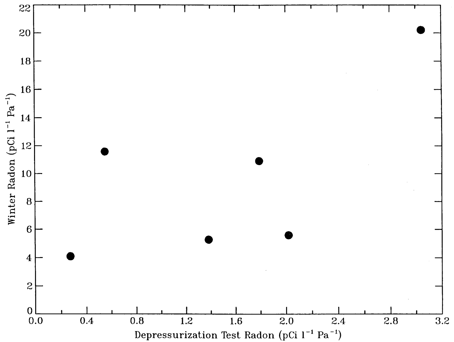
Figure 7 Time- and volume-averaged radon concentration per pascal of depressurization of heated zone in winter vs basement radon concentration per pascal of depressurization with blower door test.
