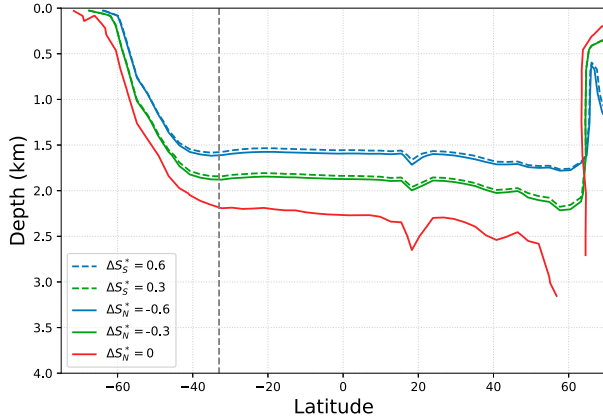
FIG. 9. Contours of the isopycnal that separates the two overturning circulation cells \rho_{\text{bdry}} , with potential density zonally averaged in the Atlantic Ocean (north of 33^\circ\text{S} ) and in the Atlantic sector of the Southern Ocean (south of 33^\circ\text{S} ) in the Southern Ocean perturbation runs (dashed) and the North Atlantic perturbation runs (solid). Only a subset of the runs is included for clarity. The red line represents the control run, which is equivalent to the North Atlantic perturbation run \Delta S_N^* = 0 and the Southern Ocean perturbation run \Delta S_S^* = 0 . The gray dashed line indicates 33^\circ\text{S} .
