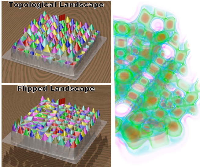
Fig. 12. Silicon dataset with average volume-to-area projection error of 1.0%. (Top left) Topological landscape. (Bottom left) Flipped landscape. (Right) traditional volume rendering.
