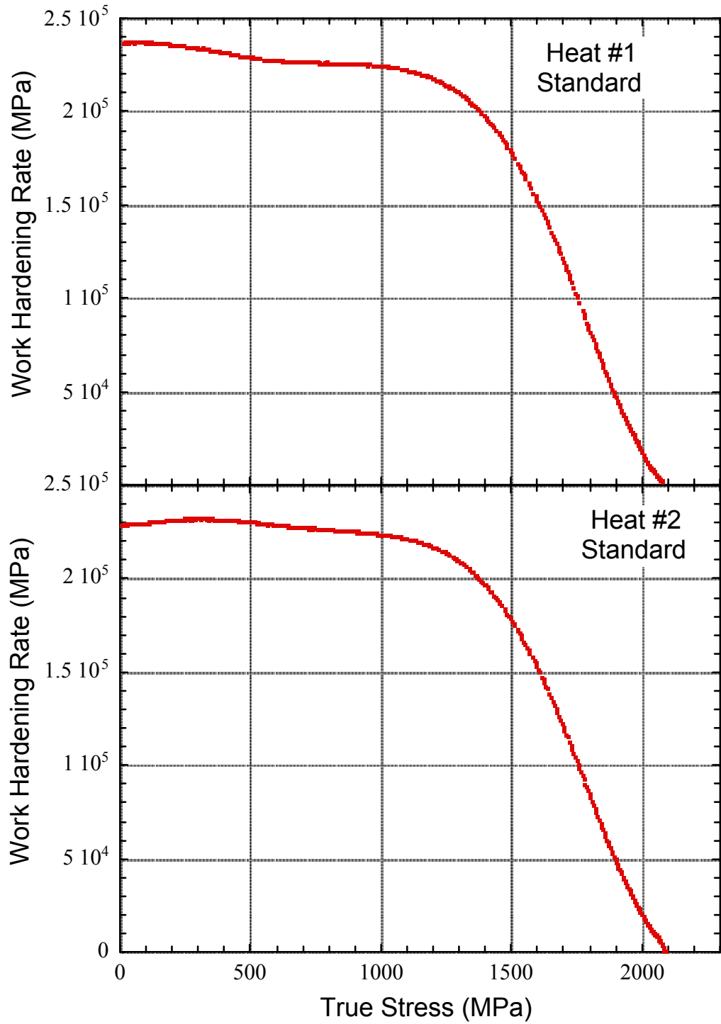
Figure A8 Work hardening rate – true stress curve. Standard heat treatment: (A) 885^{\circ}\text{C} \times 1\text{hr} , OQ + (DF) -197^{\circ}\text{C} \times 1\text{h} + (Ag) 482^{\circ}\text{C} \times 5\text{h} , OQ
