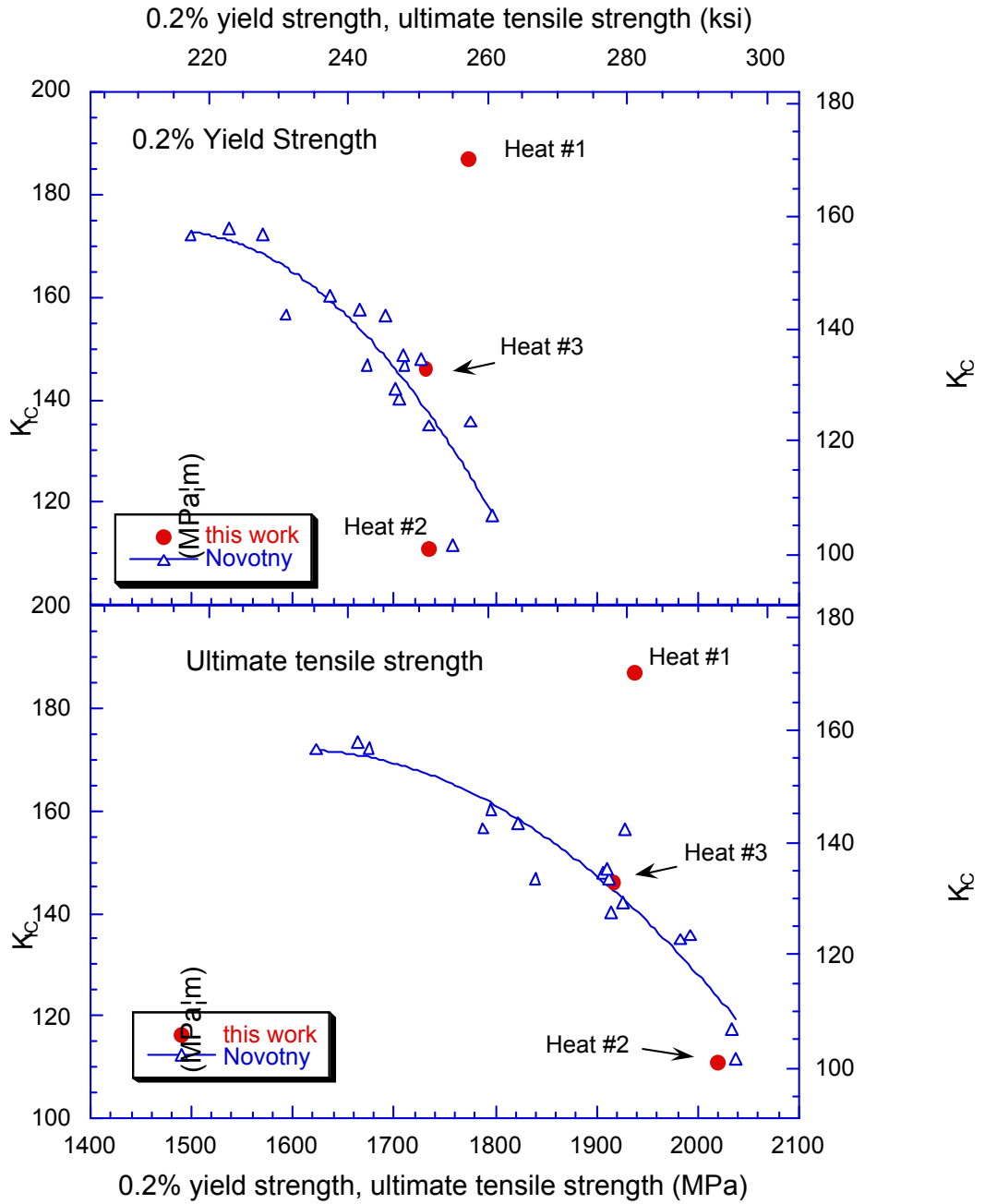
Figure 2.7 Relationship between fracture toughness and tensile strengths among three heats - All three heats of this study are treated in the standard heat treatment condition. - Novotny's data is obtained from a series of heat treatments of one heat.
