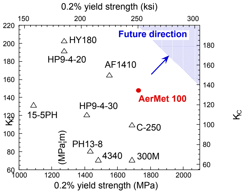
Figure 1.1 Relationship between fracture toughness, K_{Ic} , and 0.2% yield strength among several ultrahigh strength steels.
