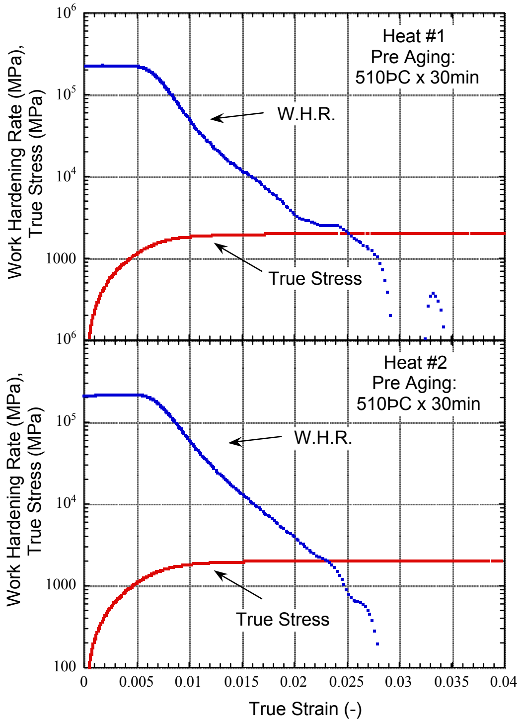
Figure 4.10 Effect of pre-aging on the work hardening rate – true strain curve. Heat treatment: (A) 885°C x 1h, OQ + (DF) -197°C x 1h + (PreAg) 510°C x 30min, OQ + (DF) -197°C x 1h + (Ag) 482°C x 5h, OQ
