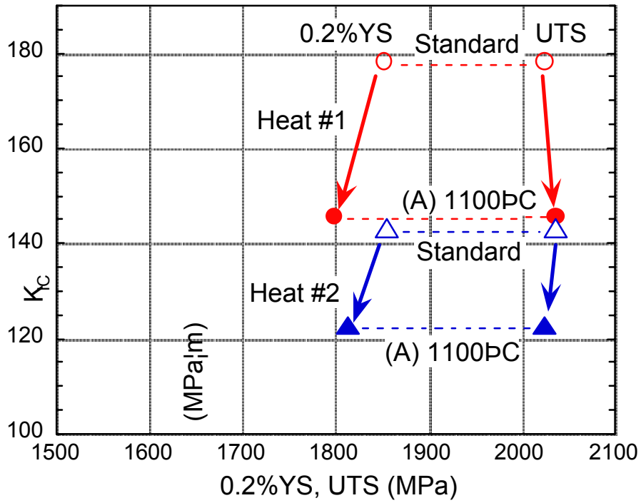
Figure 4.19 Effect of high temperature austenitization on the toughness-strength relationship.
