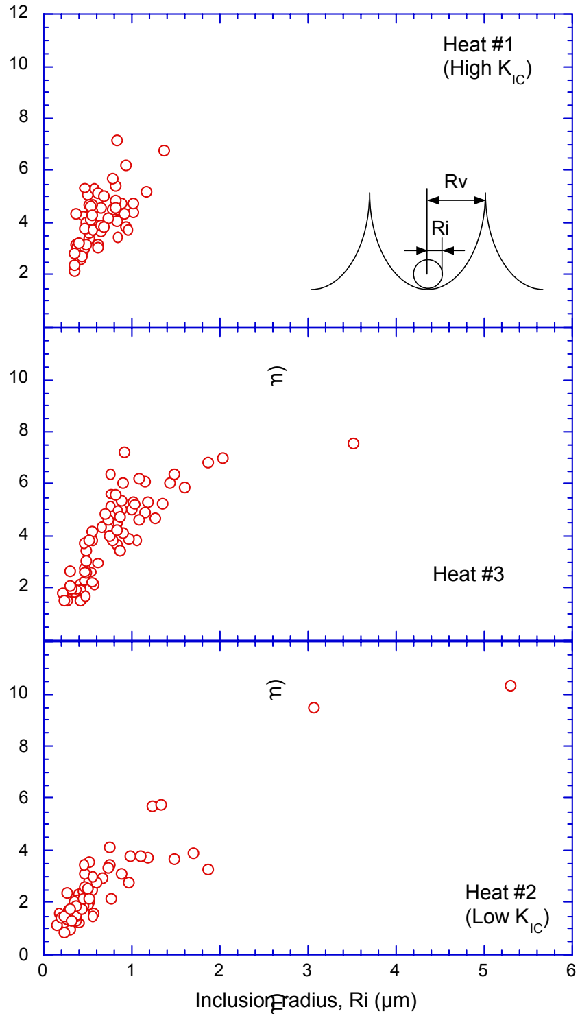
Figure 2.12 Relationship between the void radius and the inclusion radius sitting in the void
