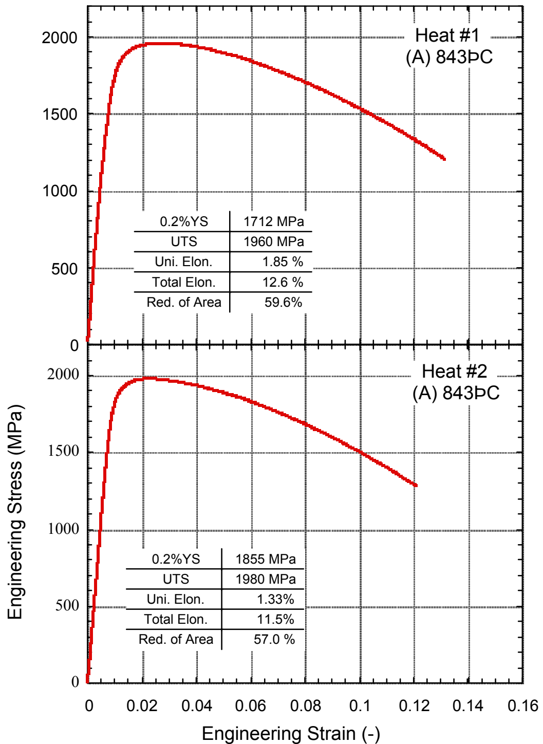
Figure A3 . Effect of low temperature austenitization on the engineering stress – engineering strain curve. Heat treatment: (A) 843°C x 1hr, OQ +(DF)-197°C x 1h + (Ag) 482°C x 5h, OQ
