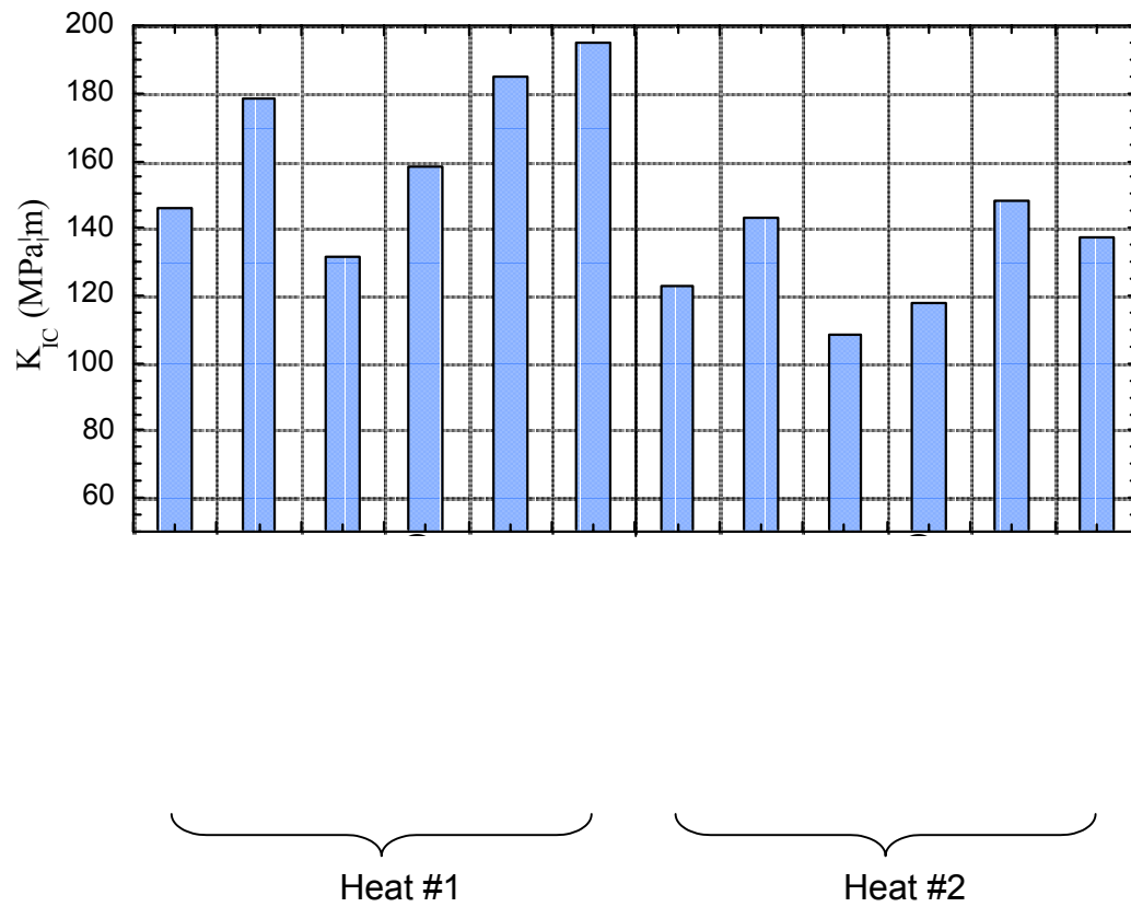
Figure 4.13 Effect of heat treatment conditions on K_{IC} .
