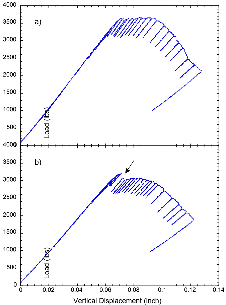
Figure 4.12 Examples of the load-displacement curves of the J-integral tests: a) slow stable crack propagation, and b) fast unstable crack propagation (marked by the arrow).
