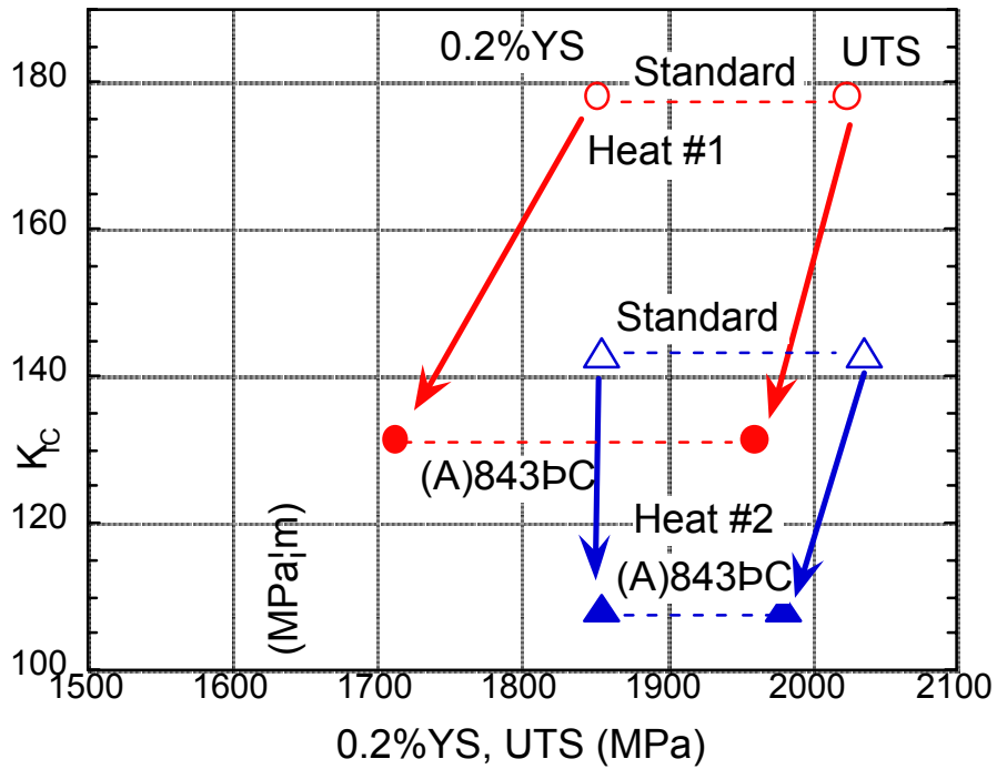
Figure 4.20 Effect of low temperature austenitization on the toughness-strength relationship.
