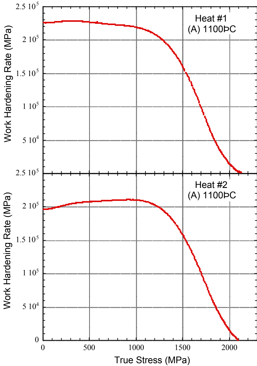
Figure A7 Effect of high temperature austenitization on the work hardening rate – true stress curve. Heat treatment: (A) 1100°C x 1hr, OQ +(DF)-197°C x 1h + (Ag) 482°C x 5h, OQ
