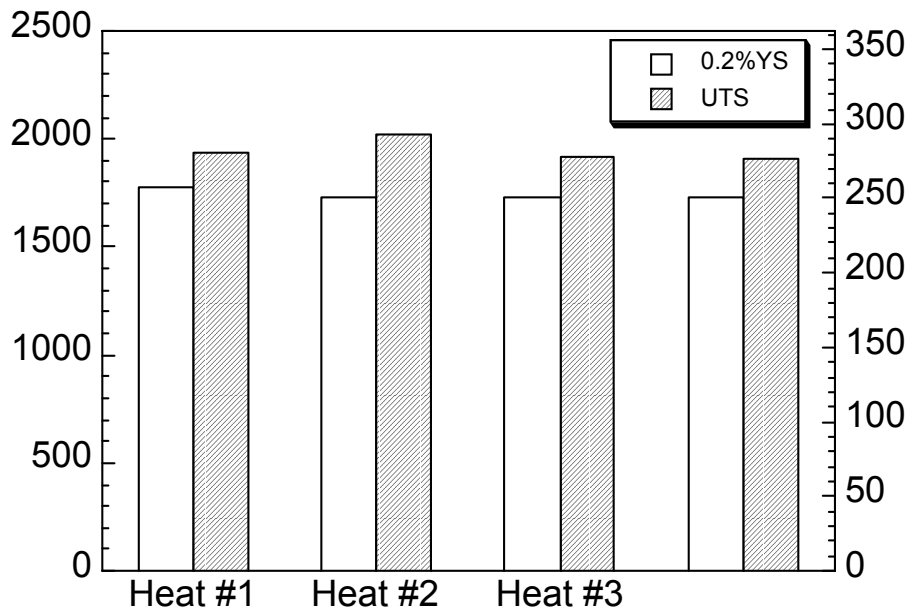
Figure 2.5 0.2% yield strength and ultimate tensile strength of AerMet 100 among 3 heats
