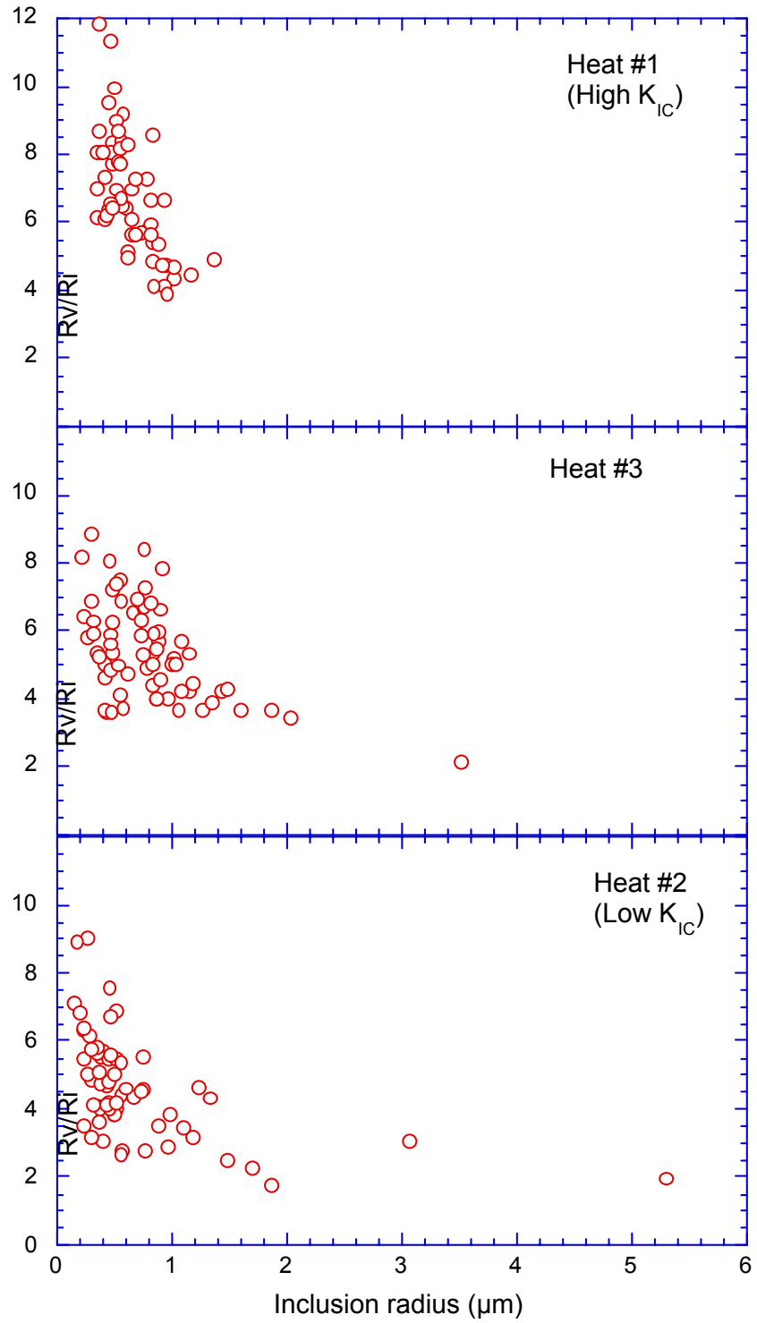
Figure 2.13 Plots of the void growth factor ( R_v/R_i ) as a function of inclusion radius ( R_i )
