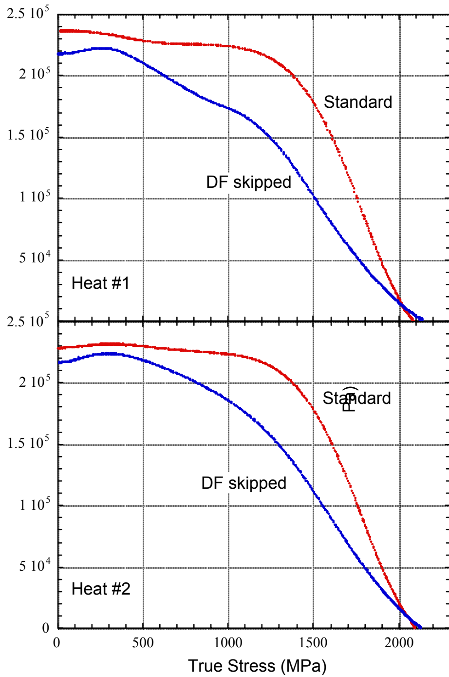
Figure 4.22 Effect of skipping the deep freeze on the work hardening rate – true stress curve.
