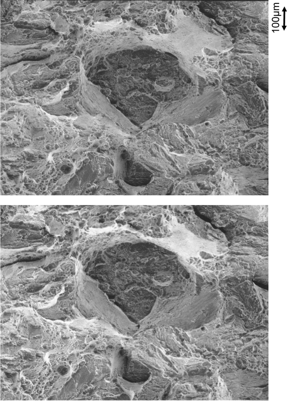
Figure 3.8 A stereo pair of SEM fractographs. Sample: Heat #2, (A) 1100°C, Test temperature: 25°C, CVN impact energy: 9.9J.
