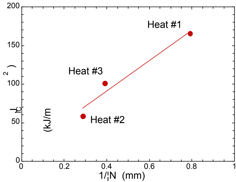
Figure 2.10 Effect of areal inclusion spacing on the fracture toughness. Minimum resolvable particle diameter \approx 2\mu\text{m} .
