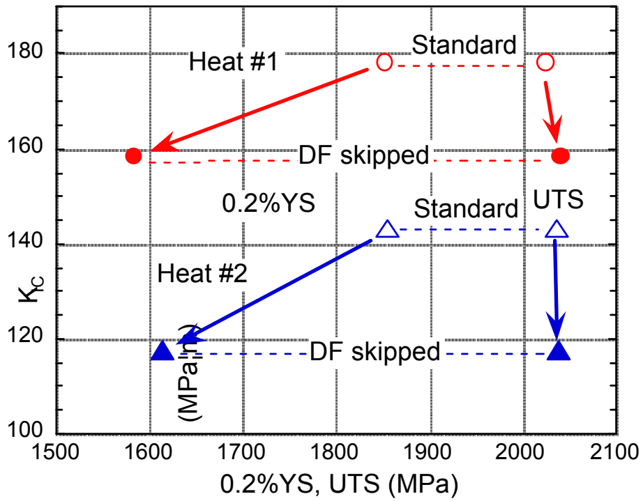
Figure 4.21 Effect of skipping the deep freeze treatment on the toughness-strength relationship.
