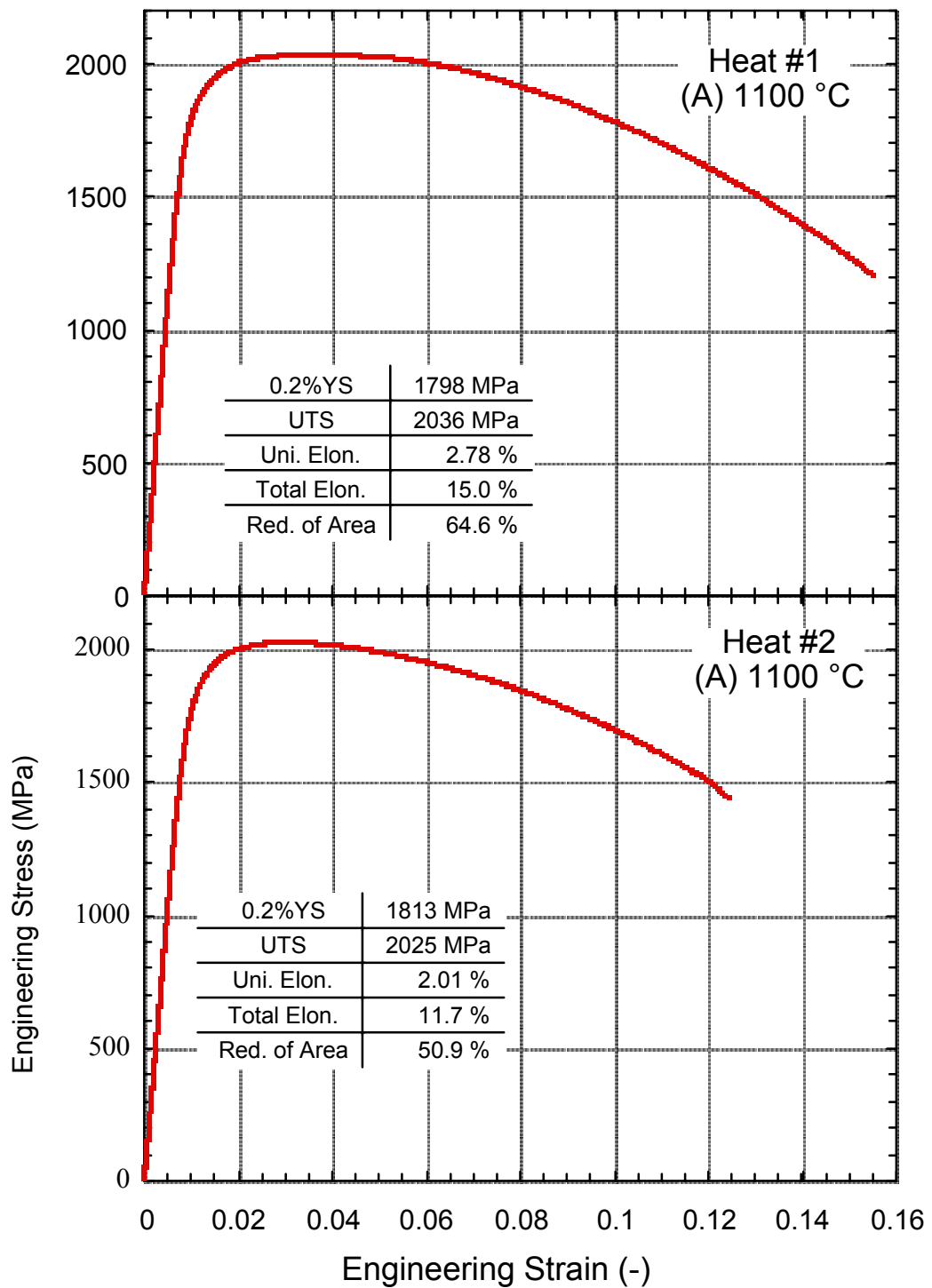
Figure A1 Effect of high temperature austenitization on the engineering stress – engineering strain curve Heat treatment: (A) 1100°C x 1hr, OQ +(DF)-197°C x 1h + (Ag) 482°C x 5h, OQ
