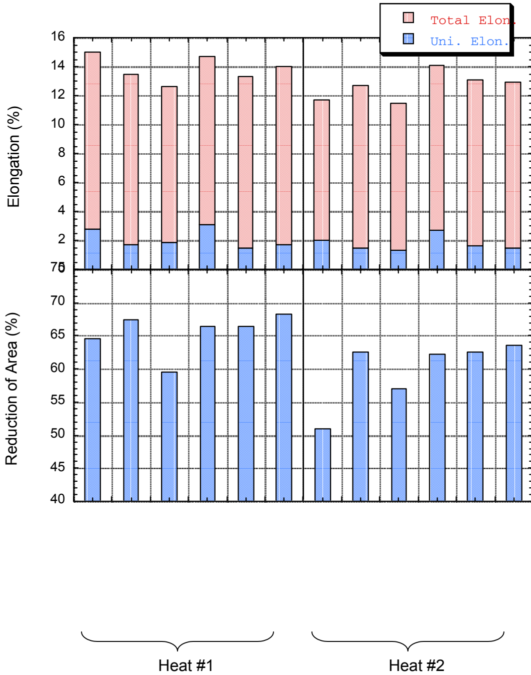
Figure 4.4 Effect of heat treatment conditions on the elongations and the reduction of area.
