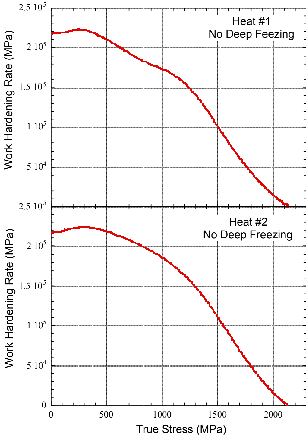
Figure A10 Effect of skipping the deep freeze on the work hardening rate – true stress curve Heat Treatment: (A) 885°C x 1hr, OQ + (Ag) 482°C x 5h, OQ
