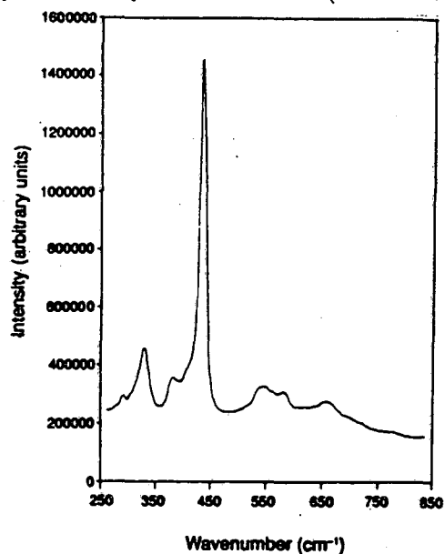
Figure 2. Raman spectrum of ZnO powder. (XBL 898-7278)
