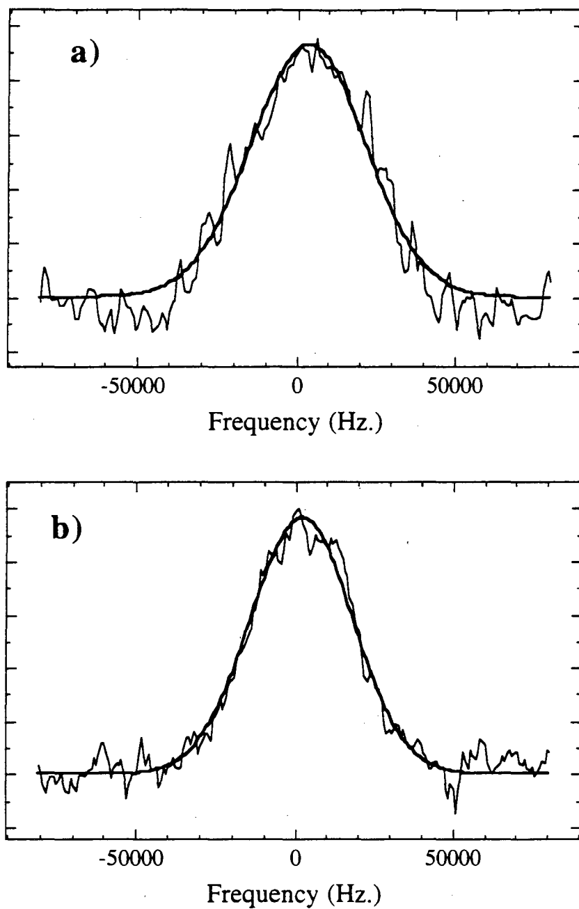
Figure 5.6 Proton spectra of poly(triarylcarbinol) obtained with (a) T_{CP}=200 \mu s (8 contacts) and (b) T_{CP}=20 ms (1 contact).
