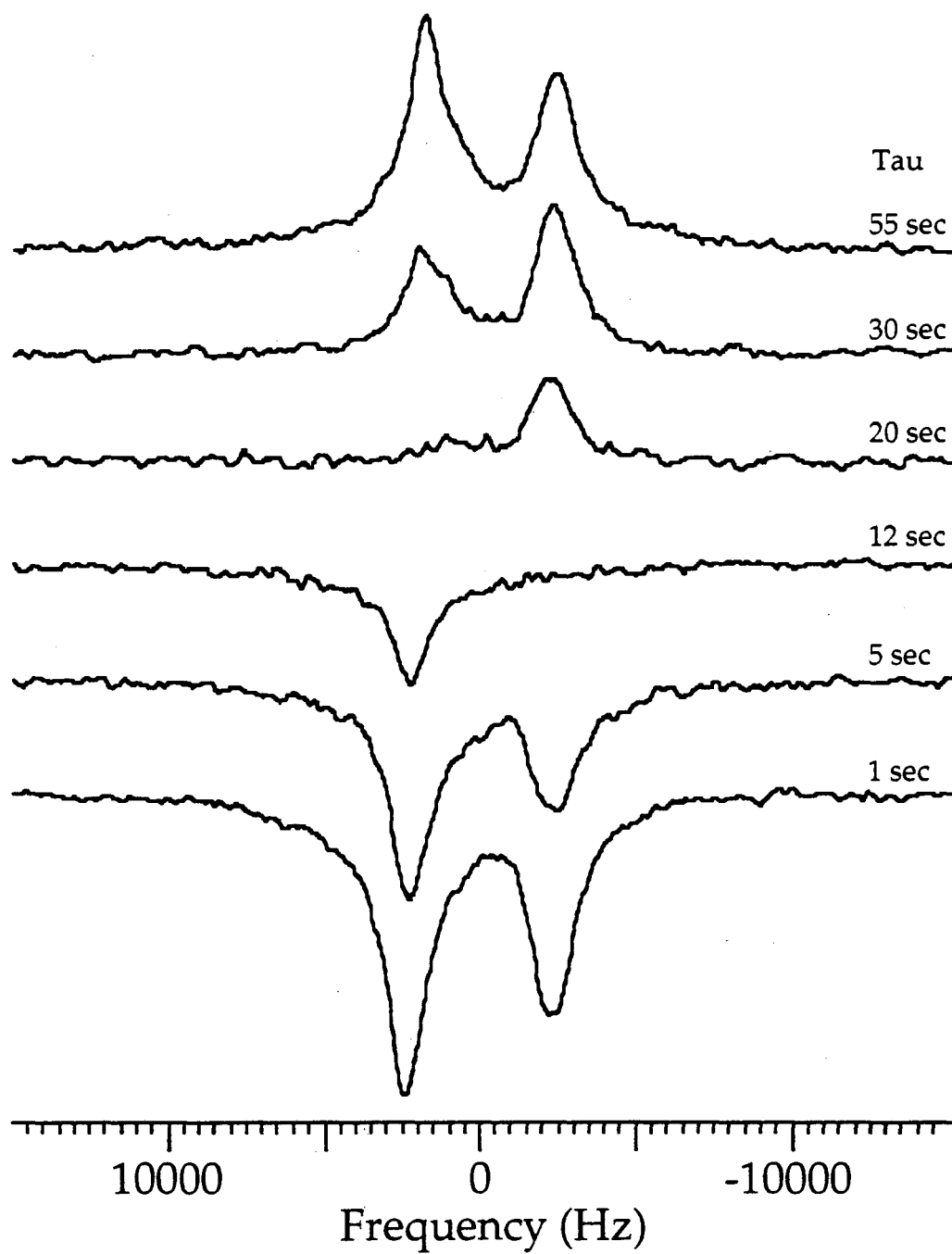
Figure 4.14 Representative spectra of inversion-recovery xenon T_1 measurement in WCB at -168^\circ\text{C} .
