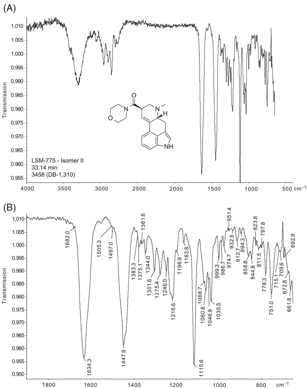
FIGURE 3. GC-solid state-IR spectrum of LSM-775. Top: Entire scan range. Bottom: Partial scan range
