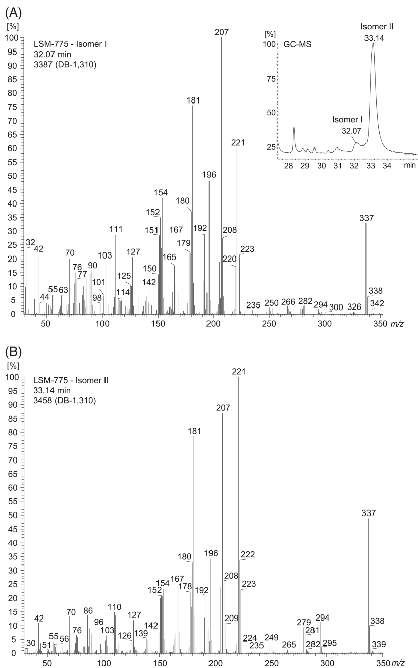
FIGURE 2. Electron ionization mass spectrum, gas chromatography retention time and Kovats retention index recorded for LSM-775 and its minor isomer
