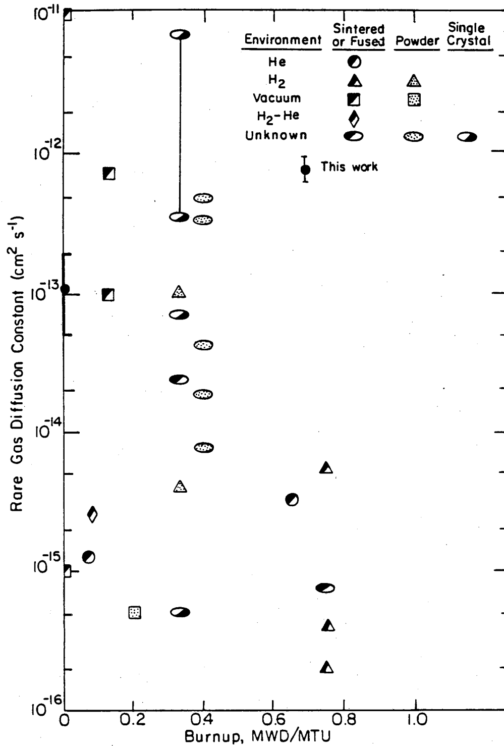
Fig. 7. Diffusion coefficient of xenon in \text{UO}_2 at 1400^\circ\text{C} . References for the various experiments summarized here are given by Lawrence [1].
