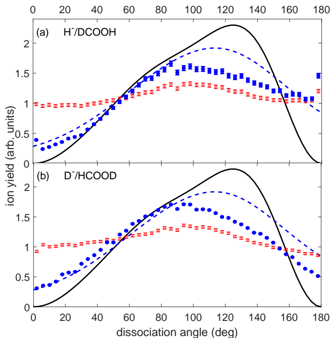
FIG. 10. (Color online) Measured (red open circles) and computed (black curve) ion angular distributions from lowest {}^2A'' Feshbach resonance: H^- from DCOOH (a) and D^- from HCOOD (b). The incident electron energy is 8.45 eV. Theoretical results computed from 2a''(\sigma^*)^2, {}^2A'' entrance amplitude at equilibrium geometry, and the experimental data are normalized to the theory. The blue dashed curve shown in both (a) and (b) is a Gaussian convolution ( 60^\circ full width at half maximum) of the calculated angular distribution to approximate the dissociation dynamics. The blue filled circles are the measured ion angular distribution after subtraction of 50% of the ion yield from the {}^2A' resonance (measured at 7.25 eV; see Figs 6(b) and 7(b)). Error bars show 1 standard deviation in the statistical uncertainty, and the experimental data are normalized to the theory.
