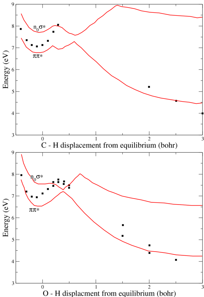
FIG. 2. (Color online) Lowest {}^3A' electronically excited states of neutral formic acid (solid curves) and n_0(\sigma^*)^2 , {}^2A' Feshbach resonance (squares) as a function of C-H and O-H displacement from equilibrium. The parent triplets have conical intersections, but the resonance can be followed to H^- + HOCO for CH and H^- + HCOO for OH dissociation.
