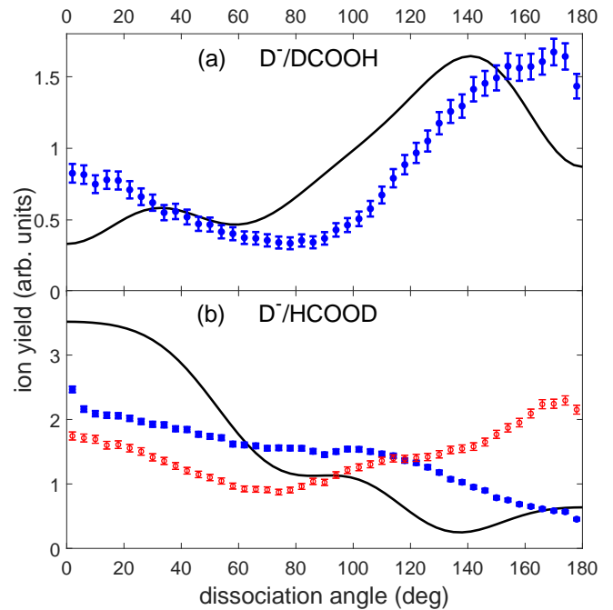
FIG. 7. (Color online) Same as Fig. 6, but for \text{D}^- ions from (a) DCOOH and (b) HCOOD. In panel (b), the blue filled circles are \text{D}^- ions with low kinetic energy (0.5 to 2 eV) and the red open circles are \text{D}^- ions with high kinetic energy (2.7 to 5 eV).
