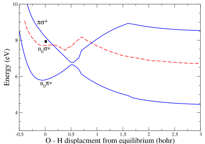
FIG. 5. (Color online) Lowest {}^3A'' electronically excited states of neutral formic acid (solid curves); the 2a''(\sigma^*)^2, {}^2A'' Feshbach resonance (square) is also plotted at equilibrium geometry. The {}^3A' excited state (dashed line) is from Fig. 2b.
