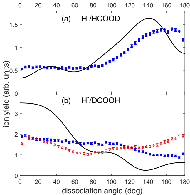
FIG. 6. (Color online) Measured and computed \text{H}^- ion angular distributions from lowest {}^2\text{A}' Feshbach resonance, for (a) HCOOD and (b) DCOOH. The incident energy is 7.25 eV and the theoretical results computed from entrance amplitude at equilibrium geometry. In panel (b), the blue filled circles are \text{H}^- ions with low kinetic energy (1.5 to 3 eV) and the red open circles are \text{H}^- ions with high kinetic energy (3 to 5 eV). Error bars show 1 standard deviation in the statistical uncertainty, and the experimental data are normalized to the theory.
