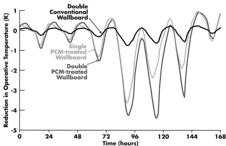
Figure. Reduction in operative temperature for double conventional and single and double PCM-treated wallboard, compared with single conventional wallboard.
