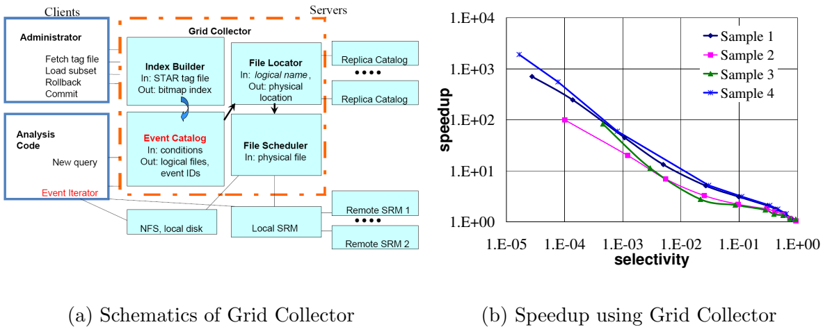
Figure 5: Using Grid Collector can significantly speed up analysis of STAR data (Timing measurements collected on a cluster with 2.8 GHz Intel Xeon processors [32, 42]).
