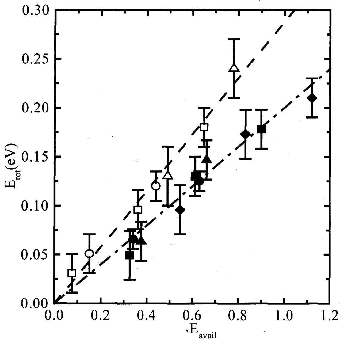
Figure 8. Plot of the photofragment rotational energy, E_{\text{rot}} as a function of the energy available to translation, E_{\text{avail}} . The results of the impulsive model calculation for HNCN and DNCN are indicated by a dot-dash and dashed line respectively. The experimental values for E_{\text{rot}} from the experimental P(E_{\text{T}}) distributions are shown as closed symbols for HNCN and open symbols for DNCN with photon energies of 3.6 eV ( \circ ), 3.9 eV ( \square ), 4.03 eV ( \triangle ) and 4.16 eV ( \diamond ). The effective barrier heights for each transition, E'_{\text{barrier}} are estimated by determining the intercept value required to place the experimental data on the line of the impulsive model calculations, see text.
