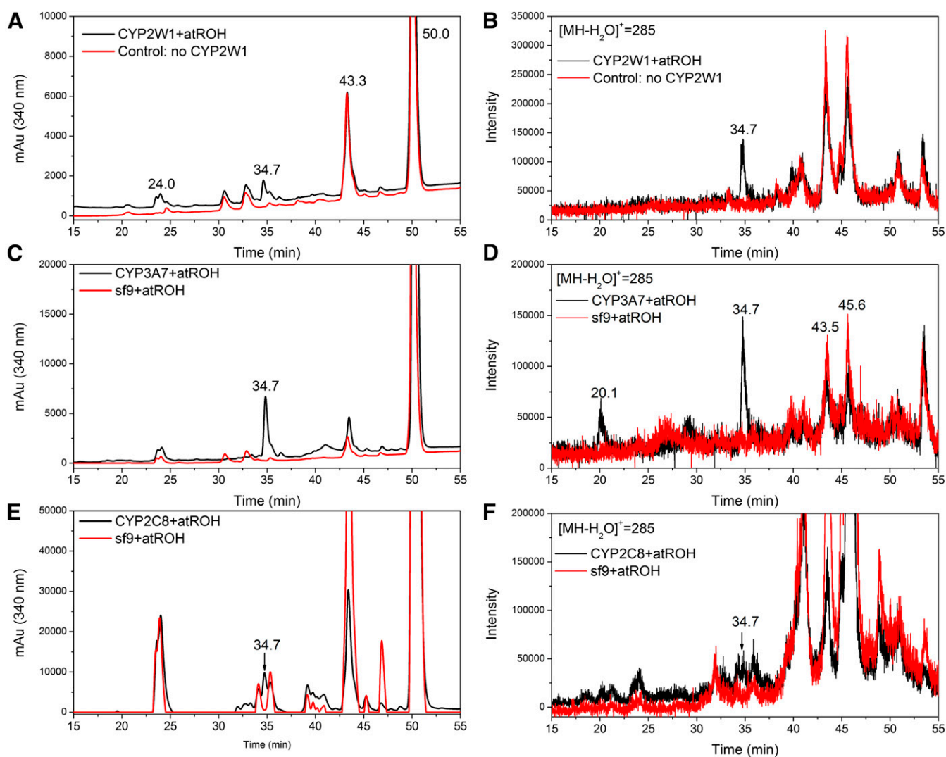
Fig. 6. LC-MS analysis of CYP2W1, CYP3A7, and CYP2C8, all- trans retinol metabolites. In the plots, the red trace is from a control incubation without a P450 enzyme, and the black trace is from the complete incubation with the indicated P450 enzyme. (A) LC chromatogram with the detector at 340 nm and (B) extracted ion ( m/z = 285 ) chromatogram in positive ES mode of all- trans retinol metabolites generated by incubation with and without CYP2W1 enzyme; (C) LC chromatogram with the detector at 340 nm and (D) extracted ion ( m/z = 285 ) chromatogram of all- trans retinol metabolites generated by incubation with and without baculovirus-insect cell microsomes expressing CYP3A7 and cytochrome b_5 supplemented with recombinant CPR; (E) LC chromatogram with the detector at 340 nm; and (F) extracted ion ( m/z = 285 ) chromatogram of all- trans retinol metabolites generated by incubation with and without baculovirus-insect cell microsomes expressing CYP2C8 and cytochrome b_5 supplemented with recombinant CPR.
