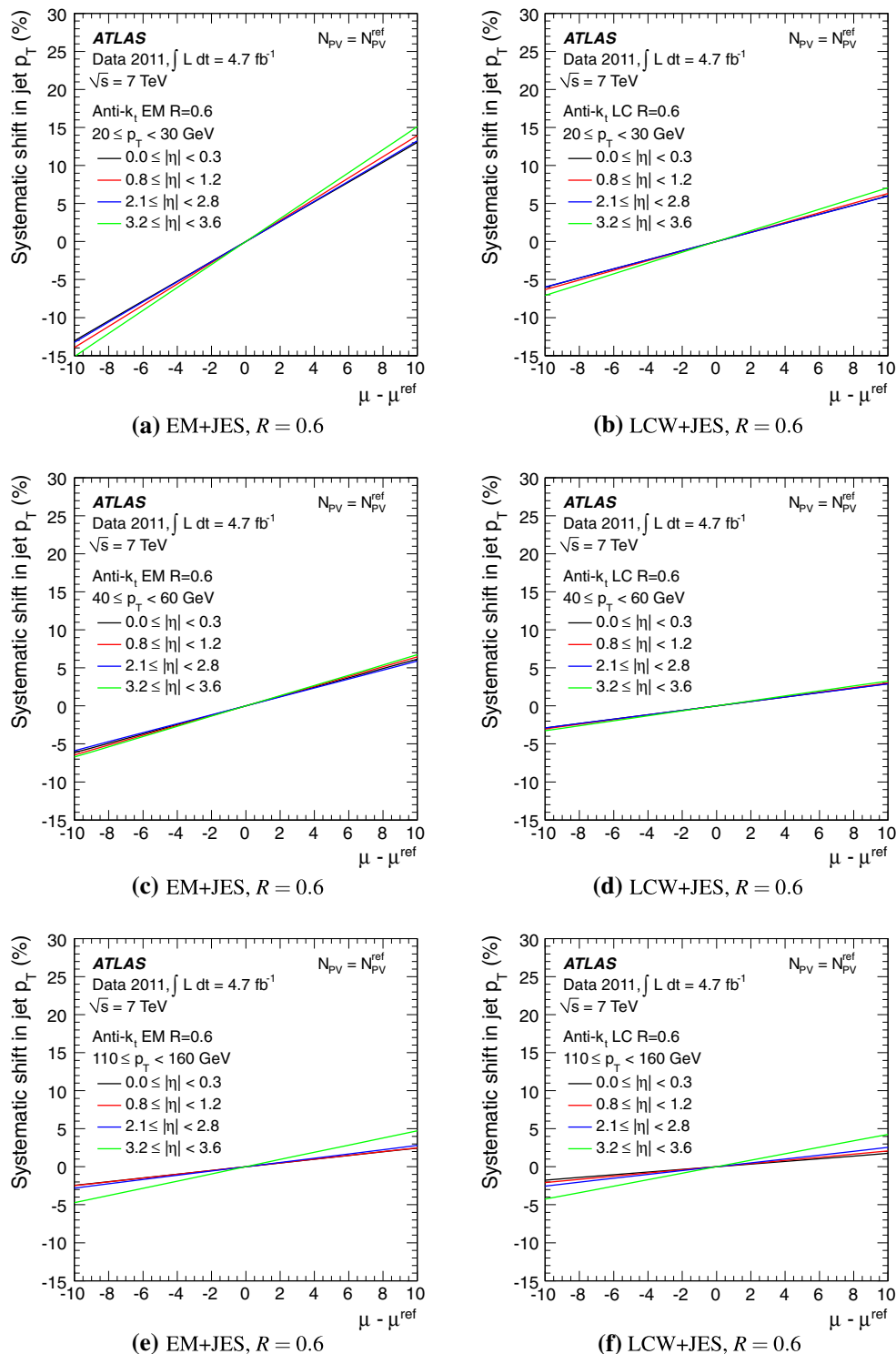
Fig. 49 The fractional systematic shift due to mis-modelling of the effect of out-of-time pile-up on the transverse momentum p_{T,EM+JES}^{jet} of jets reconstructed with the anti- k_t algorithm with R = 0.6 and calibrated with the EM+JES scheme, is shown as a function of (\mu - \mu^{ref})
