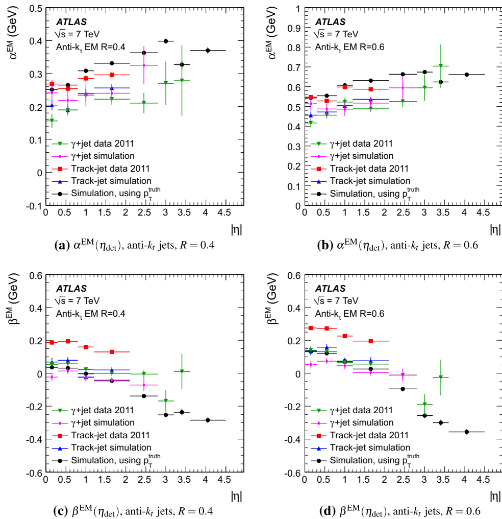
Fig. 8 The pile-up contribution per additional vertex, measured as \alpha^{\text{EM}} = \partial p_{T,EM}^{\text{jet}} / \partial N_{PV} , as function of |\eta_{\text{det}}| , for the various methods discussed in the text, for a R = 0.4 and b R = 0.6 jets. The contribution from \mu , calculated as \beta^{\text{EM}} = \partial p_{T,EM}^{\text{jet}} / \partial \mu and displayed for the various
