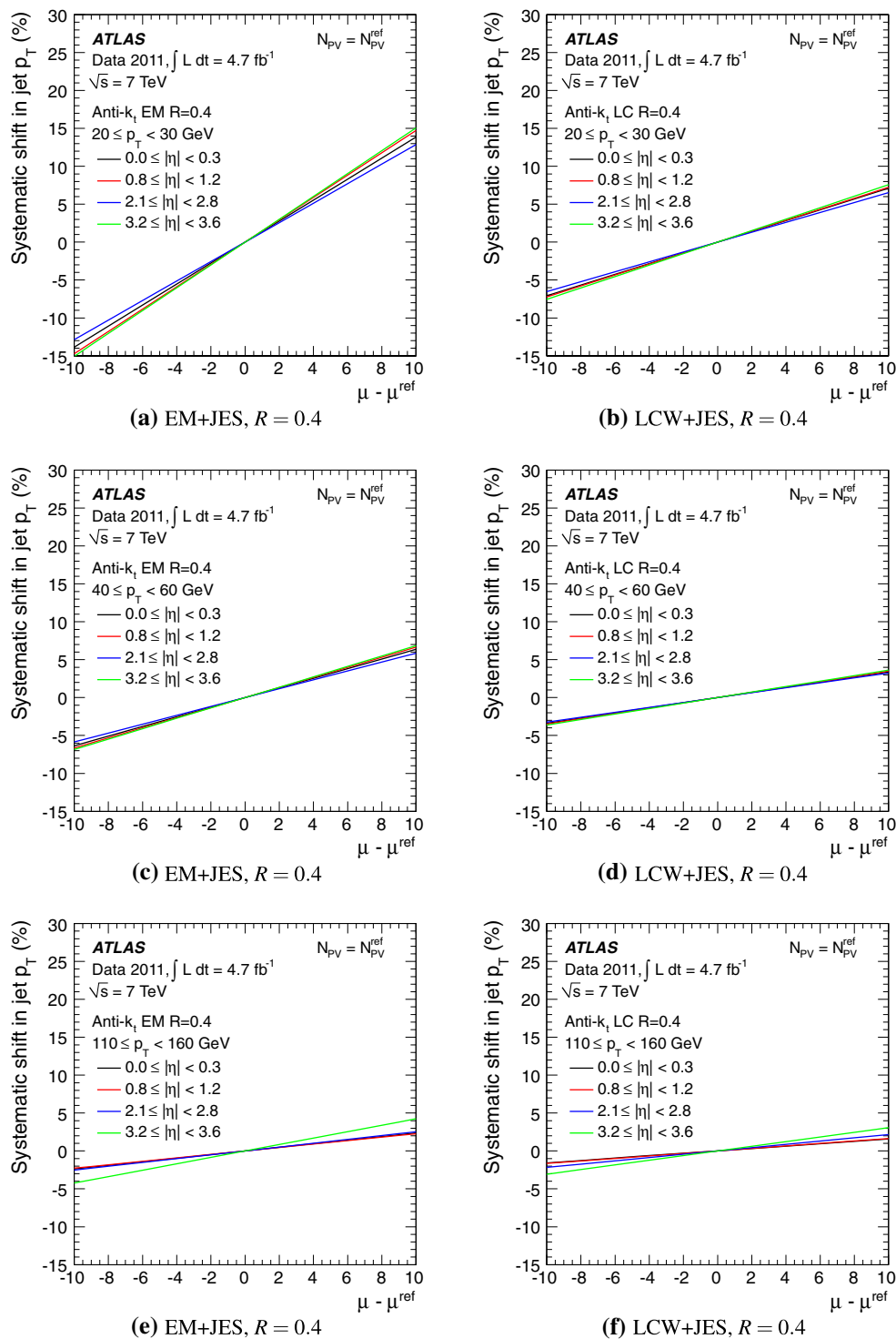
Fig. 48 The fractional systematic shift due to mis-modelling of the effect of out-of-time pile-up on the transverse momentum p_{T,EM+JES}^{jet} of jets reconstructed with the anti- k_r algorithm with R = 0.4 and calibrated with the EM+JES scheme, is shown as a function of (\mu - \mu^{ref})
