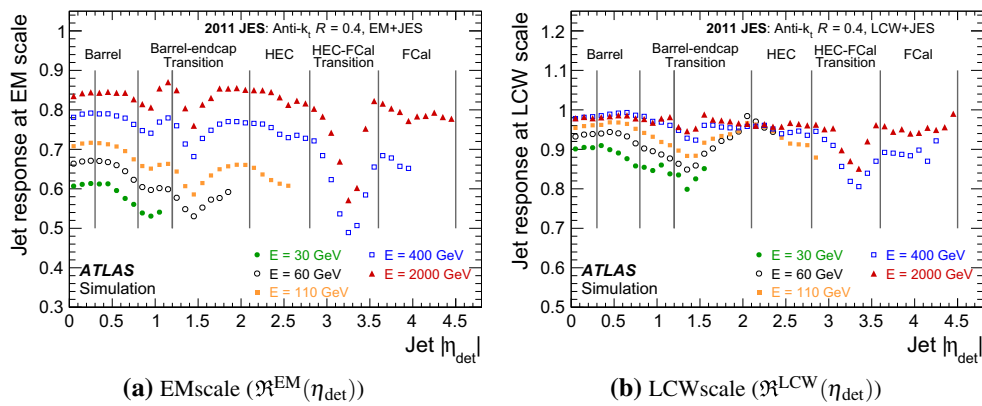
Fig. 4 Average response of simulated jets formed from topo-clusters, calculated as defined in Eq. (1) and shown in a for the EM scale ( \mathcal{R}^{EM} ) and in b for the LCW scale ( \mathcal{R}^{LCW} ). The response is shown separately for various truth-jet energies as function of the uncorrected (detector) jet
