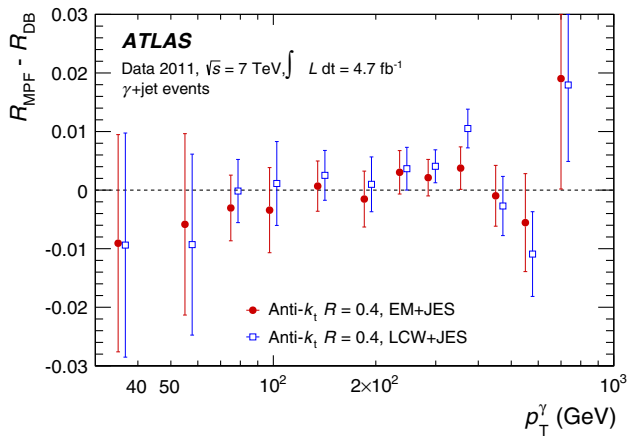
Fig. 39 Difference between the data-to-MC response ratio R measured using the direct balance (DB) and the missing momentum fraction (MPF) methods for jets reconstructed with the anti- k_r algorithm with R = 0.4 calibrated with the EM+JES and LCW+JES schemes. The error bars shown only contain the uncorrelated uncertainties
