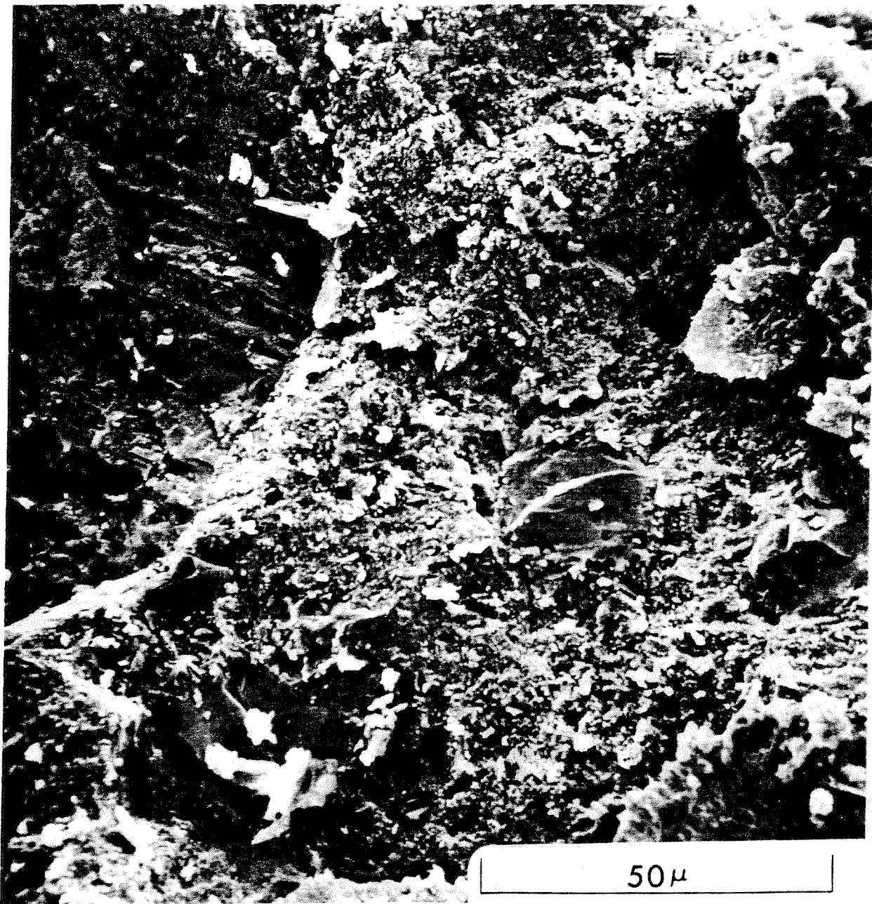
Figure 4.10 (continued from opposite page)... (b) A micrograph of an area marked in (a) which shows the fracture surface of several sand grains. The presence of the broken sand grains means that the cement paste is sound. (Please note that 1\mu corresponds to 10^{-4} cm or approximately 4 \times 10^{-5} in.)
