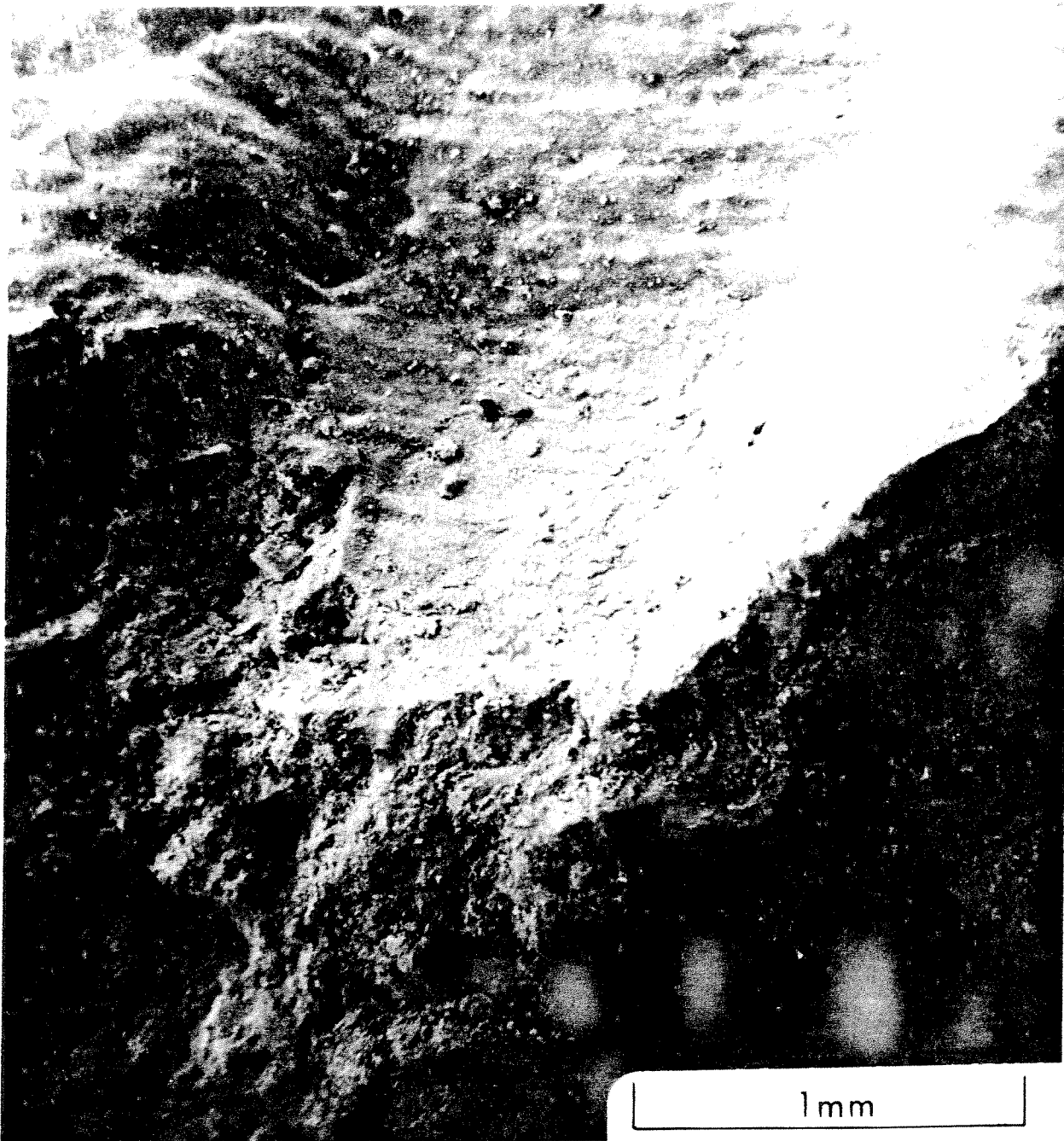
Figure 4.11 (a) A low magnification micrograph showing the surface of the mortar with \text{CrO}_3 is smooth and unmarked by bubbles. Notice that there are not any bubbles on the fracture surface through the mortar in the foreground.
