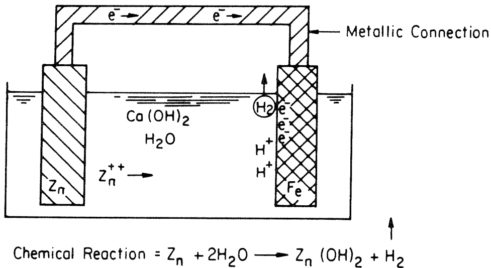
Figure 3.1. Schematic representation of a zinc-iron galvanic cell.
