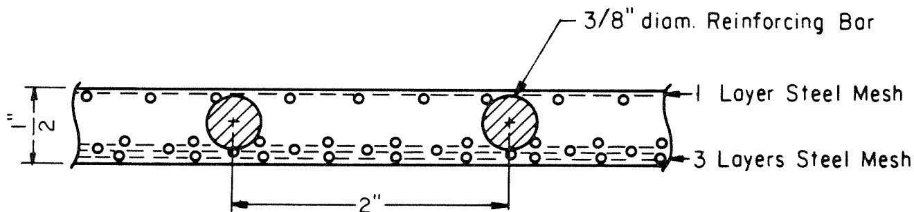
Figure 4.2. \frac{1}{2} -in ferro-cement visual inspection specimen (cross section), scale 1:1.
