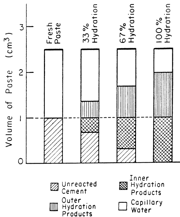
Figure 2.1. Graphical representation of the relative volumes of hydration products of portland cement at three stages of hydration: 33%, 67%, and 100% completion. The initial water-to-cement ratio is 0.5, and one unit volume of cement is shown to produce two unit volumes of hydration products.
