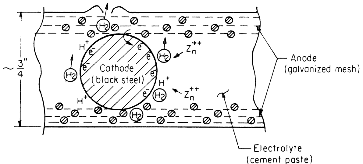
Figure 3.2. A cross section of ferro-cement schematically showing the galvanic cell between galvanized mesh and black steel reinforcing bar.
