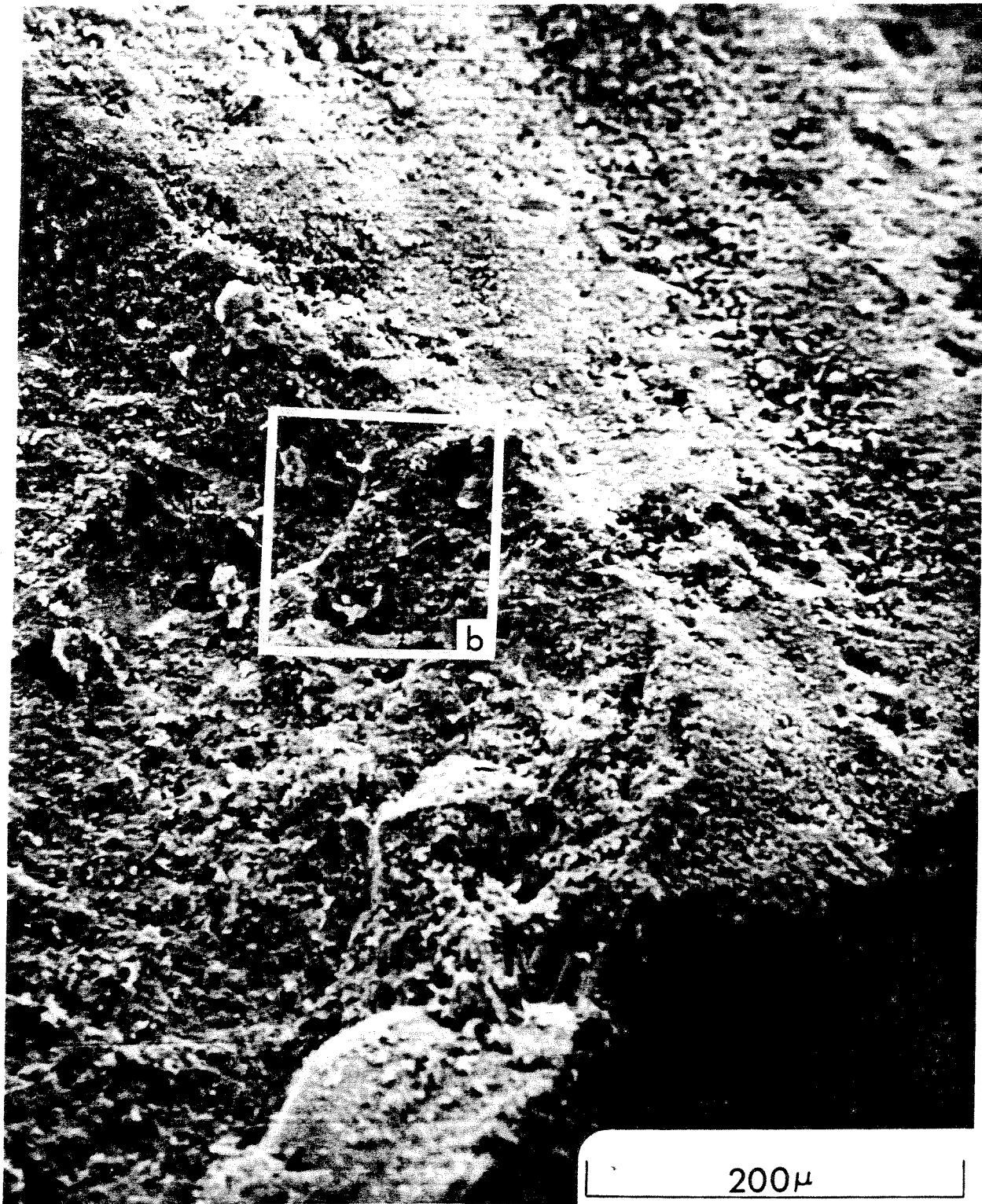
Figure 4.10 (a) A higher magnification micrograph of a region just to the left of the arrow in Figure 4.9. The surface of the mortar that was in contact with the steel is in the upper right hand side of this micrograph.
