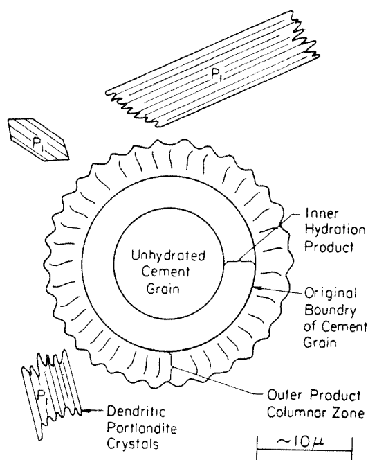
Figure 2.2. The hydration products formed inside and outside the cement grain are schematically represented. The multiple nature of the cement grain is neglected and is assumed to be a single phase that shows two types of hydration products.
