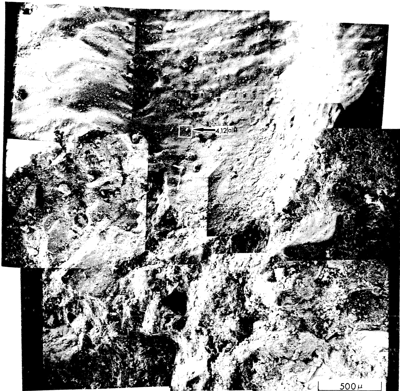
Figure 4.11 (continued from opposite page)... (b) A mosaic of micrographs showing approximately the same region as in (a) but with more detail. Notice the smoothness of the mortar with \text{CrO}_3 .
