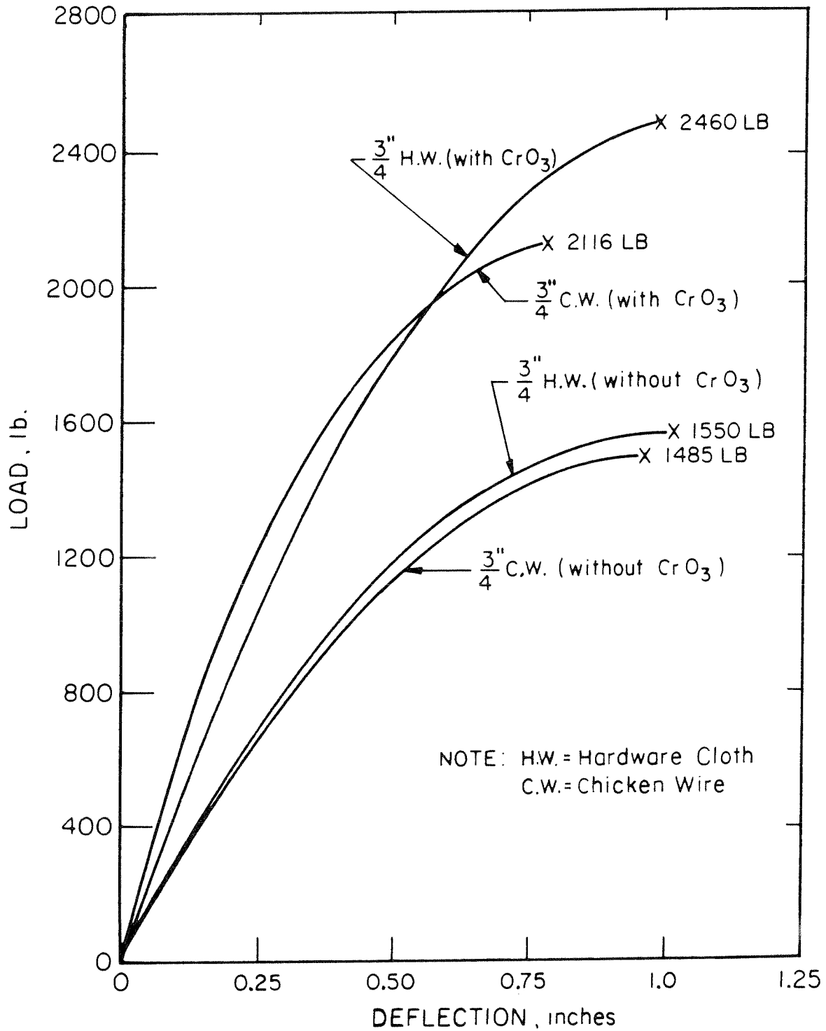
Figure 4.7. The load-deflection curve for the flexure tests of specimens with and without \text{CrO}_3 . The specimens with \text{CrO}_3 show substantially greater stiffness as well as ultimate strength.
