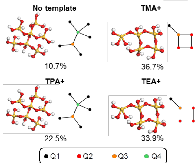
Figure 3. Predominant chemical species calculated in kMC calculations identified as \text{Q}^1 , \text{Q}^2 , \text{Q}^3 and \text{Q}^4 .
