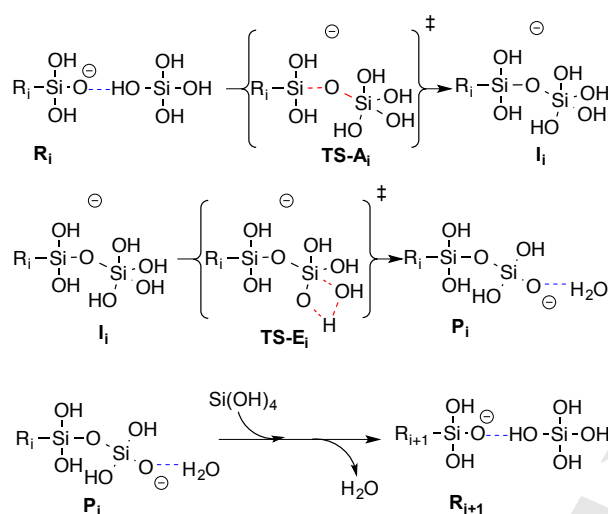
Scheme 1. Anionic concerted mechanism in basic conditions proposed for the formation of linear oligomers. The reactive complex ( \mathbf{R}_i ) formed of the anionic oligomer and an \text{Si}(\text{OH})_4 monomer undergoes an addition reaction ( \text{TS-A}_i ) yielding a five-coordinated intermediate ( \mathbf{I}_i ). The elimination of water ( \text{TS-E}_i ) allows the formation of a hydrated complex ( \mathbf{P}_i ). The exchange of the water molecule with a monomer results in the reactant complex \mathbf{R}_{i+1} . (see also the mechanisms for cyclic and branched oligomers in Schemes S1 and S2 , respectively). TS stands for transition state.
