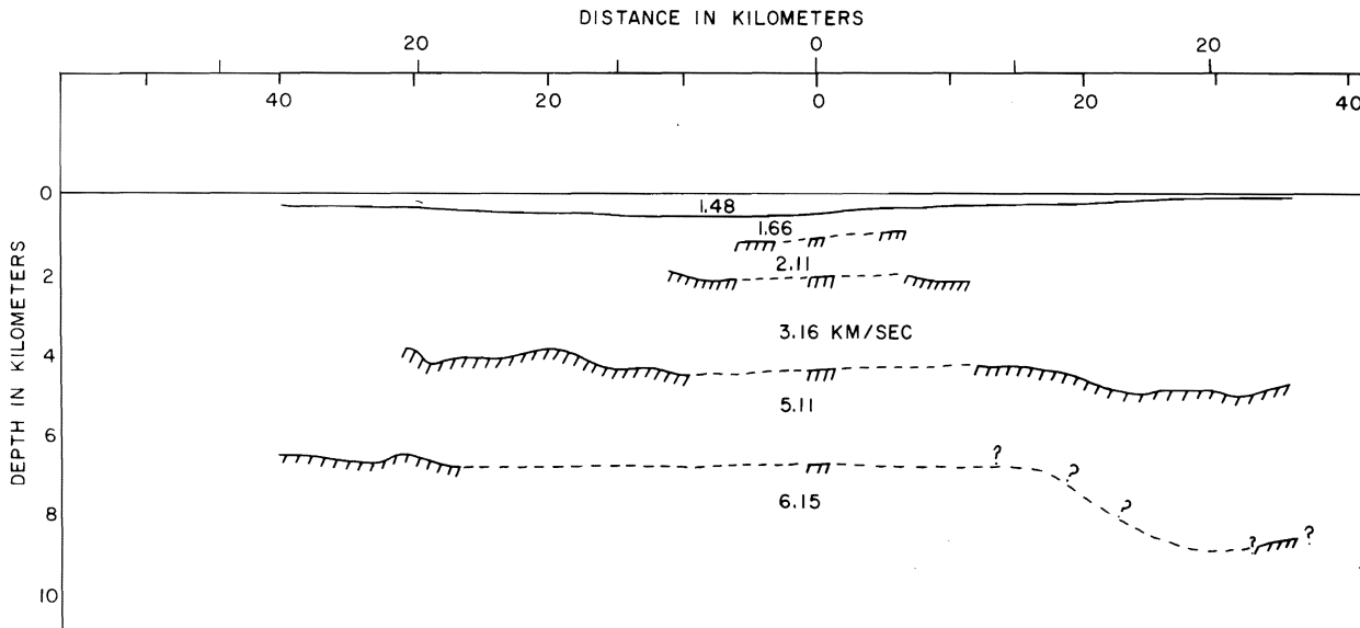
Fig. 99. Structural section, ARGUELLO, Station 6, 21 March 1957
