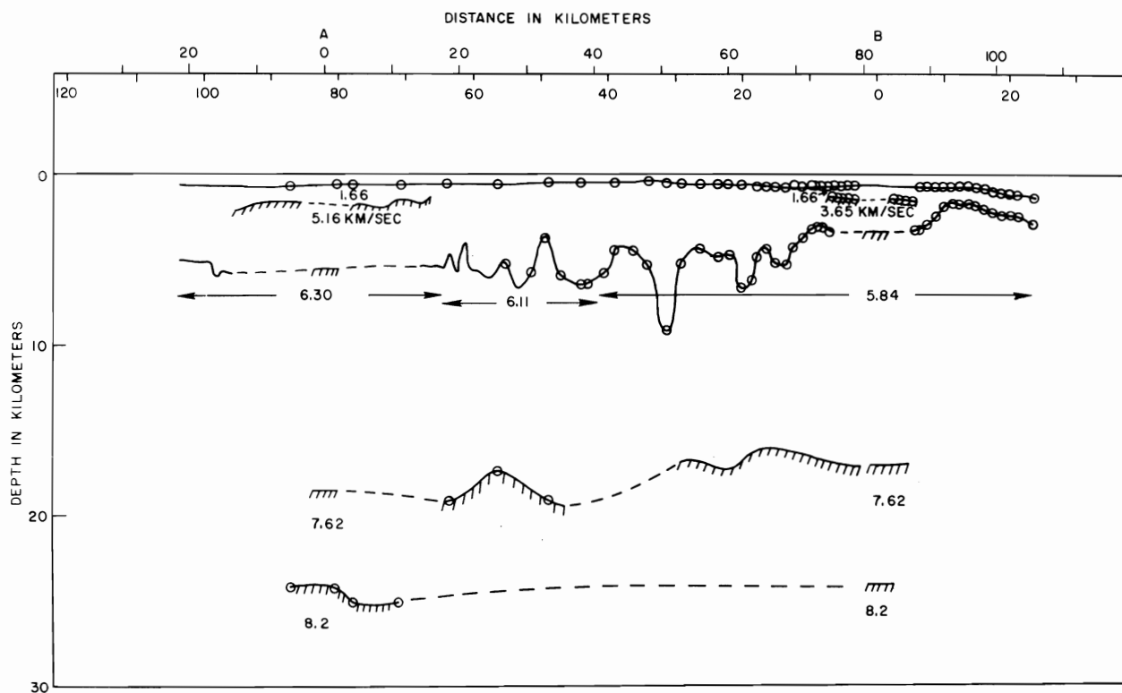
Fig. 94. Structural section, ARGUELLO, Stations 4 and 5, 19 and 20 March 1957
