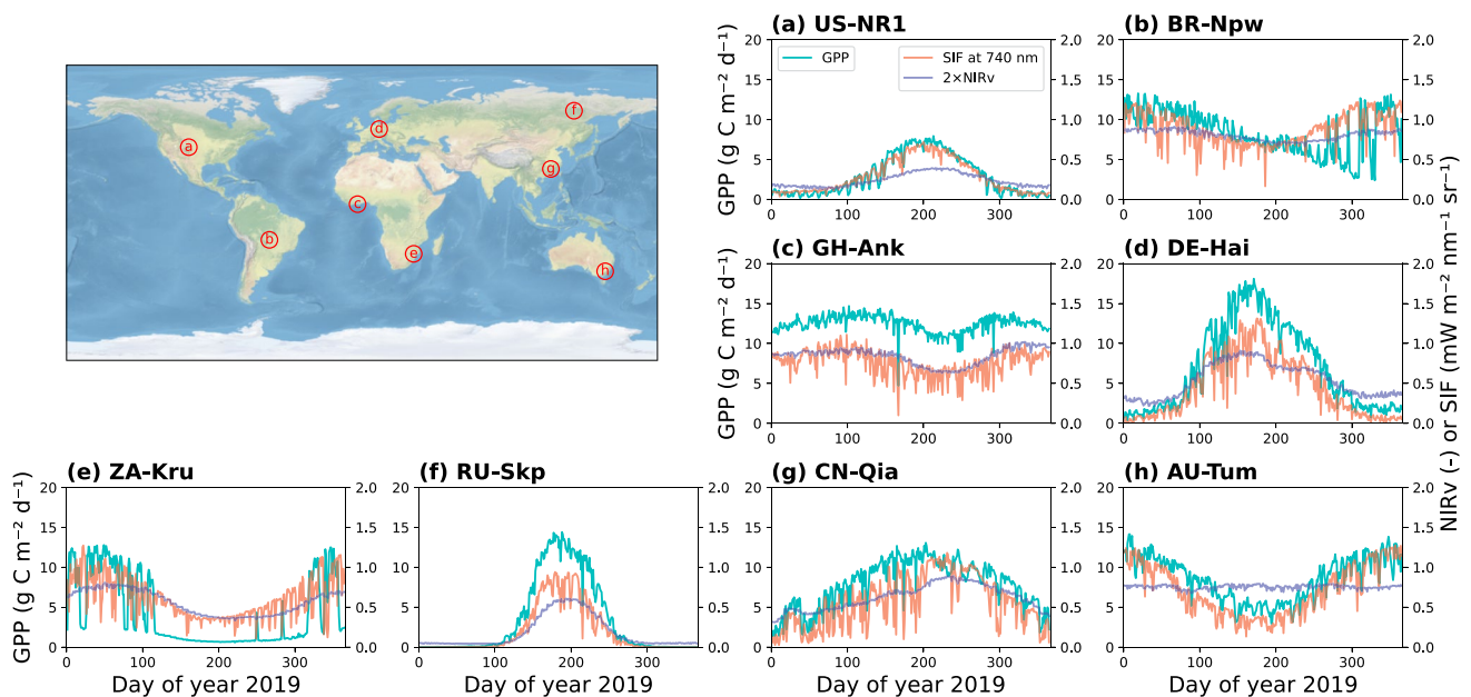
Figure 2. Examples of Climate Modeling Alliance (CliMA) Land run at eight 1° grid cells across the globe. CliMA Land global run was made for year 2019. The (latitude, longitude) centers are (a) (40.5°, -105.5°), (b) (-16.5°, -56.5°), (c) (5.5°, -2.5°), (d) (51.5°, 10.5°), (e) (-25.5°, 31.5°), (f) (62.5°, 129.5°), (g) (26.5°, 115.5°), and (h) (-35.5°, 148.5°), respectively. There is a flux tower within each example grid cell, and they are US-NR1, BR-Npw, GH-Ank, DE-Hai, ZA-Kru, RU-Skp, CN-Qia, and AU-Tum, respectively. The cyan curve plots the modeled daily cumulative gross primary productivity; the red curve plots the modeled daily mean solar-induced chlorophyll fluorescence at 740 nm; the blue curve plots the modeled daytime mean near infrared reflectance of vegetation (NIRv). NIRv is scaled to 2 times the original value to facilitate visualization.
