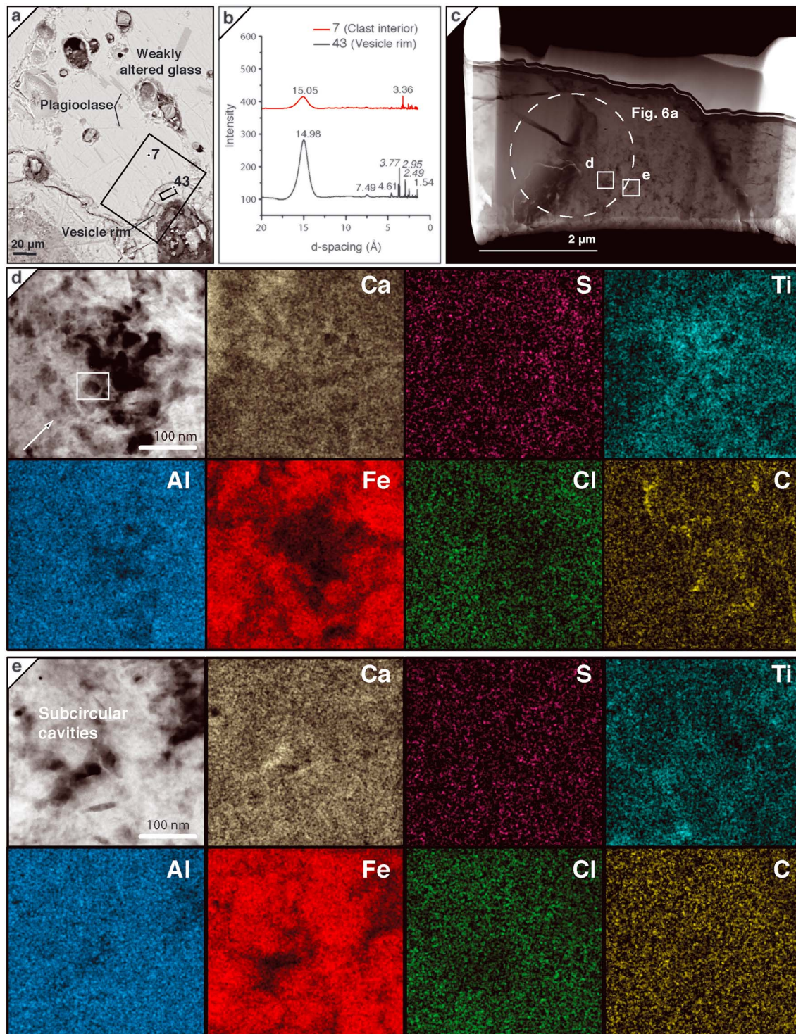
Figure 5. Basaltic lapillus, 137.9-m depth, showing investigations of altered glass. (a) Scanning electron microscopy-backscattered electron image, sites of X-ray microdiffraction( \mu XRD) analyses and focused ion beam (FIB) lift out. (b) Intensity versus d spacing plot for \mu XRD analyses (#7 [red] and #43 [black]), including plagioclase [shown in italics ]. (c) FIB lift out, site of Raman spectra (Figure 7a). (d) Scanning transmission electron microscopy-energy dispersive X-ray spectrometer (S/TEM EDS) elemental maps, white rectangle indicates a subcircular cavity along the left edge of the vesicle and very fine nanoscale cavities nearby (arrow). (e) S/TEM EDS elemental maps, area of larger nanoscale subcircular cavities.
