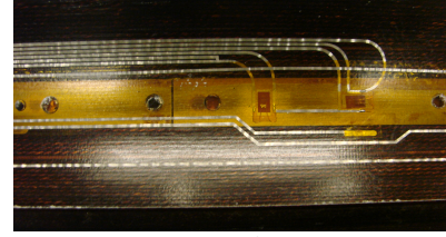
Fig. 8. TQ inner layer traces - connection of the traces to the strain gages
