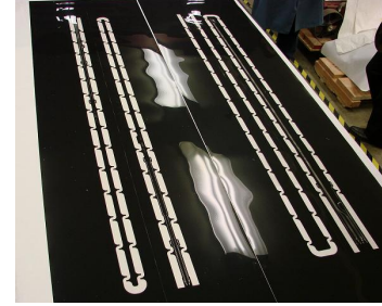
Fig. 5. Artwork of LQ layer 1 and layer 2 traces
