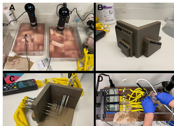
Fig. 1 Equipment. A Pieces of meat heated in a water bath using heating units (Culinary Sous Vide Precision Cooker Pro, 1200 W, San Francisco, CA). B A stand to hold the cryoneurolysis probe at a 30° angle of approach and nine tapered thermocouple temperature probes at precise 5-mm increments in all three dimensions relative to the end of the cryoprobe. C The stand created with a three-dimensional printer with the temperature probes inserted (Cooper-Atkins 50209-K micro-needle thermocouple type K probe, Cooper-Atkins Corp., Middlefield, CT). D Positioning of the equipment during measurements
