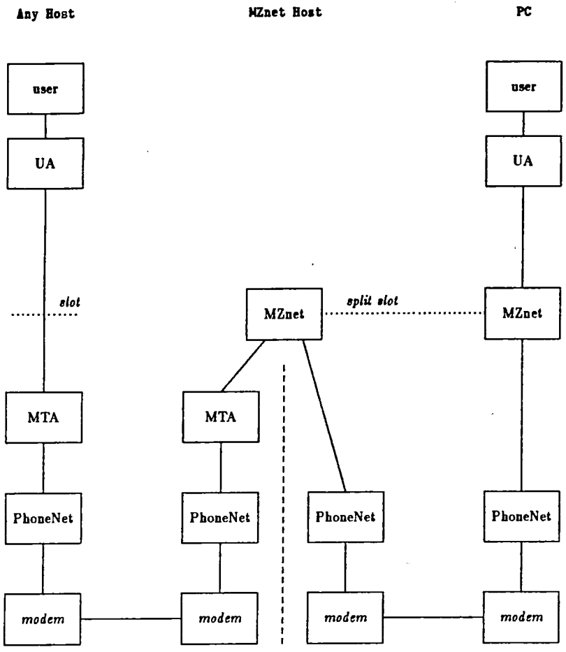
Figure 2. MZnet split-slot arrangement
