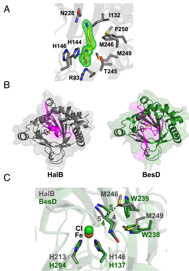
Fig. 3. Structural basis of site-selectivity. (A) Crystal structure of HalB (1.9 Å) with F_{\sigma}-F_c omit map (green mesh, contoured at 1 \sigma ) for lysine (yellow). Active site residues of HalB are shown as gray sticks. (B) Comparison of the overall structures of HalB (1.90 Å, gray) and BesD (1.95 Å, green, PDB 6NIE). The enzymes share high structural similarity except at the substrate covering lid (magenta). (C) Structural alignment of HalB (gray) and BesD (green). Although the carboxylate and amine of lysine are in a similar position in both cases, the sidechain samples a different conformation in the two enzymes. In BesD, C_4 is oriented toward chloride in the active site, while C_5 is oriented away. In contrast, HalB orients C_5 toward chloride. The substrate conformation is influenced by residues in the substrate covering lids of BesD and HalB. In particular, Met246 in HalB makes a steric contribution to the reaction outcome.
