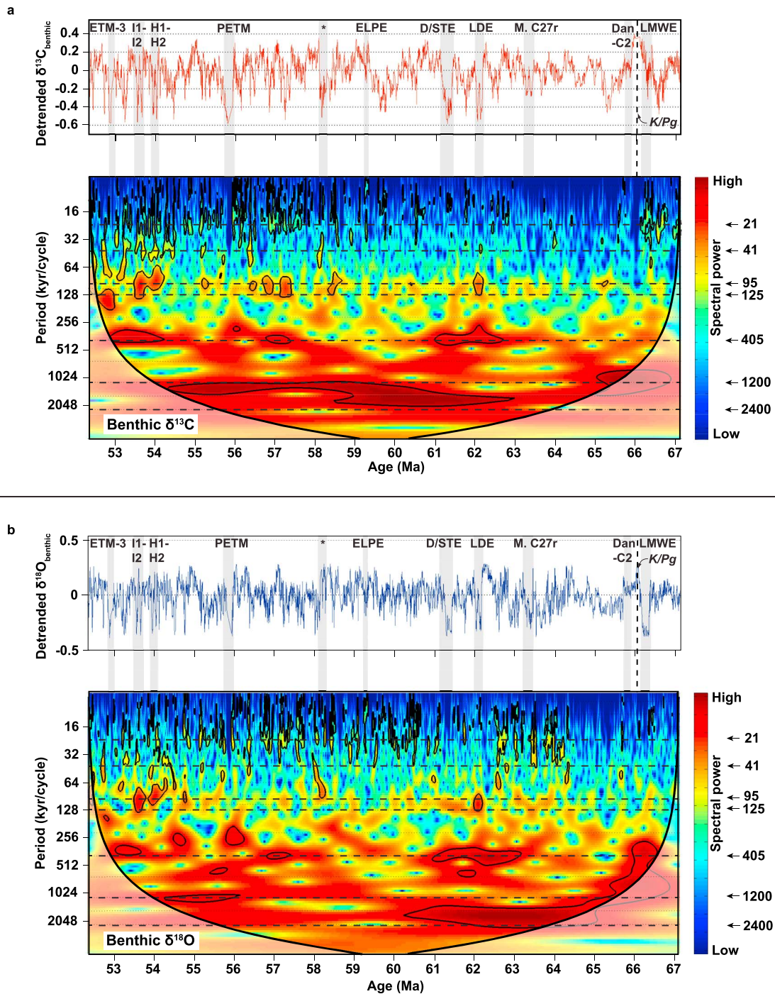
Figure 9. Evolutionary wavelet spectra for the complete Late Maastrichtian–Early Eocene records from Ocean Drilling Program Site 1262. Milankovitch cycles (in kyr) are indicated by dashed lines across the spectra and labeled with arrows along the right-hand margin. (a) \delta^{13}\text{C}_{\text{benthic}} . (b) \delta^{18}\text{O}_{\text{benthic}} . LMWE = Late Maastrichtian warming event; Dan-C2 = Dan-C2 event; M. C27r = Middle Chron 27r event; LDE = Latest Danian Event; D/STE = Danian/Selandian Transition Event; ELPE = Early Late Paleocene Event; PETM = Paleocene-Eocene Thermal Maximum; ETM-3 = Eocene Thermal Maximum 3.
