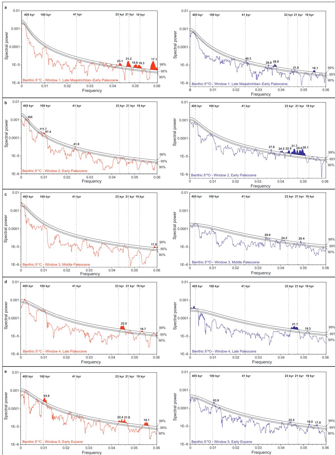
Figure 8. Multitaper Method power spectra for the \delta^{13}\text{C}_{\text{benthic}} record (in red) and \delta^{18}\text{O}_{\text{benthic}} record (in blue) for the five discrete time windows. (a) Window 1, Late Maastrichtian–Early Paleocene (67.1–64.0 Ma). (b) Window 2, Early Paleocene (64.0–61.25 Ma). (c) Window 3, Middle Paleocene (61.25–58.75 Ma). (d) Window 4, Late Paleocene (58.75–55.93 Ma). (e) Window 5, Early Eocene (55.83–52.35 Ma). Temporal distribution of the time windows is illustrated in Figures 2f and 6g.
