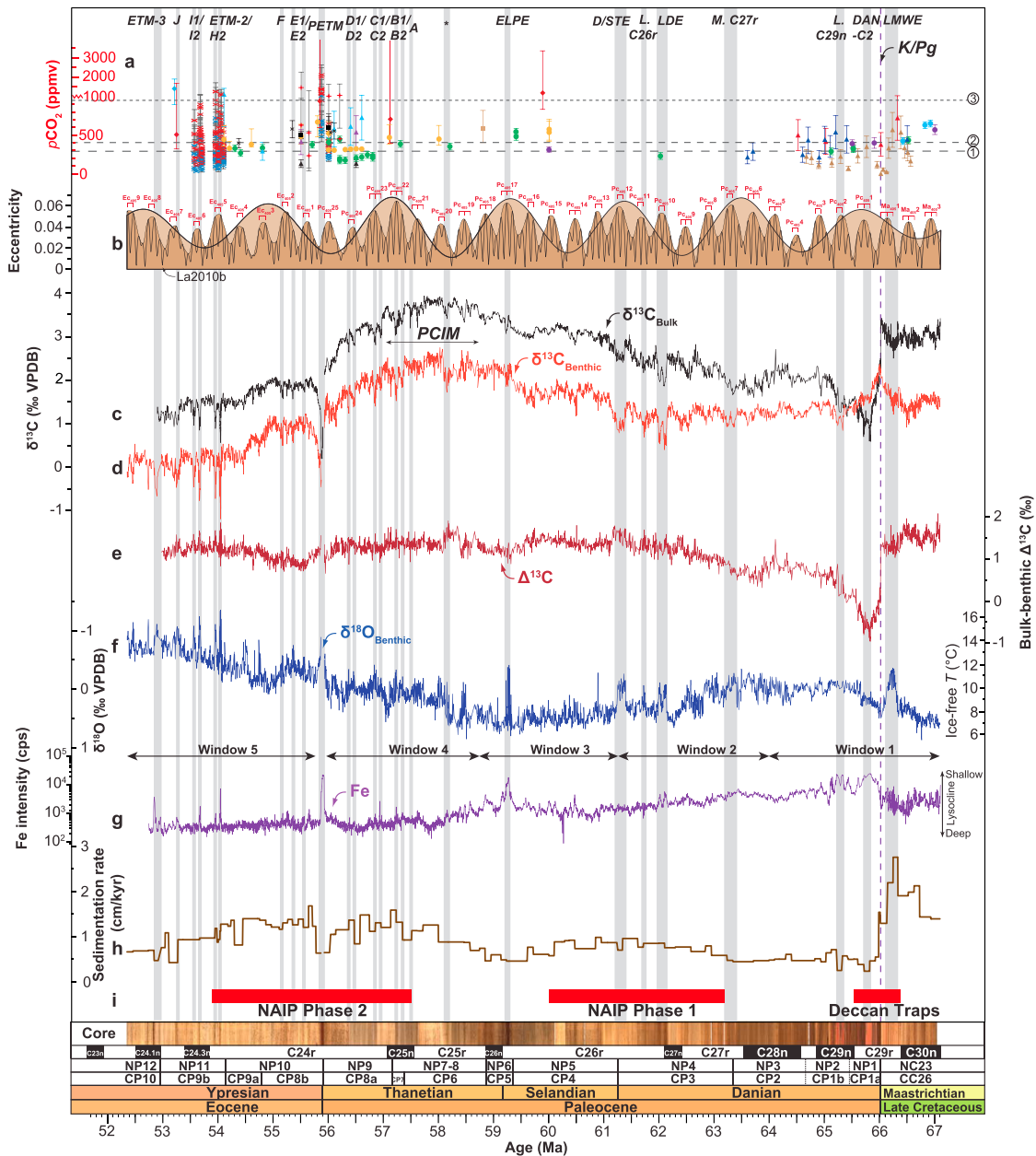
Figure 2. Recalibrated proxies for atmospheric p\text{CO}_2 along with stable carbon and oxygen isotope records and elemental Fe intensities from Ocean Drilling Program Site 1262, calibrated against the updated orbitally tuned age model. Previously described hyperthermals and smaller climatic perturbations are indicated by labeled gray bands, with the following abbreviations: LMWE = Late Maastrichtian warming event; Dan-C2 = Dan-C2 event; L. C29n = Lower Chron 29n event; M. C27r = Middle Chron 27r event; LDE = Latest Danian Event; L. C26r = Lower Chron 26r event; D/STE = Danian/Selandian Transition Event; ELPE = Early Late Paleocene Event; PETM = Paleocene-Eocene Thermal Maximum; ETM-2 = Eocene Thermal Maximum 2; ETM-3 = Eocene Thermal Maximum 3. Core photo from Shipboard Scientific Party (2004). (a) Recalibrated atmospheric p\text{CO}_2 data (Anagnostou et al., 2016; Beerling et al., 2002, 2009; Cui & Schubert, 2016, 2017; Demicco et al., 2003; Fletcher et al., 2008; Gehler et al., 2016; Huang et al., 2013; Koch et al., 1992; Nordt et al., 2002, 2003; Royer, 2003, 2006, 2014; Royer, Berner, et al., 2001; Royer, Wing, et al., 2001; Sinha & Stott, 1994; Steinthorsdottir et al., 2016; Stott, 1992; see Figure S2). Horizontal dashed lines indicate pre-industrial (1), and 2018 (2) levels, along with the most pessimistic emission scenario (RCP8.5) for the year 2100 (3), from Cubasch et al. (2013). (b) La2010b orbital solution (Laskar et al., 2011), with long eccentricity (405-kyr) maxima illustrated in dark brown and the filtered \sim 2.4 million-year modulation of eccentricity illustrated in pale brown. The 405-kyr eccentricity maxima are labeled in red following the nomenclature of Husson et al. (2011) for the Maastrichtian, Dinarès-Turell et al. (2014) for the Paleocene, and Westerhold and Röhl (2009) for the Eocene. Panels (c)–(g), new and published stable isotope and geochemical records from Ocean Drilling Program Site 1262: (c) bulk carbonate \delta^{13}\text{C} ; (d) benthic \delta^{13}\text{C} ; (e) bulk \delta^{13}\text{C} to benthic \delta^{13}\text{C} (representing surface to deep) gradient; (f) benthic \delta^{18}\text{O} , with distribution of discrete time windows used in Figures 8 and 10. The sources of all stable isotope data are illustrated in Figure S2. (g) Elemental Fe intensity (Westerhold et al., 2007, 2008). (h) Sedimentation rate based on new age model. (i) Timing of Large Igneous Province volcanism (Renne et al., 2015; Schoene et al., 2015; Sinton & Duncan, 1998). PCIM = Paleocene Carbon Isotope Maximum; NAIP = North Atlantic Igneous Province. Magnetostratigraphy from Bowles (2006), and biostratigraphy from Agnini et al. (2007), Monechi et al. (2013), and Shipboard Scientific Party (2004).
