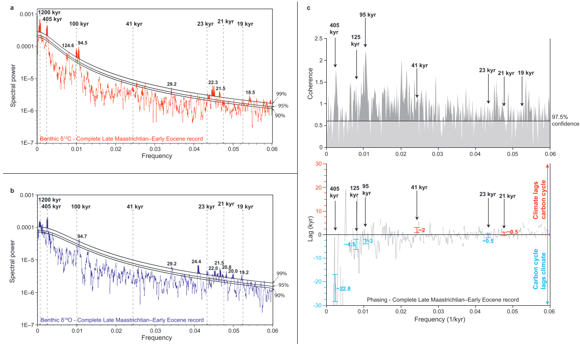
Figure 7. Multitaper Method (MTM) power spectra and phasing for the \delta^{13}\text{C}_{\text{benthic}} and \delta^{18}\text{O}_{\text{benthic}} records from Ocean Drilling Program Site 1262. (a) MTM power spectra for the complete Late Maastrichtian–Early Eocene (67.10–52.35 Ma) \delta^{13}\text{C}_{\text{benthic}} record. The resolution of our \delta^{13}\text{C}_{\text{benthic}} record enables the split eccentricity peaks at ~125 and ~95 kyr to be resolved. (b) MTM power spectra for the complete Late Maastrichtian–Early Eocene (67.10–52.35 Ma) \delta^{18}\text{O}_{\text{benthic}} record. (c) Average coherence and phasing between the Ocean Drilling Program Site 1262 \delta^{13}\text{C}_{\text{benthic}} and \delta^{18}\text{O}_{\text{benthic}} records spanning the Late Maastrichtian–Early Eocene (67.10–52.35 Ma). On the coherence spectra, frequencies above the 97.5% confidence level are considered coherent, for which the phasing between \delta^{13}\text{C}_{\text{benthic}} and \delta^{18}\text{O}_{\text{benthic}} was calculated. Negative values for the phasing (lag) in blue indicate that \delta^{13}\text{C}_{\text{benthic}} lags \delta^{18}\text{O}_{\text{benthic}} (i.e., carbon cycle lags climate), while positive values in red indicate \delta^{18}\text{O}_{\text{benthic}} lags \delta^{13}\text{C}_{\text{benthic}} (i.e., climate lags carbon cycle). Values for the mean lag (in kyr) are indicated, with error at the 97.5% confidence level indicated by vertical bars.
