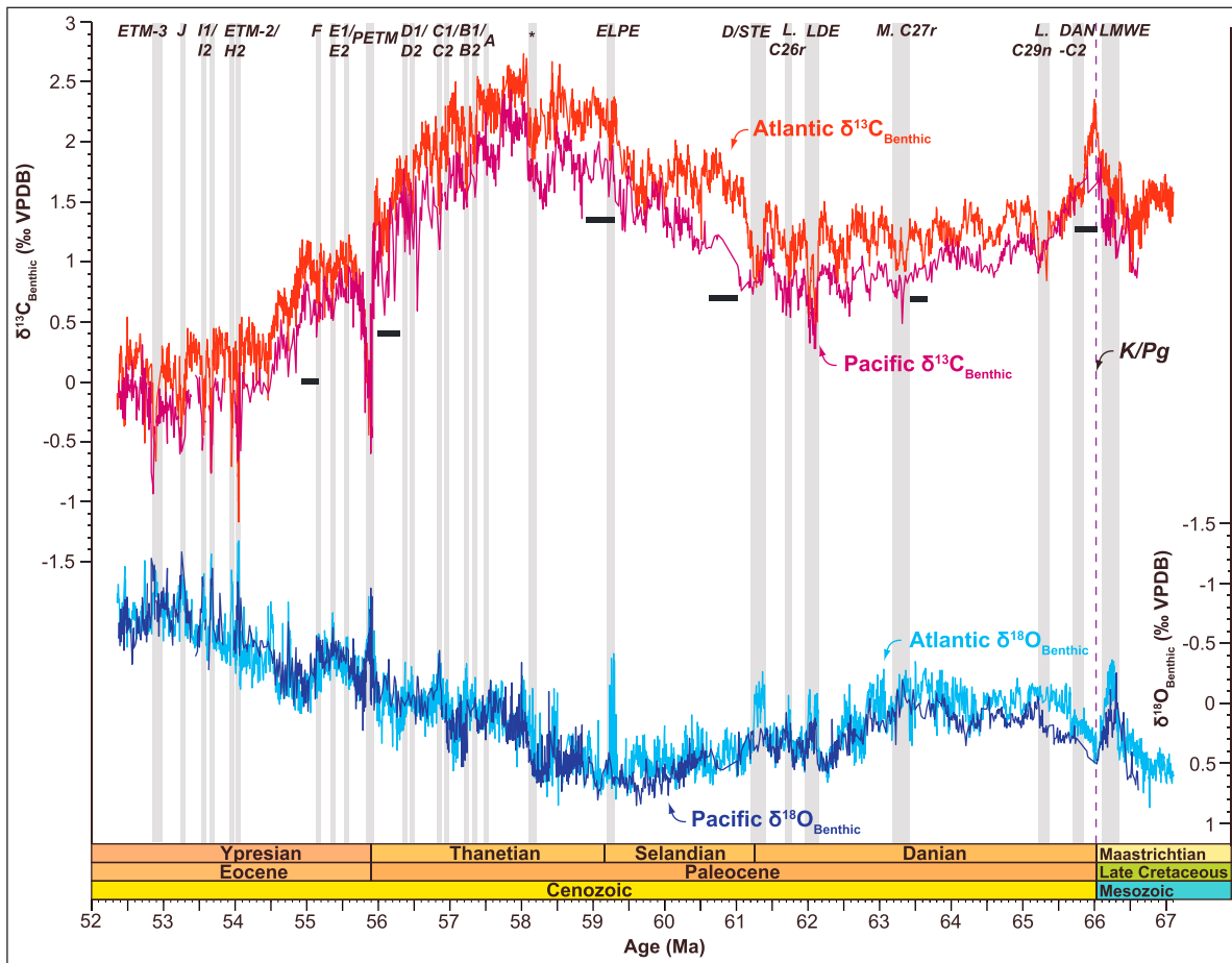
Figure 3. \delta^{13}\text{C}_{\text{benthic}} and \delta^{18}\text{O}_{\text{benthic}} records from ODP Site 1262 (South Atlantic) and ODP Site 1209 (equatorial Pacific; Westerhold et al., 2011, 2018), spanning the Late Maastrichtian–Early Eocene. Both data sets are calibrated to a common orbitally tuned age model correlated to the La2010b orbital solution (Laskar et al., 2011). See Figure 1 for site locations. Condensed intervals at ODP Site 1209 are highlighted beneath the \delta^{13}\text{C}_{\text{benthic}} record by black bars. Hyperthermals and smaller climatic perturbations are illustrated by labeled gray vertical bars. LMWE = Late Maastrichtian warming event; Dan-C2 = Dan-C2 event; L. C29n = Lower Chron 29n event; M. C27r = Middle Chron 27r event; LDE = Latest Danian Event; L. C26r = Lower Chron 26r event; D/STE = Danian/Selandian Transition Event; ELPE = Early Late Paleocene Event; PETM = Paleocene-Eocene Thermal Maximum; ETM-2 = Eocene Thermal Maximum 2; ETM-3 = Eocene Thermal Maximum 3; ODP = Ocean Drilling Program.
