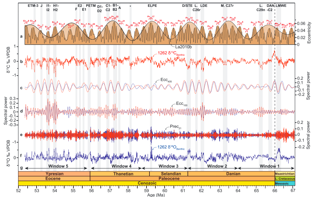
Figure 6. Gaussian filters at the principle Milankovitch frequencies for the benthic stable carbon isotope record ( \delta^{13}\text{C}_{\text{benthic}} , red) and benthic stable oxygen isotope record ( \delta^{18}\text{O}_{\text{benthic}} , blue) from Ocean Drilling Program Site 1262. (a) La2010b orbital solution (Laskar et al., 2011), with long eccentricity (405-kyr) maxima illustrated in dark brown and the filtered \sim 2.4 million-year modulation of eccentricity illustrated in pale brown. The 405-kyr eccentricity maxima are labeled in red following the nomenclature of Husson et al. (2011) for the Maastrichtian, Dinarès-Turell et al. (2014) for the Paleocene, and Westerhold and Röhl (2009) for the Eocene. (b) Detrended \delta^{13}\text{C}_{\text{benthic}} data. (c) Long eccentricity (405-kyr) filter. (d) Short eccentricity (100-kyr) filter. (e) Precession (21-kyr) filter. (f) Detrended \delta^{18}\text{O}_{\text{benthic}} data. (g) Temporal distribution of discrete time windows used in Figures 8 and 10. LMWE = Late Maastrichtian warming event; Dan-C2 = Dan-C2 event; L. C29n = Lower Chron 29n event; M. C27r = Middle Chron 27r event; LDE = Latest Danian Event; L. C26r = Lower Chron 26r event; D/STE = Danian/Selandian Transition Event; ELPE = Early Late Paleocene Event; PETM = Paleocene-Eocene Thermal Maximum; ETM-3 = Eocene Thermal Maximum 3.
