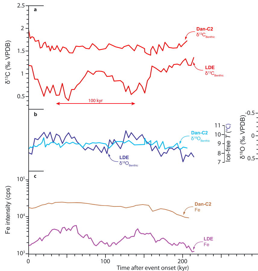
Figure 5. Comparison between the stable isotope and geochemical expressions of the Dan-C2 event and Latest Danian Event (LDE) at Ocean Drilling Program Site 1262, plotted relative to time since onset of the respective events: (a) benthic stable carbon isotope ( \delta^{13}\text{C}_{\text{benthic}} ) records; (b) benthic stable oxygen isotope ( \delta^{18}\text{O}_{\text{benthic}} ) records; (c) Fe intensity records (Westerhold et al., 2008).
