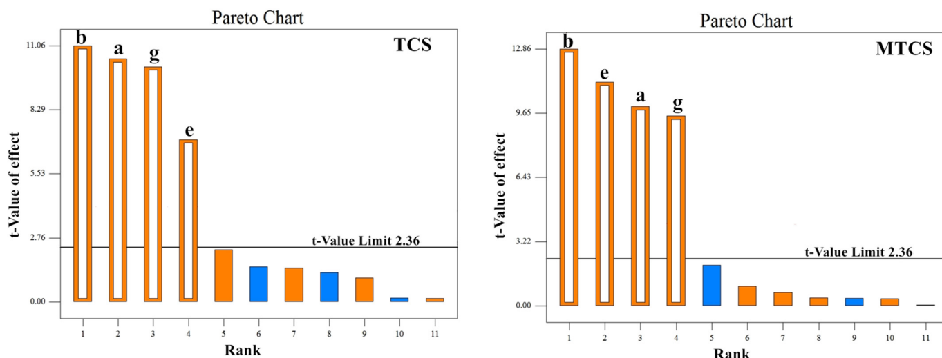
Fig. 3. Standardized Pareto charts ( p < 0.05 ) for main operational factor effects. Note: (A) volume of extractant; (B) volume of disperser; (E) vortex time; (G) centrifugation time.
