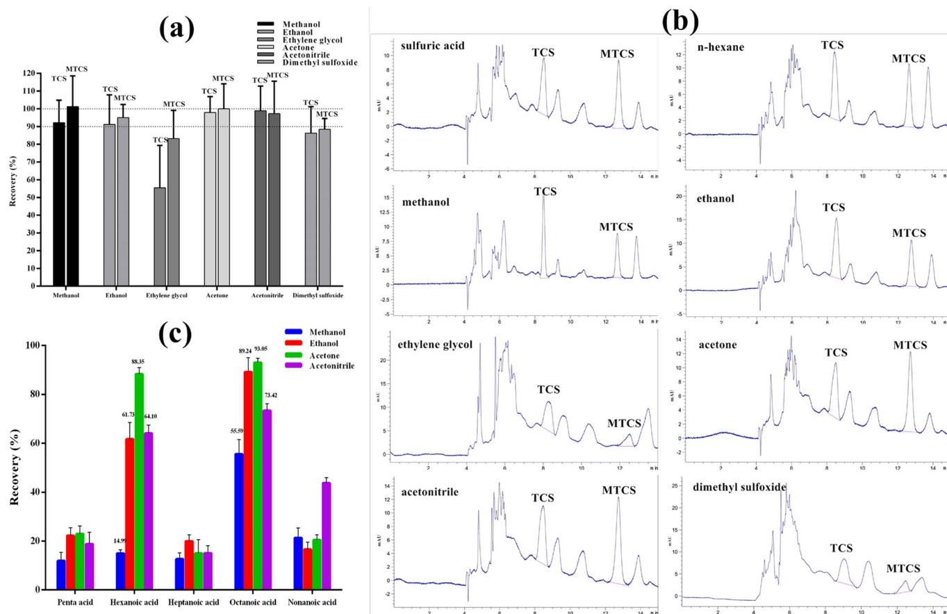
Fig. 2. (a) Enrichment ability of six disperser for TCS and MTCS, (b) Purification ability for marine environmental samples, (c) Extraction recovery of TCS and MTCS with different extractants and dispersers.
