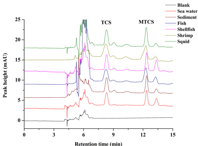
Fig. 5. Chromatogram of TCS and MTCS obtained by the newly developed IDFP-EFA-SFO method under optimized conditions.
