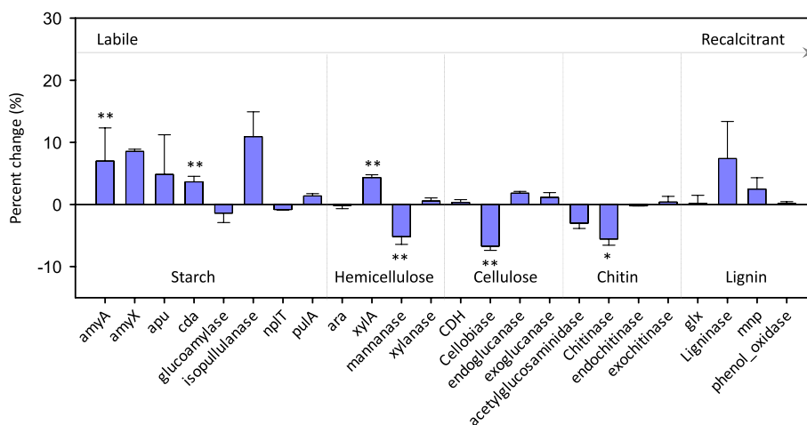
Fig. 2 Changes in C cycling gene abundances. The percent change in the relative abundance of C degradation genes by N deposition is calculated as 100*((mean value in N deposited samples/mean value in control samples) - 1). Mean values and standard deviations are presented. Asterisks indicate significant differences. * P < 0.050 ; ** P < 0.010
