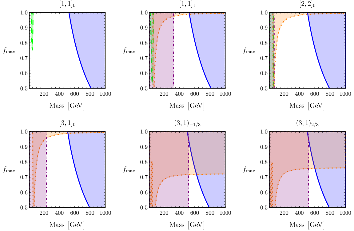
Figure 8. Regions of parameter space for scalar Loryons which are ruled out by one of the constraints described earlier. The orange, dotted region is ruled out by constraints on \kappa_\gamma or \kappa_g ; the blue, solid region is ruled out by unitarity bounds; the green, dashed region is ruled out by constraints on Higgs decay; and the purple, dot-dashed region is ruled out by direct search bounds. All plots assume no mass splitting between the components of the Loryon multiplet, which is a non-trivial assumption for [2, 2]_0 . Note that the bottom middle and right plots are indicated by their SM gauge quantum numbers.
