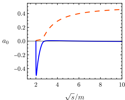
Figure 2. An example of the behavior of the zeroth partial wave coefficients a_0(\sqrt{s}) . The plot is for a neutral singlet scalar Loryon S_0 getting all of its mass m = 525 \text{ GeV} from the Higgs. The two curves correspond to the two eigenvalues of the 2 by 2 scattering matrix (S_0 S_0, hh)^T \rightarrow (S_0 S_0, hh)^T .
