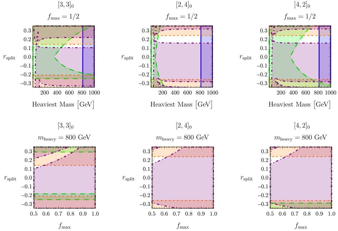
Figure 9. Regions of parameter space for scalar Loryons which are ruled out by one of the constraints described earlier. The orange, dotted region is ruled out by the electroweak precision parameter S ; the purple, dot-dashed region is ruled out by constraints on \kappa_\gamma ; the blue, solid region is ruled out by unitarity bounds; the green, dashed region is ruled out by direct search bounds. The first row has fixed f_{\max} = .5 ; the second row has fixed the heaviest mass eigenvalue at 800 GeV.
