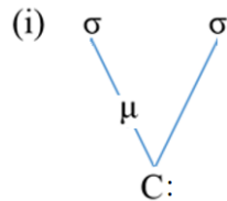
Figure 6.1. Flopped structure of geminates word-medially (adapted from Topintzi 2008: 148)
