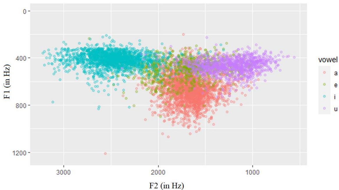
Figure 3.1. Vowel Spaces for Shiwilu
