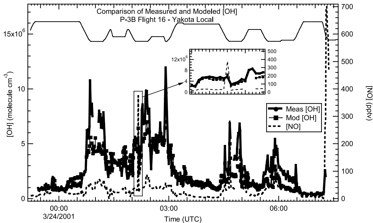
Figure 3. Plot of measured and modeled OH concentrations for a typical flight together with observed [NO], a key species in controlling OH. A relative altitude profile (0.2–5.3 km) is provided for reference. As can be seen much of the high-frequency changes are due to changes in [NO]. The large spikes in NO (due to a ship plume) are large enough to suppress OH by acting as a sink to HO x (see text).
