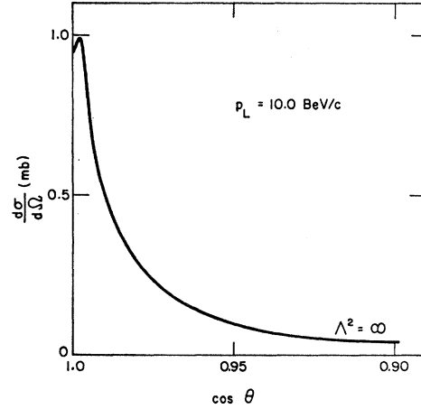
FIG. 7. The cross section at P_L = 10 BeV/c using corrections according to Eq. (5) with \rho^N \eta_{1/2} = 0 and \Lambda^2 = \infty .
